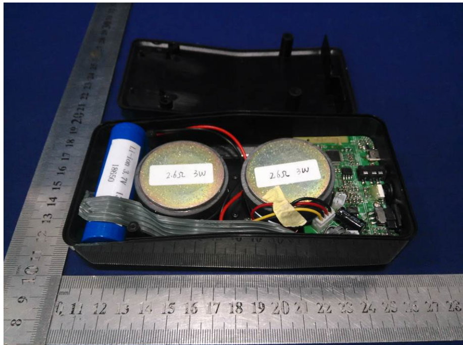
BluetoothAntenna
