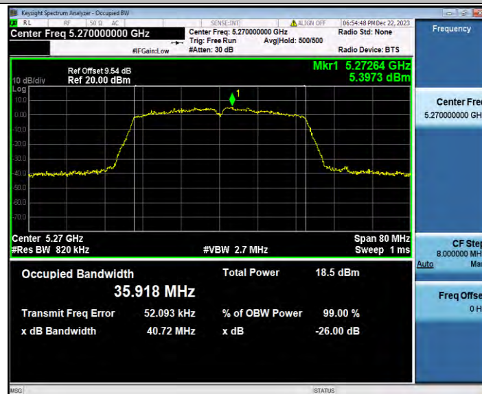
11AC40SISO_Ant0_5270
