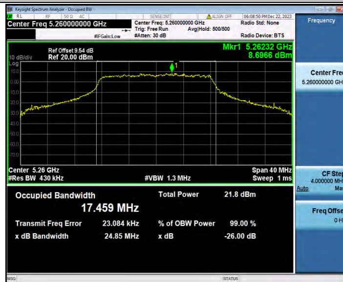
11N20SISO_Ant0_5260
