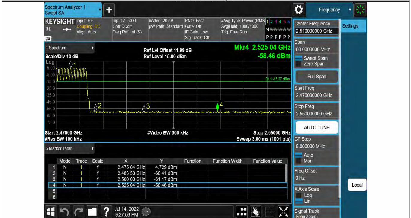
DH5_Ant1_High_Hop_2480
