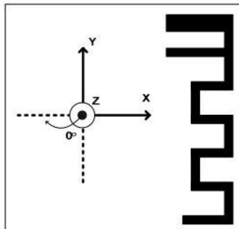
Figure 4: How to Relate the Antenna to the Radiation Patterns
