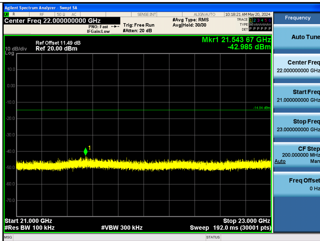
BLE_1M-Ant1-2480-21000~23000-PASS
