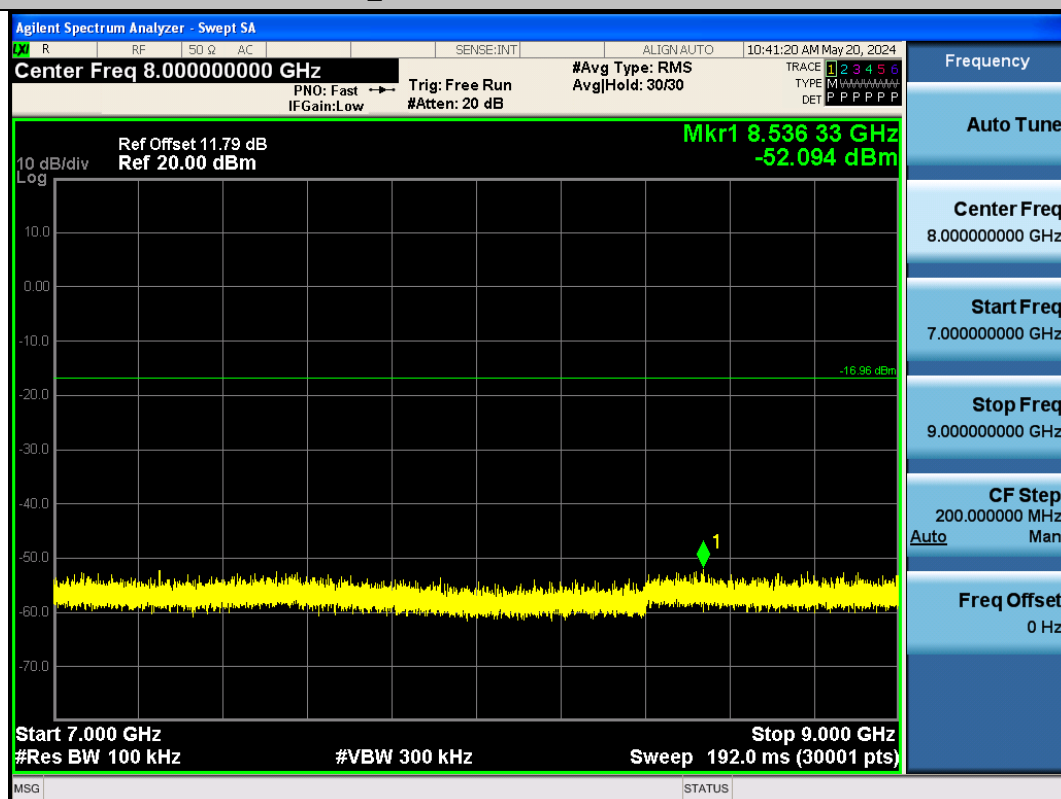
BLE_125K-Ant1-2402-7000~9000-PASS
