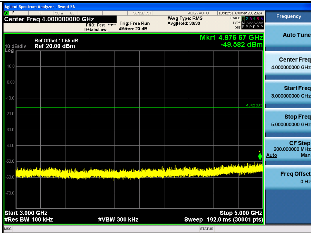
BLE_125K-Ant1-2440-3000~5000-PASS
