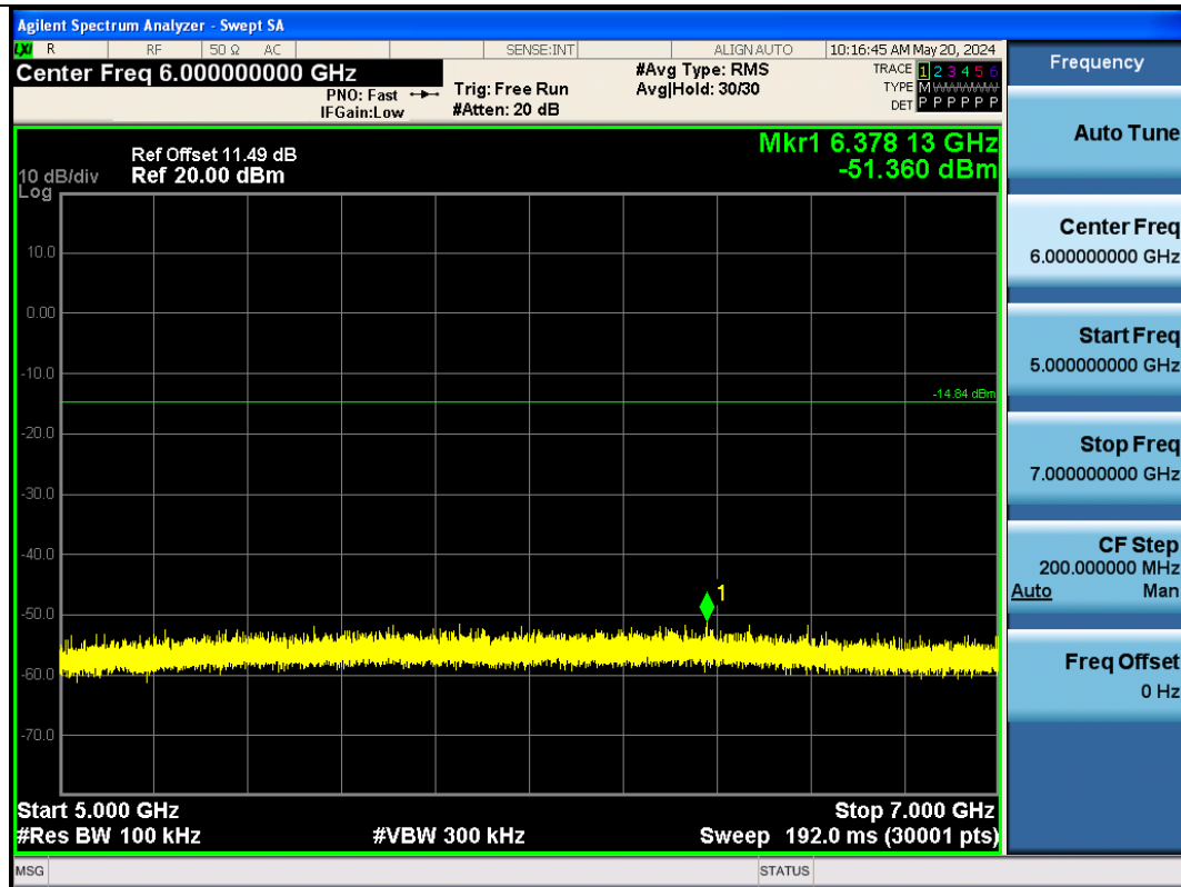
BLE_1M-Ant1-2480-5000~7000-PASS
