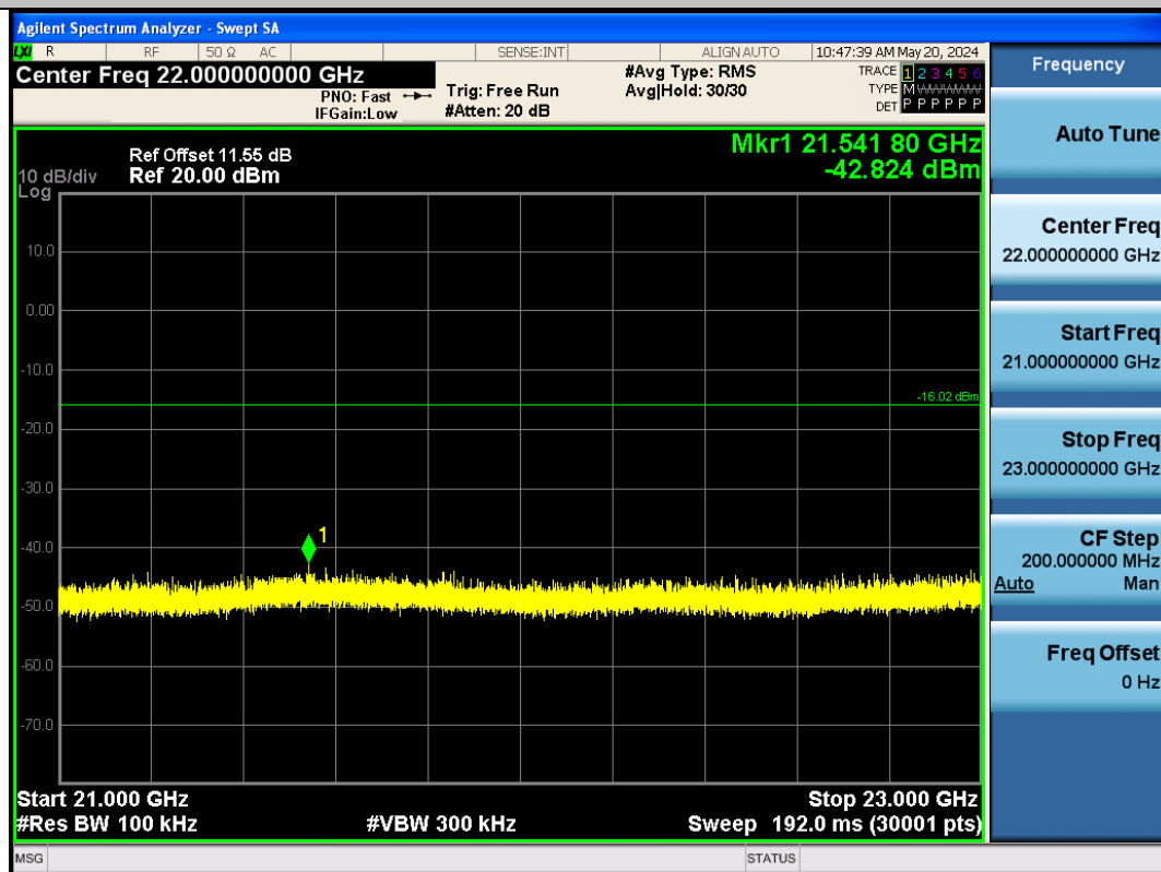
BLE_125K-Ant1-2440-21000~23000-PASS
