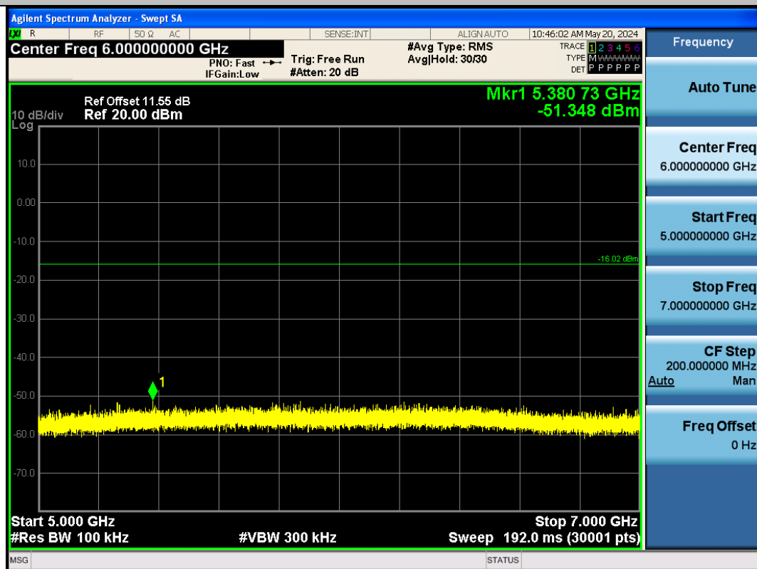
BLE_125K-Ant1-2440-5000~7000-PASS
