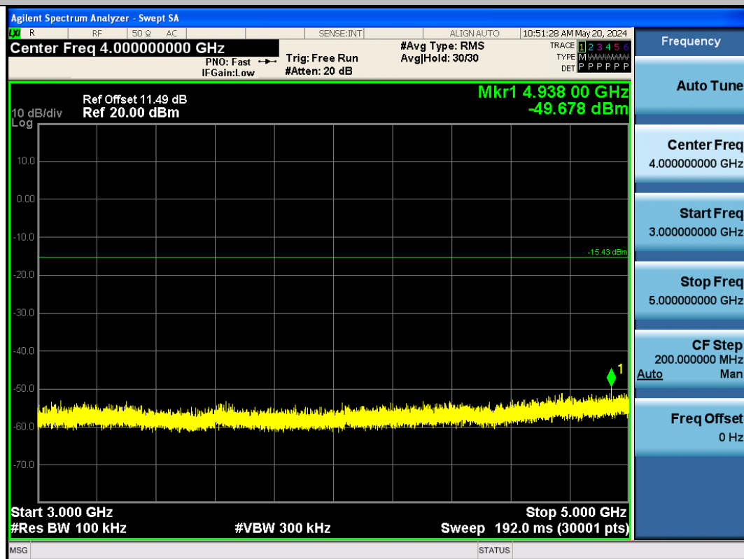
BLE_125K-Ant1-2480-3000-5000-PASS
