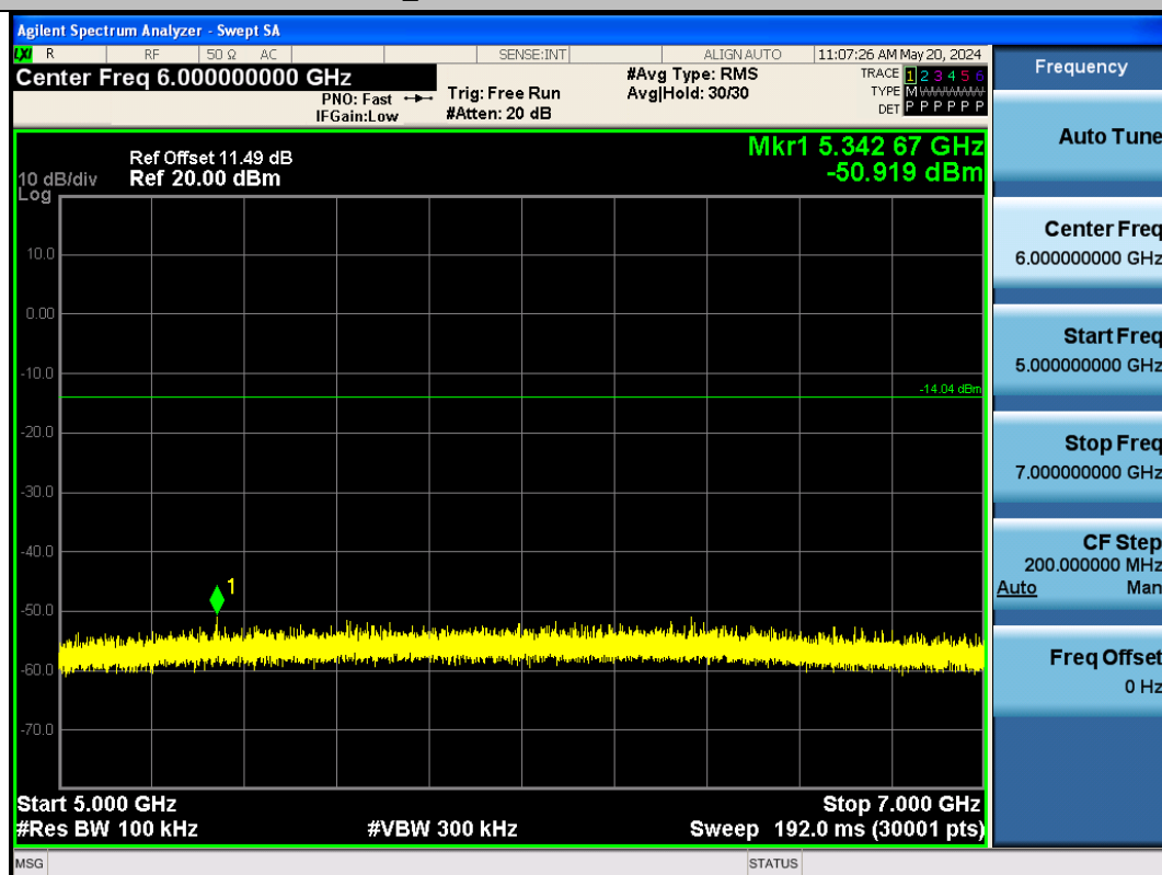
BLE_500K-Ant1-2480-5000~7000-PASS
