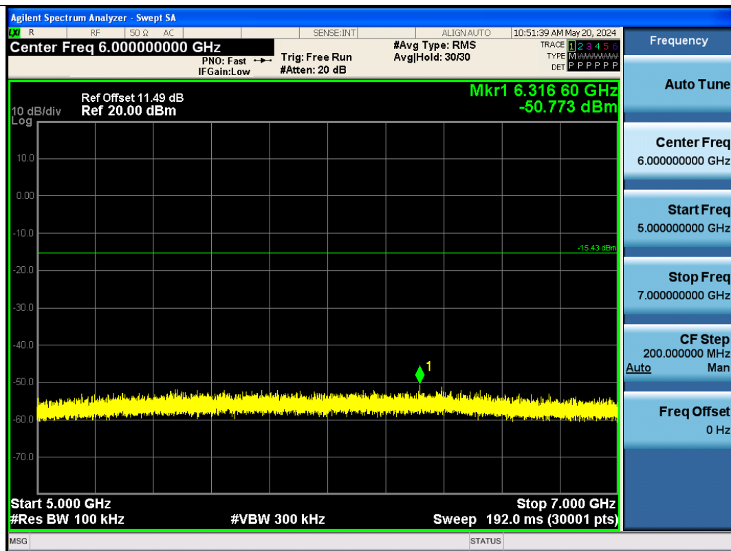
BLE_125K-Ant1-2480-5000~7000-PASS
