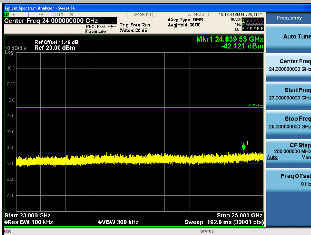
BLE_1M-Ant1-2480-23000~25000-PASS
