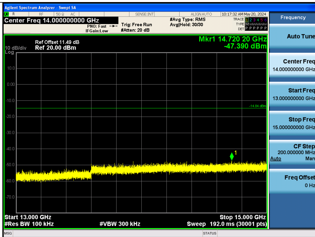
BLE_1M-Ant1-2480-13000~15000-PASS
