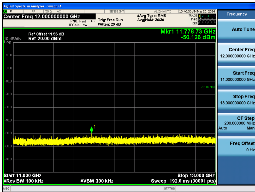
BLE_125K-Ant1-2440-11000~13000-PASS
