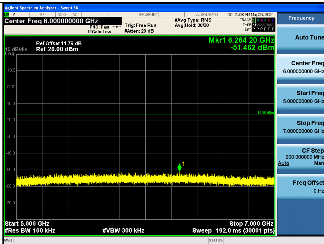
BLE_125K-Ant1-2402-5000~7000-PASS
