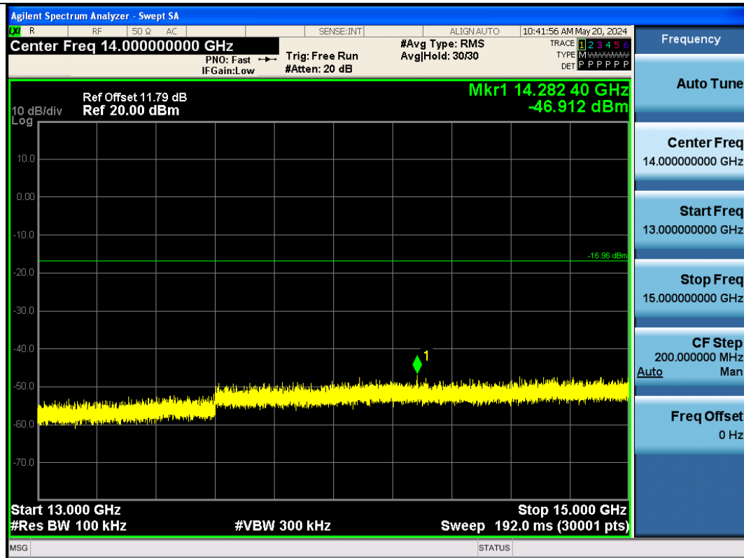
BLE_125K-Ant1-2402-13000~15000-PASS
