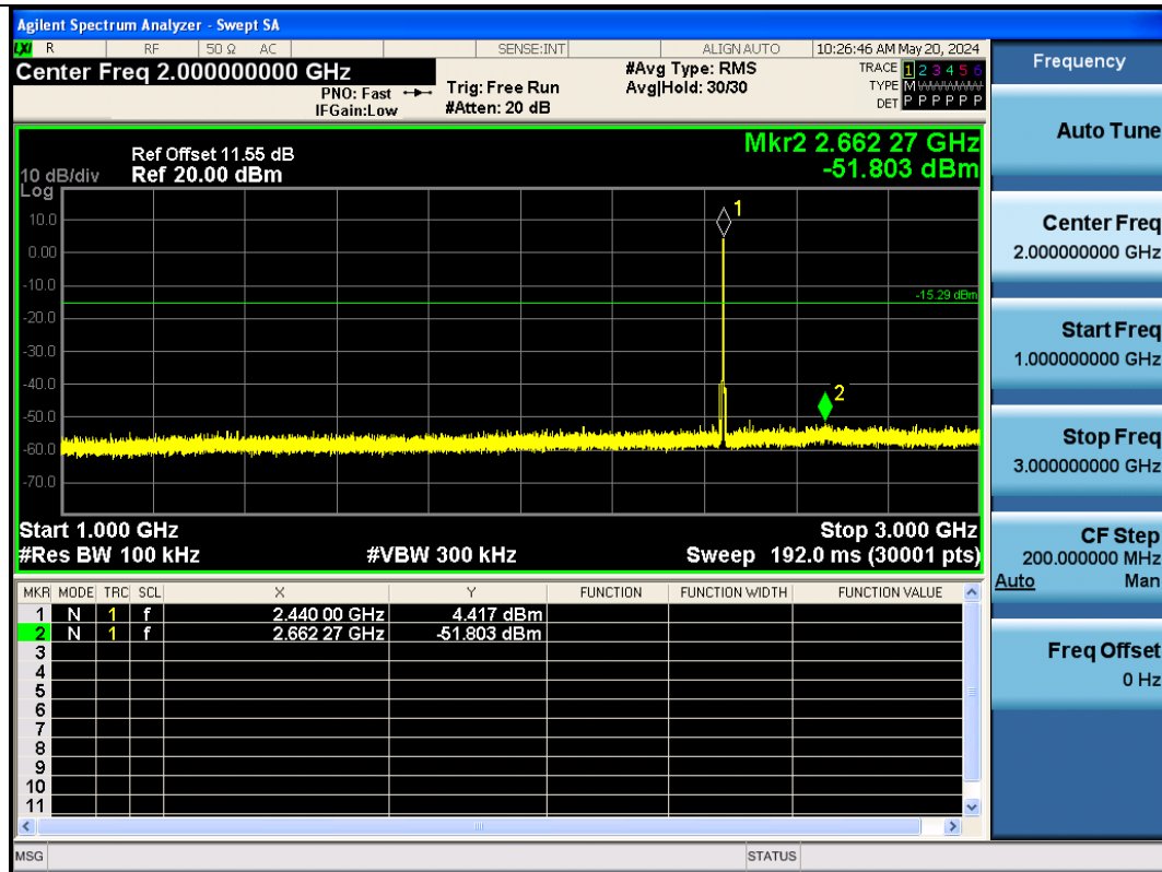
BLE_2M-Ant1-2440-1000~3000-PASS
