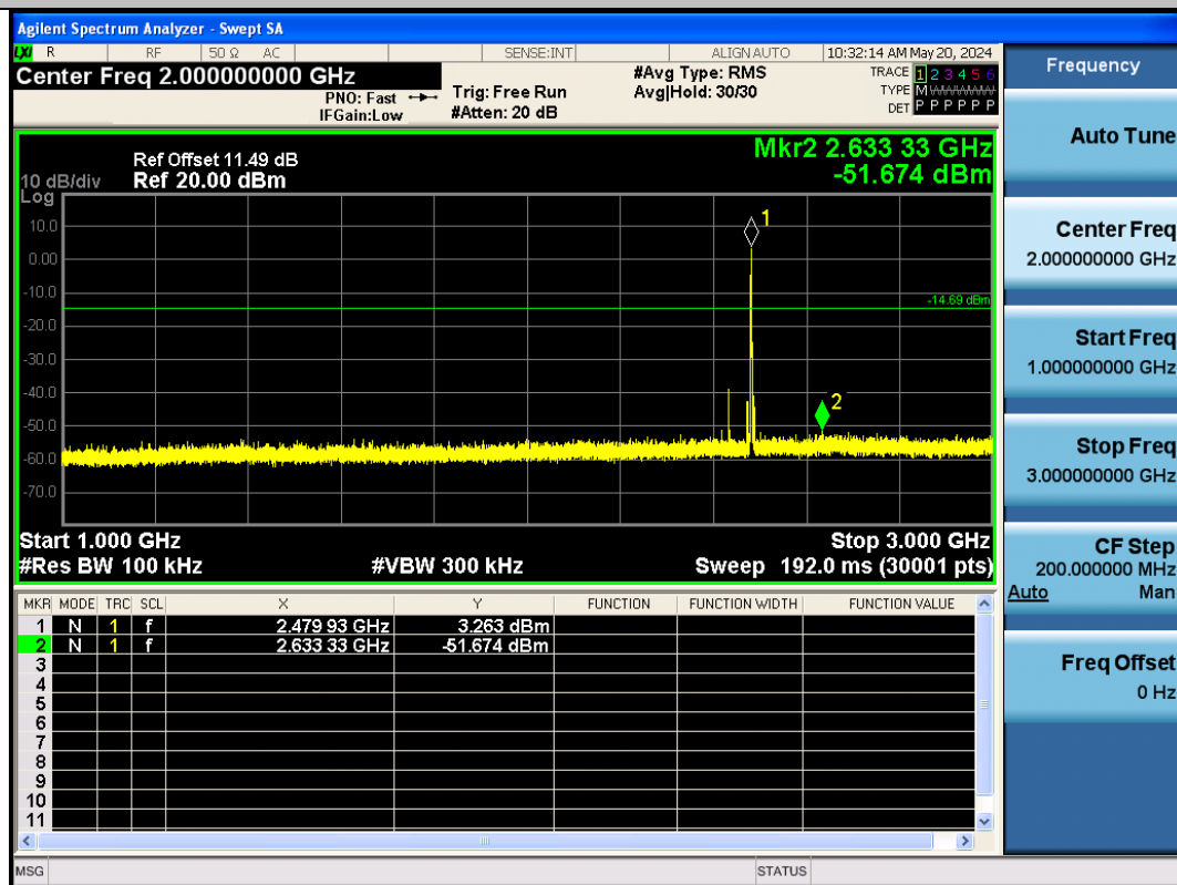
BLE_2M-Ant1-2480-1000~3000-PASS
