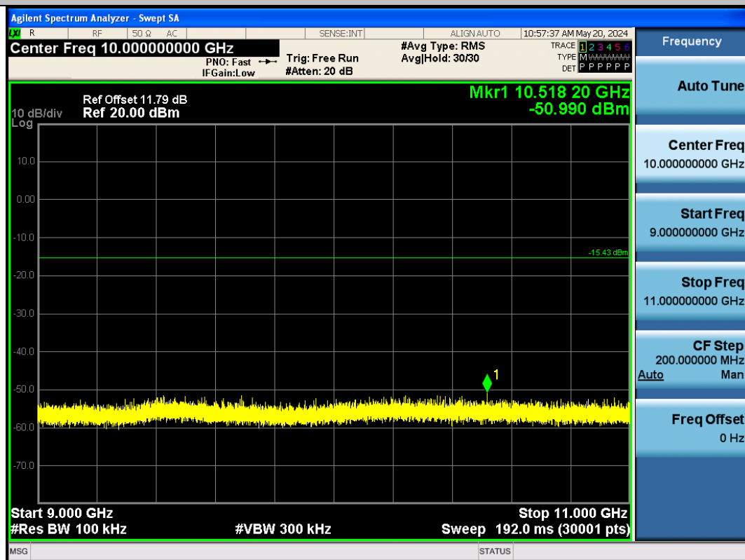
BLE_500K-Ant1-2402-9000-11000-PASS
