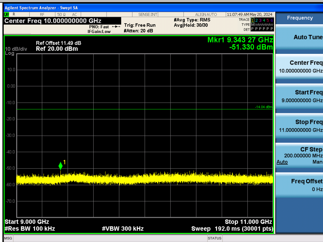
BLE_500K-Ant1-2480-9000-11000-PASS
