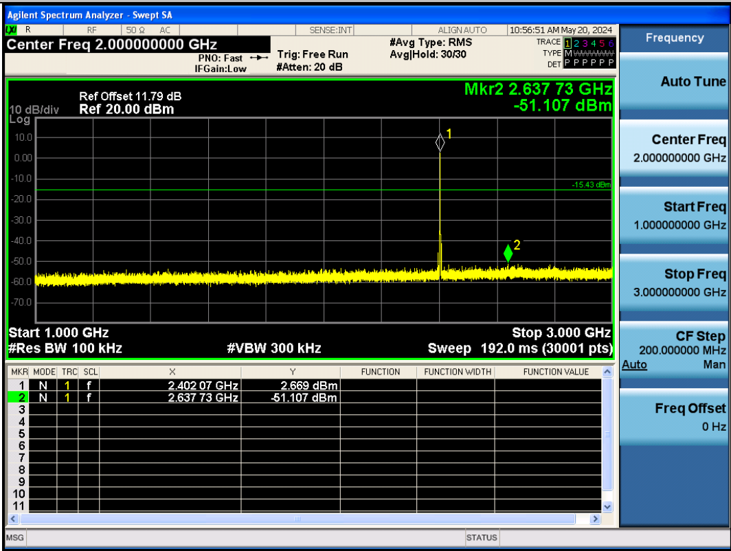
BLE_500K-Ant1-2402-1000~3000-PASS
