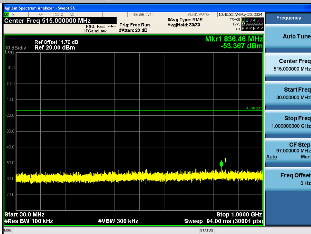
BLE_125K-Ant1-2402-30~1000-PASS
