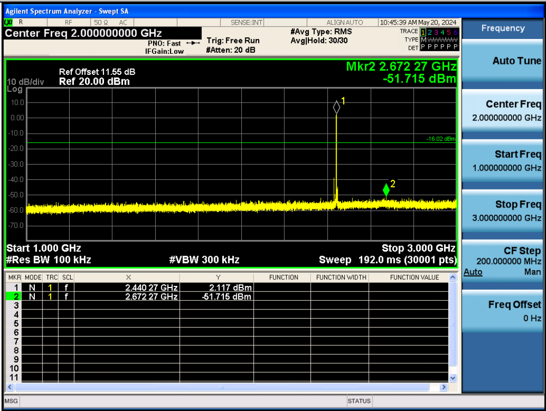
BLE_125K-Ant1-2440-1000~3000-PASS
