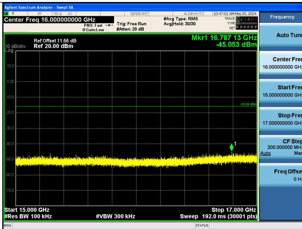
BLE_125K-Ant1-2440-15000~17000-PASS
