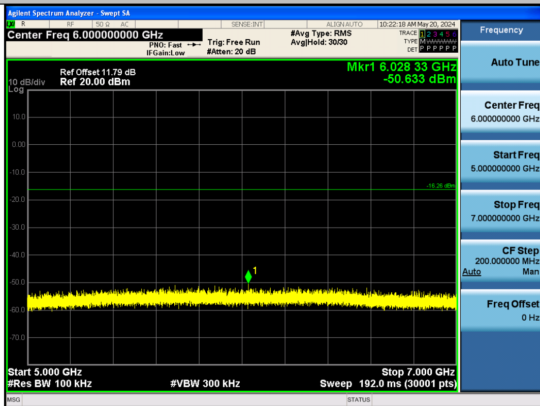
BLE_2M-Ant1-2402-5000~7000-PASS
