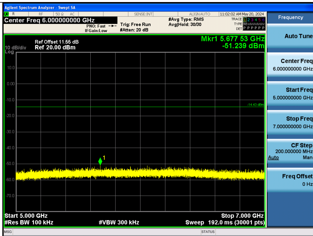
BLE_500K-Ant1-2440-5000~7000-PASS
