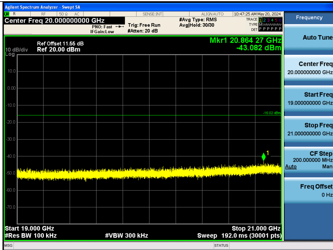
BLE_125K-Ant1-2440-19000~21000-PASS
