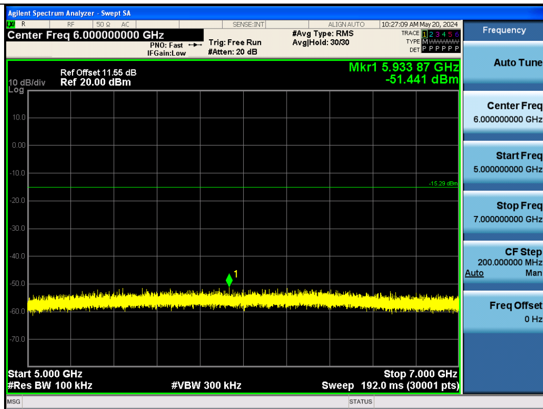
BLE_2M-Ant1-2440-5000~7000-PASS
