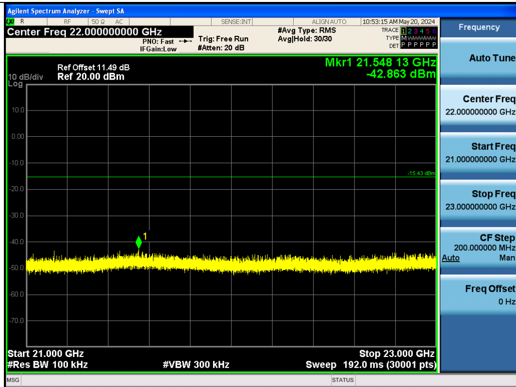
BLE_125K-Ant1-2480-21000~23000-PASS
