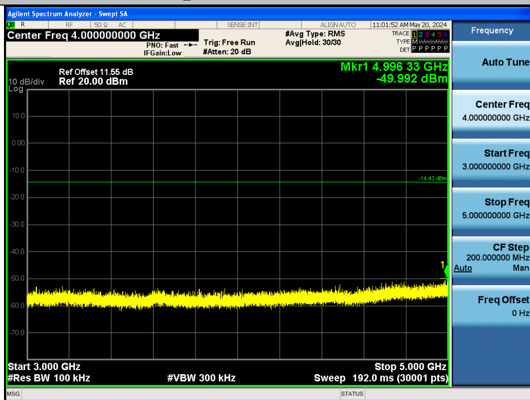
BLE_500K-Ant1-2440-3000-5000-PASS
