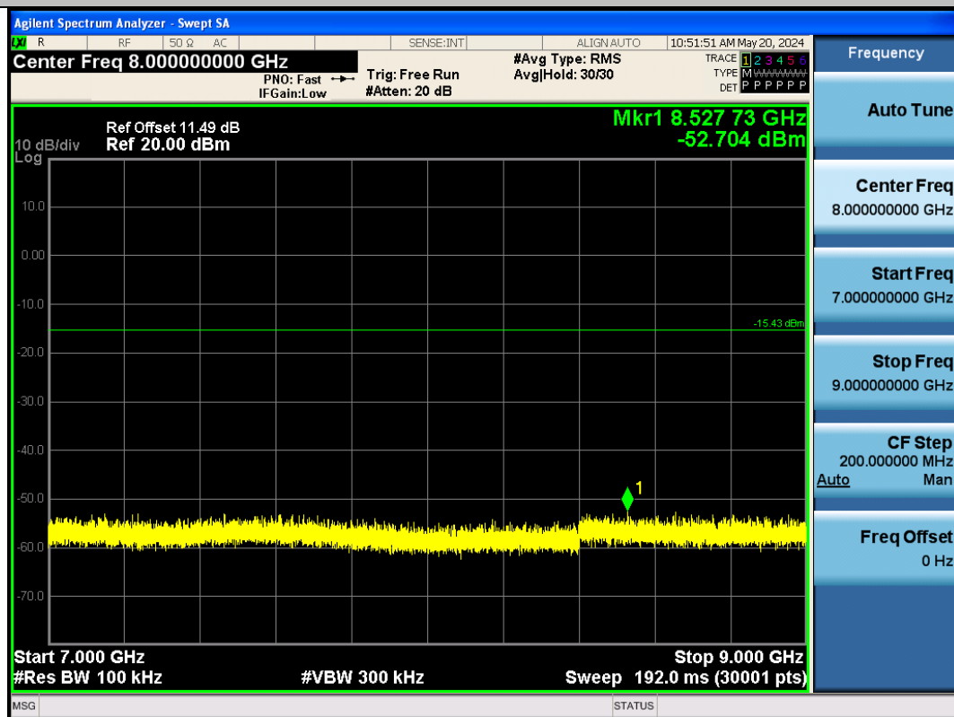
BLE_125K-Ant1-2480-7000~9000-PASS
