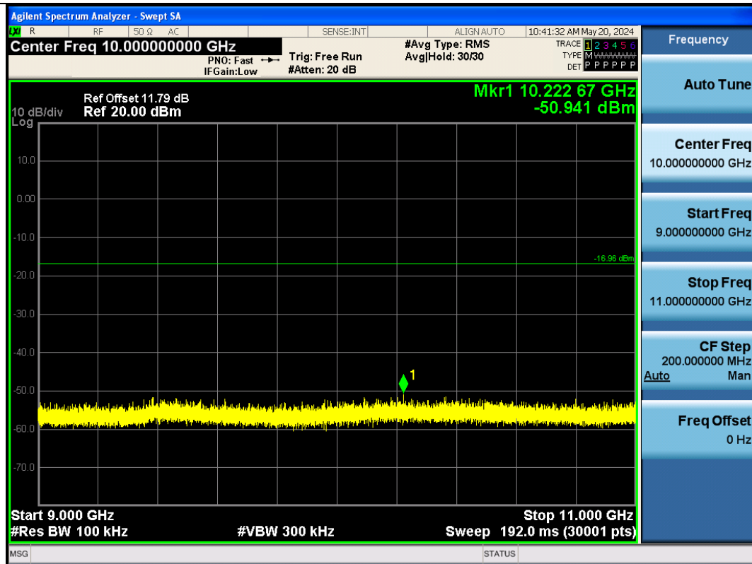
BLE_125K-Ant1-2402-9000~11000-PASS
