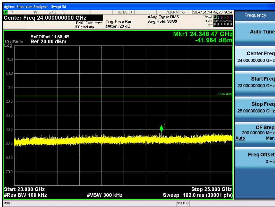
BLE_125K-Ant1-2440-23000~25000-PASS
