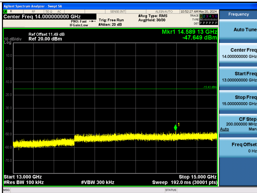
BLE_125K-Ant1-2480-13000~15000-PASS
