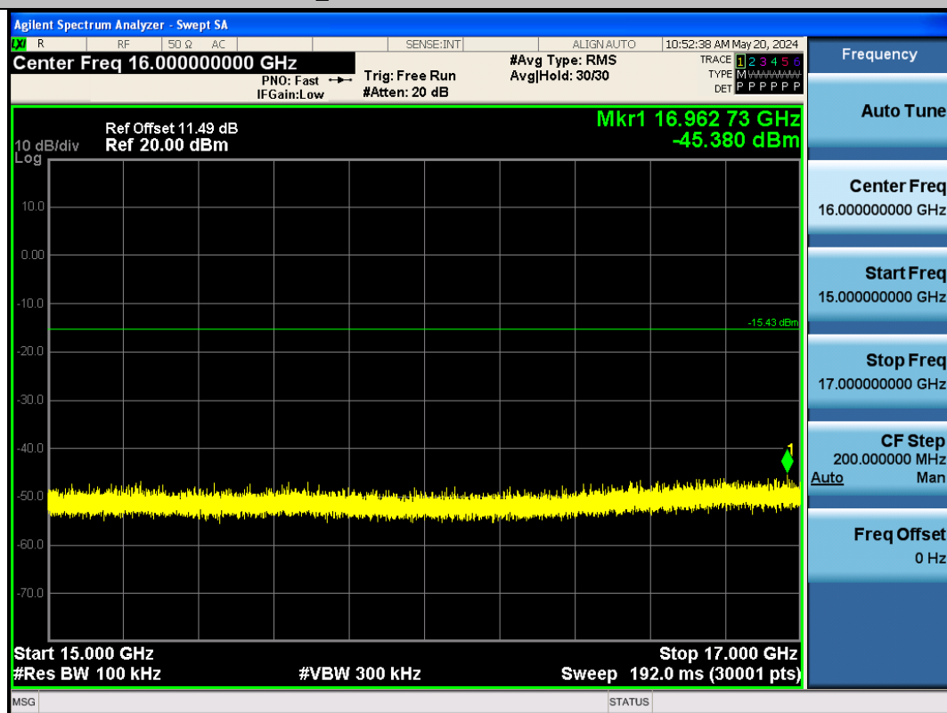
BLE_125K-Ant1-2480-15000~17000-PASS
