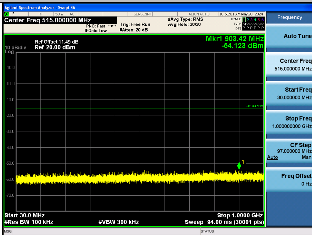
BLE_125K-Ant1-2480-30~1000-PASS
