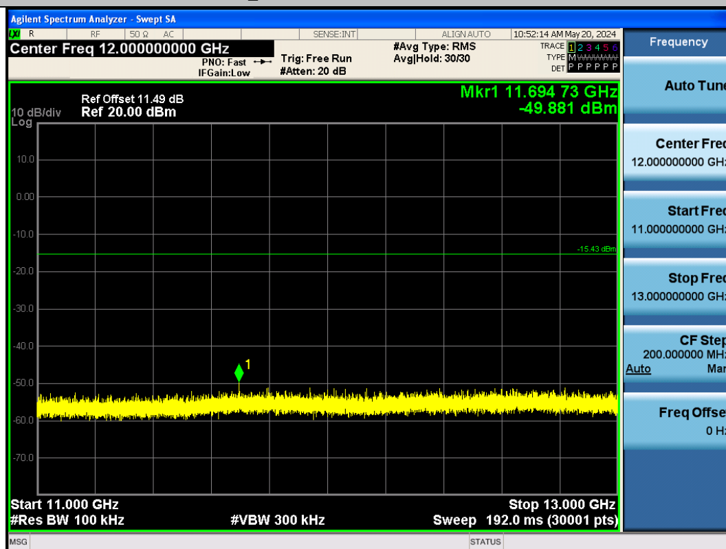
BLE_125K-Ant1-2480-11000~13000-PASS
