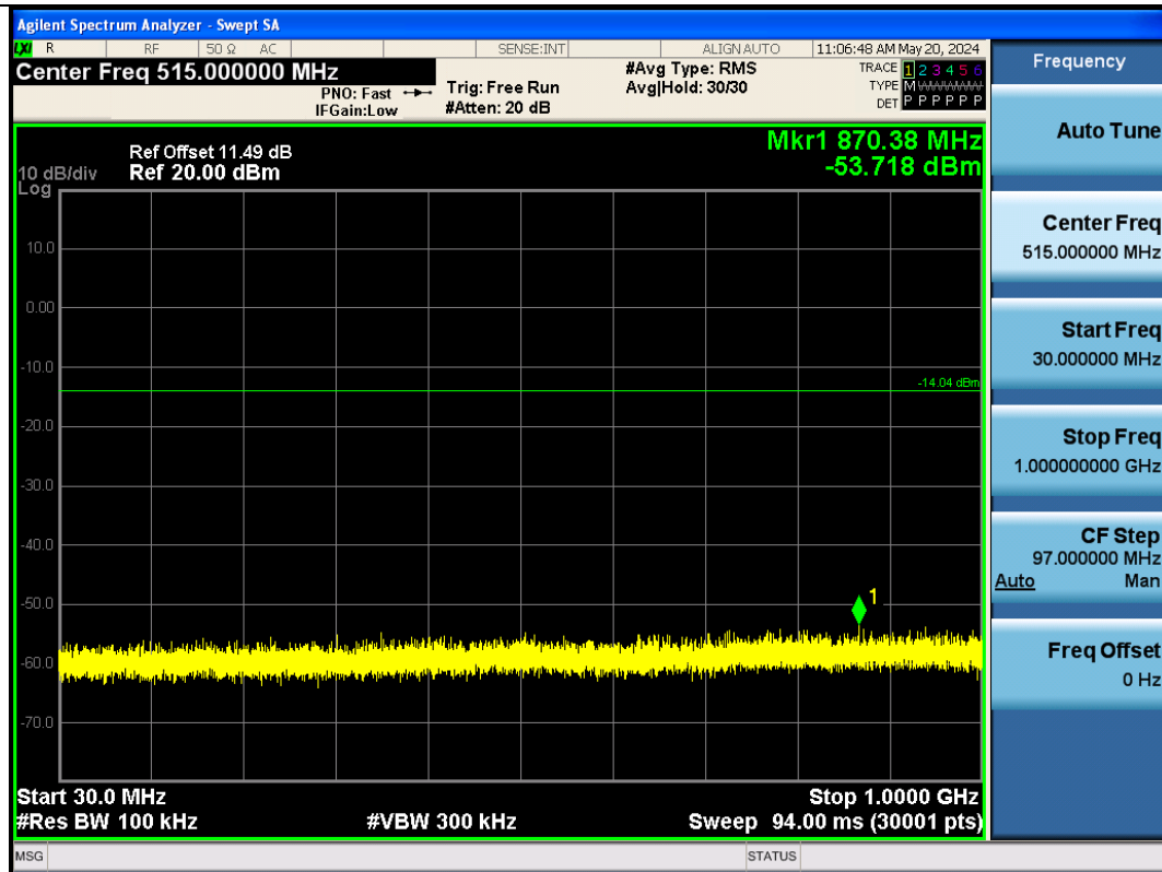
BLE_500K-Ant1-2480-30~1000-PASS
