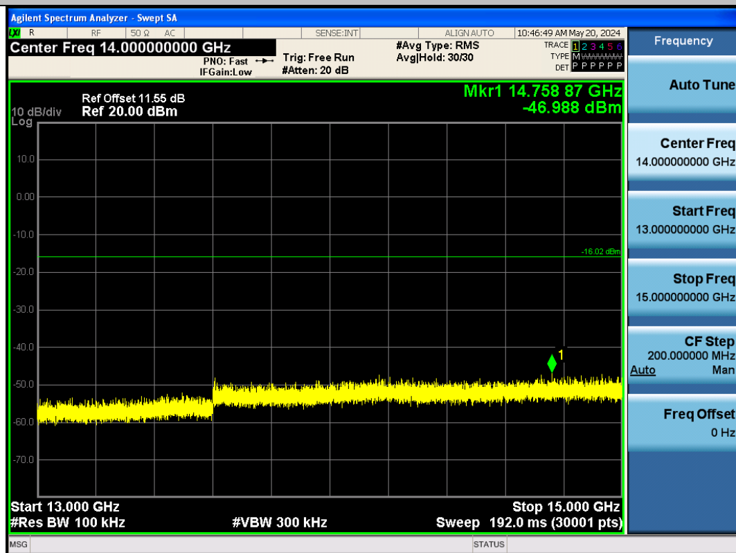
BLE_125K-Ant1-2440-13000~15000-PASS
