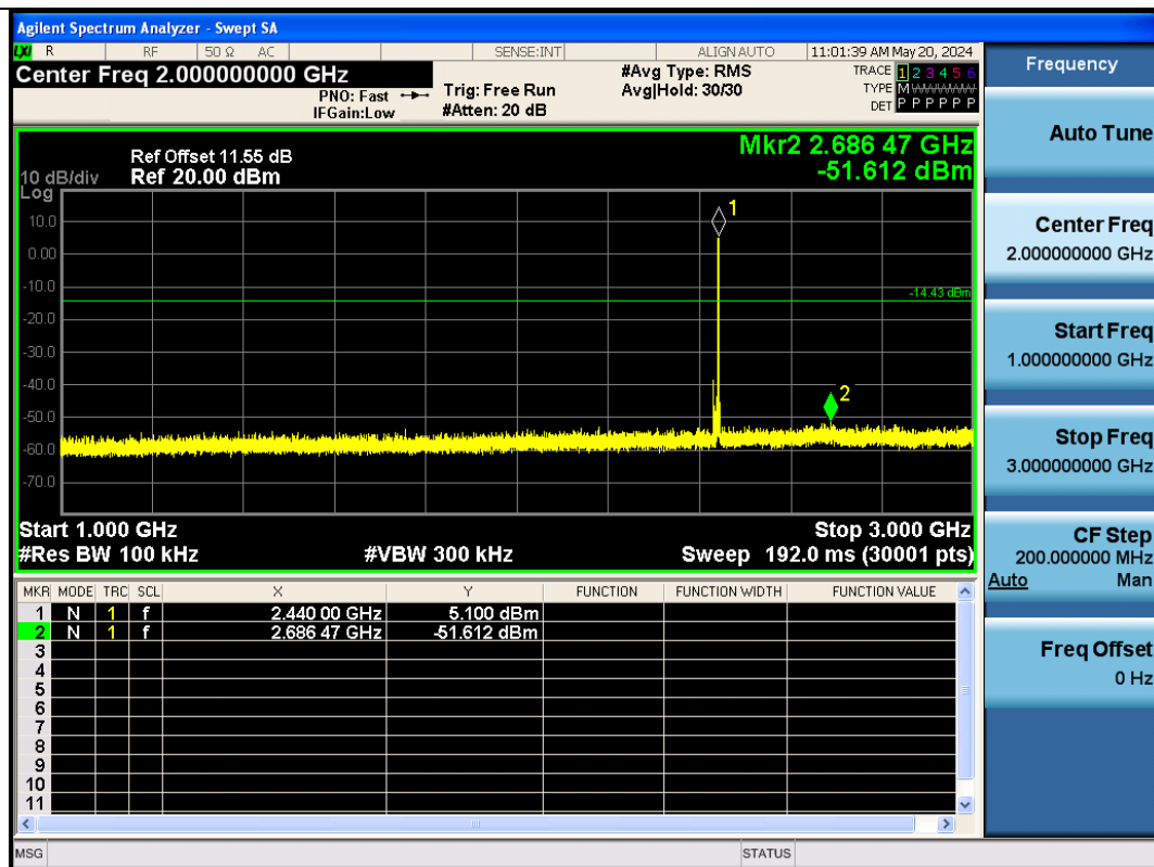
BLE_500K-Ant1-2440-1000-3000-PASS
