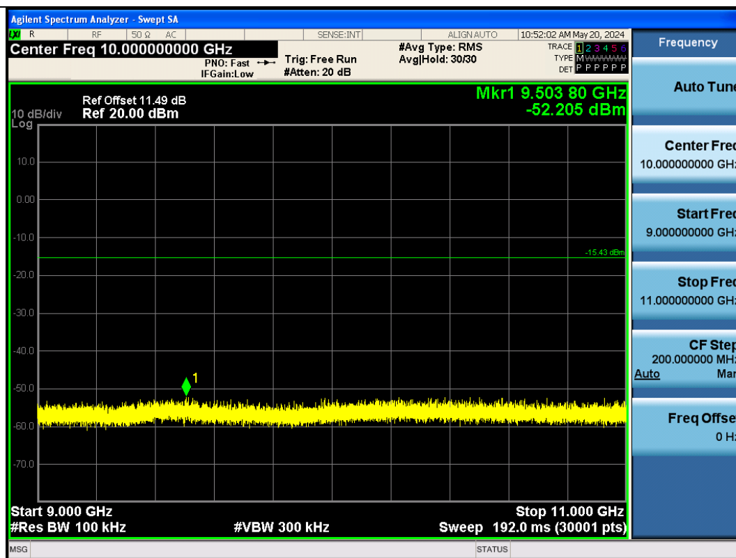
BLE_125K-Ant1-2480-9000~11000-PASS
