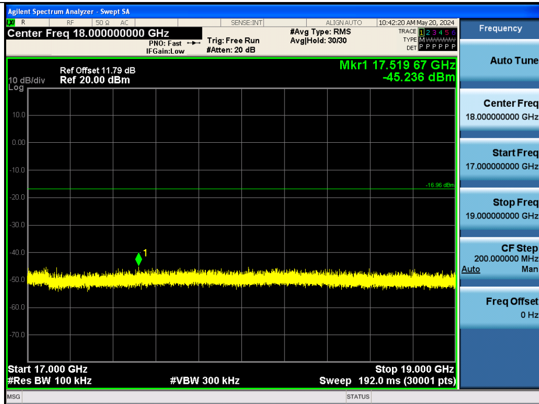
BLE_125K-Ant1-2402-17000~19000-PASS
