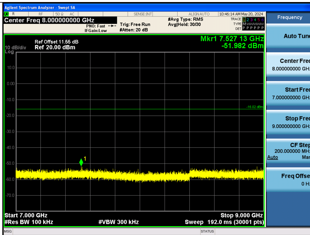
BLE_125K-Ant1-2440-7000-9000-PASS
