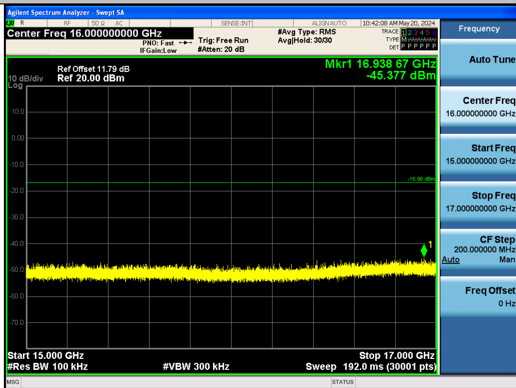
BLE_125K-Ant1-2402-15000~17000-PASS
