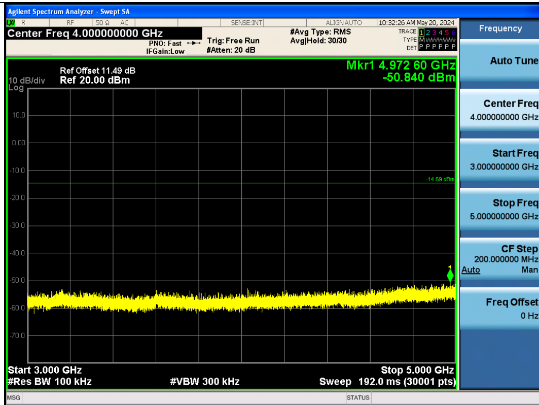
BLE_2M-Ant1-2480-3000~5000-PASS
