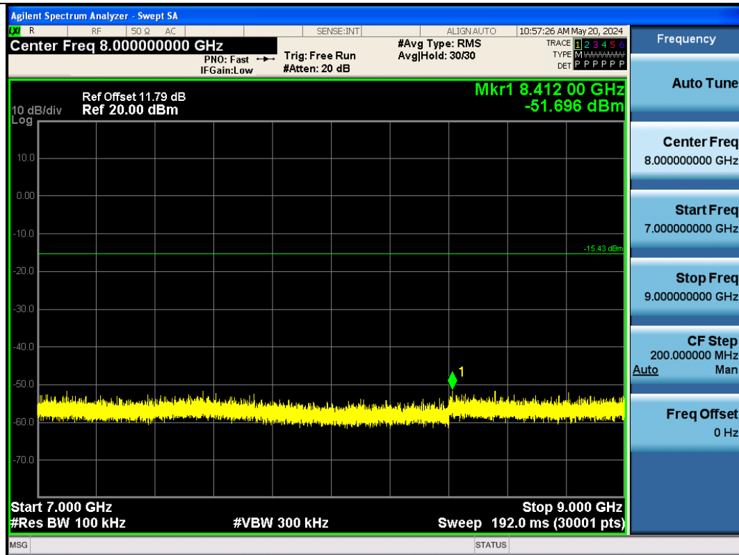
BLE_500K-Ant1-2402-7000-9000-PASS
