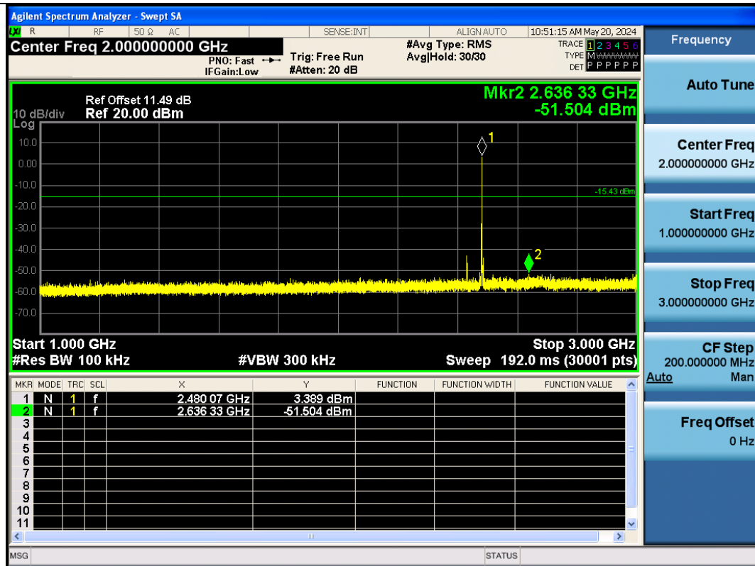
BLE_125K-Ant1-2480-1000-3000-PASS
