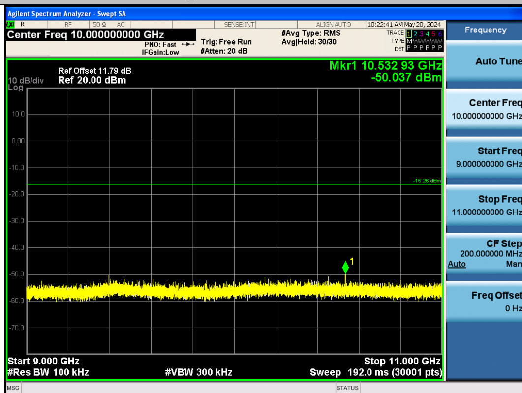
BLE_2M-Ant1-2402-9000~11000-PASS
