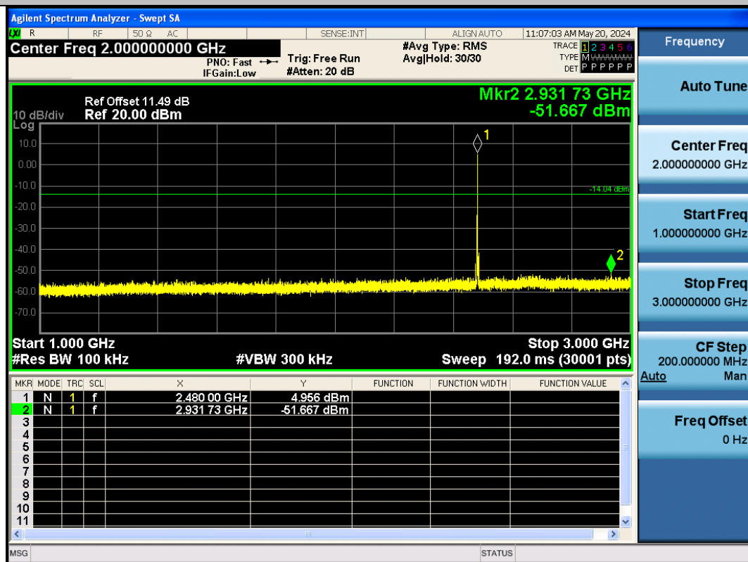
BLE_500K-Ant1-2480-1000~3000-PASS
