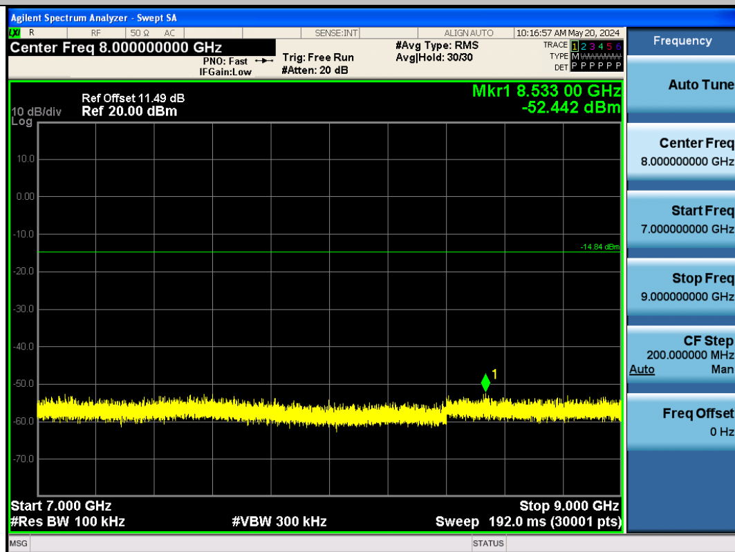
BLE_1M-Ant1-2480-7000~9000-PASS
