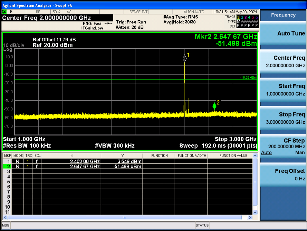
BLE_2M-Ant1-2402-1000~3000-PASS
