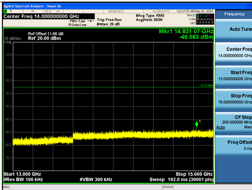
BLE_2M-Ant1-2440-13000~15000-PASS
