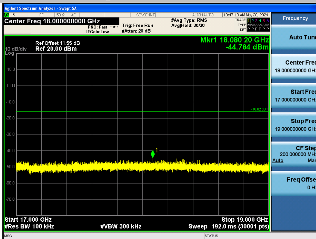
BLE_125K-Ant1-2440-17000~19000-PASS
