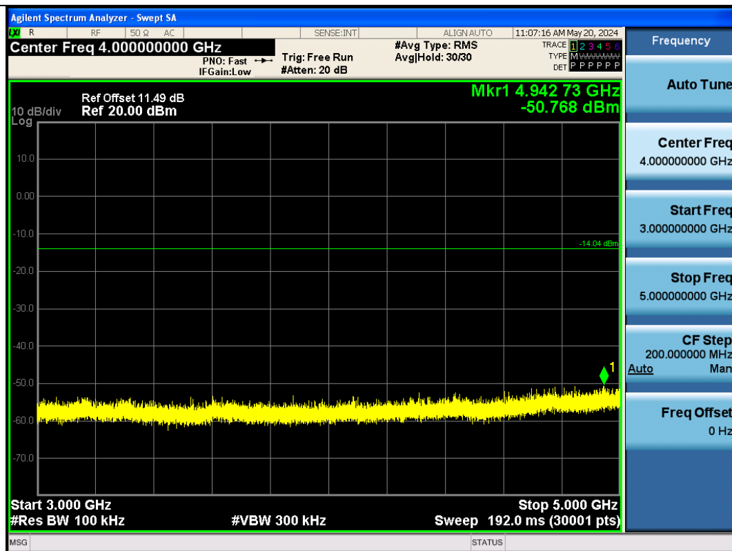
BLE_500K-Ant1-2480-3000~5000-PASS
