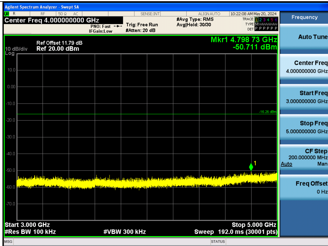
BLE_2M-Ant1-2402-3000~5000-PASS
