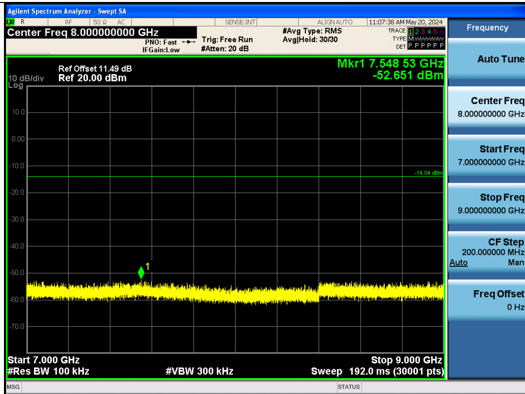
BLE_500K-Ant1-2480-7000-9000-PASS
