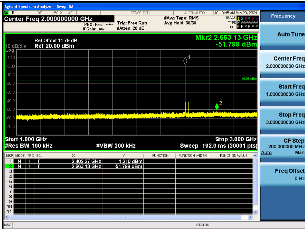
BLE_125K-Ant1-2402-1000~3000-PASS
