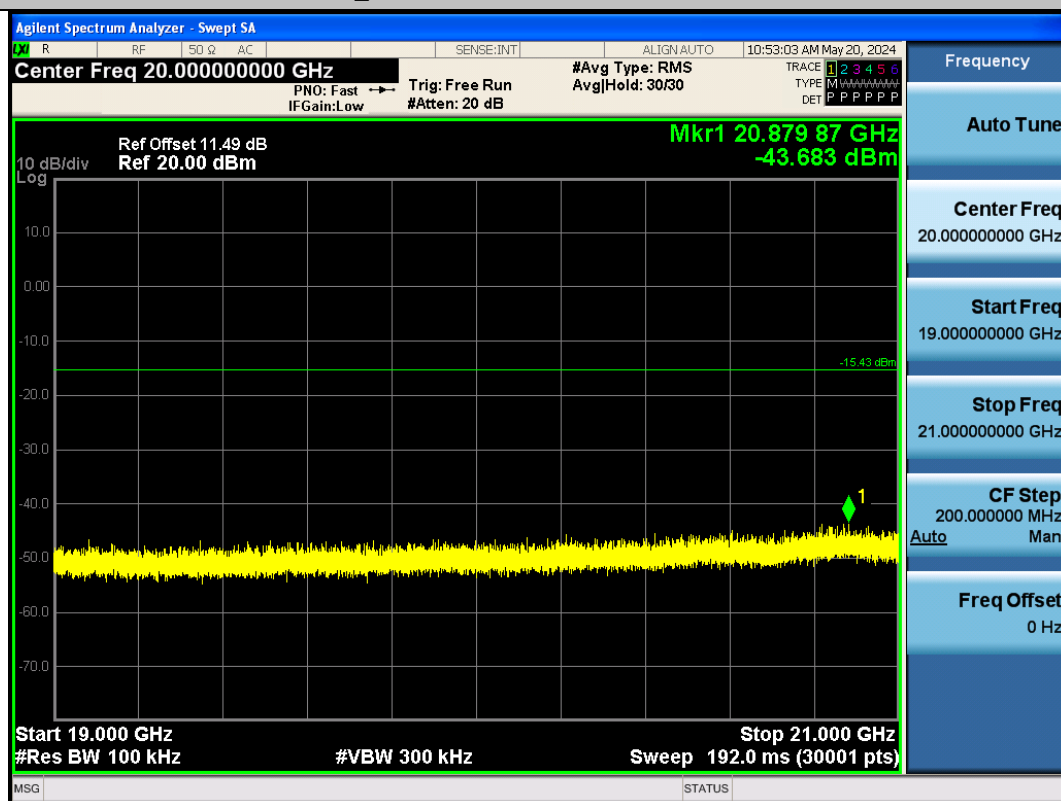
BLE_125K-Ant1-2480-19000~21000-PASS
