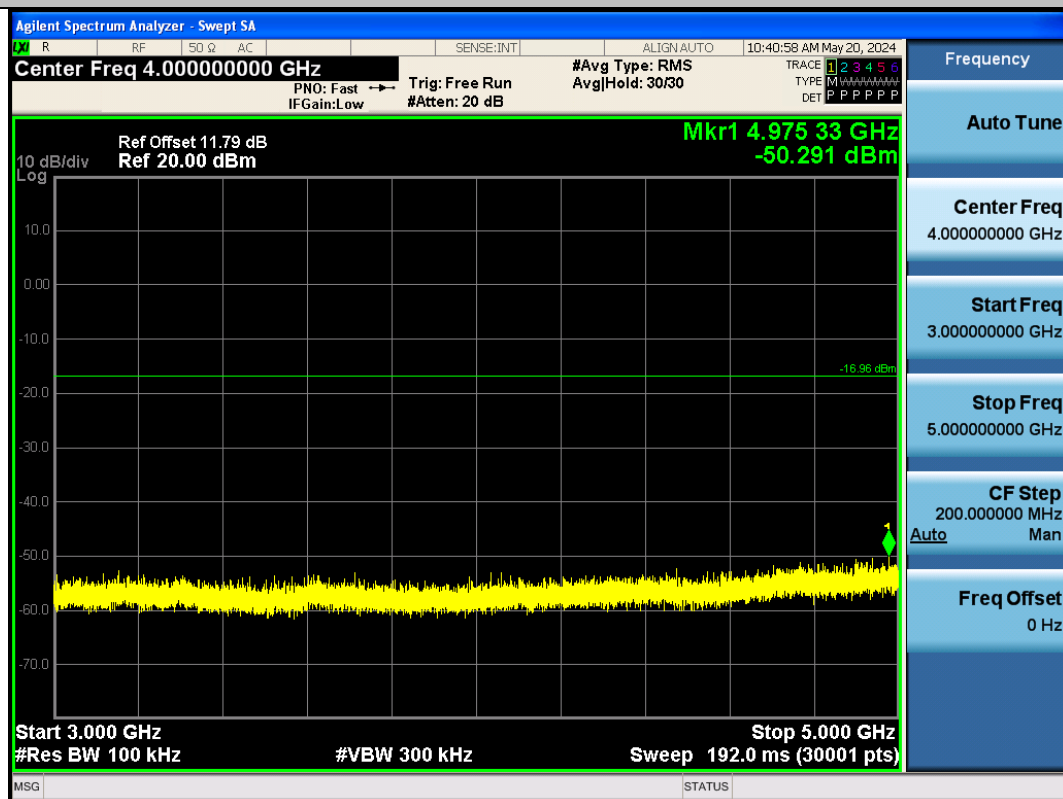
BLE_125K-Ant1-2402-3000~5000-PASS
