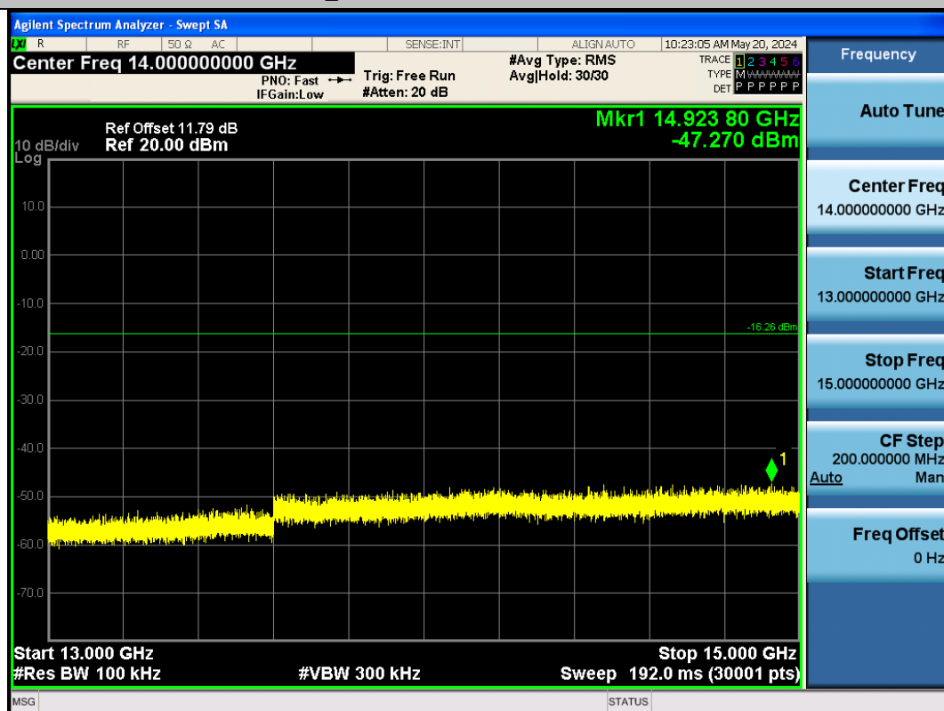
BLE_2M-Ant1-2402-13000~15000-PASS
