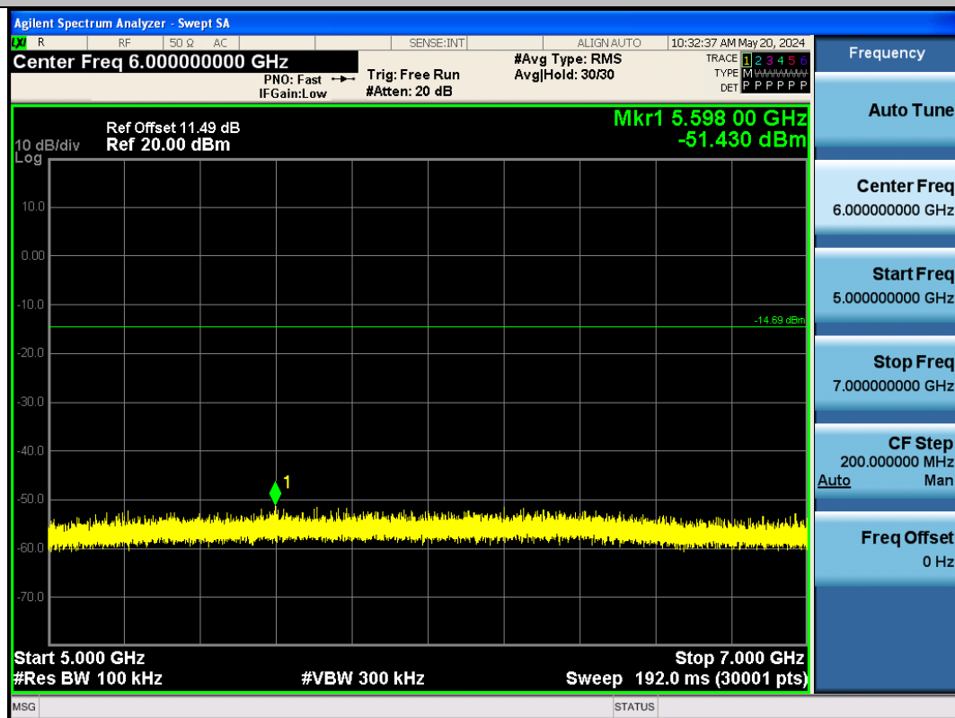
BLE_2M-Ant1-2480-5000~7000-PASS
