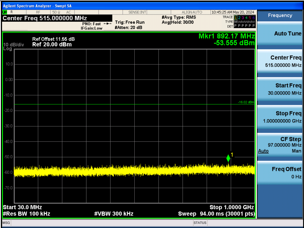
BLE_125K-Ant1-2440-30~1000-PASS
