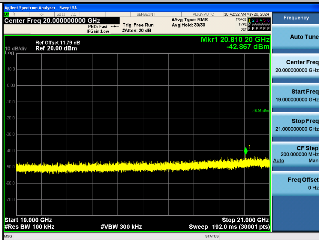
BLE_125K-Ant1-2402-19000~21000-PASS
