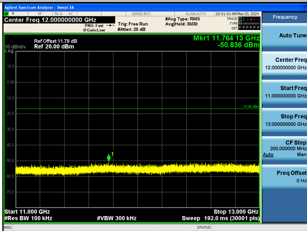
BLE_125K-Ant1-2402-11000~13000-PASS
