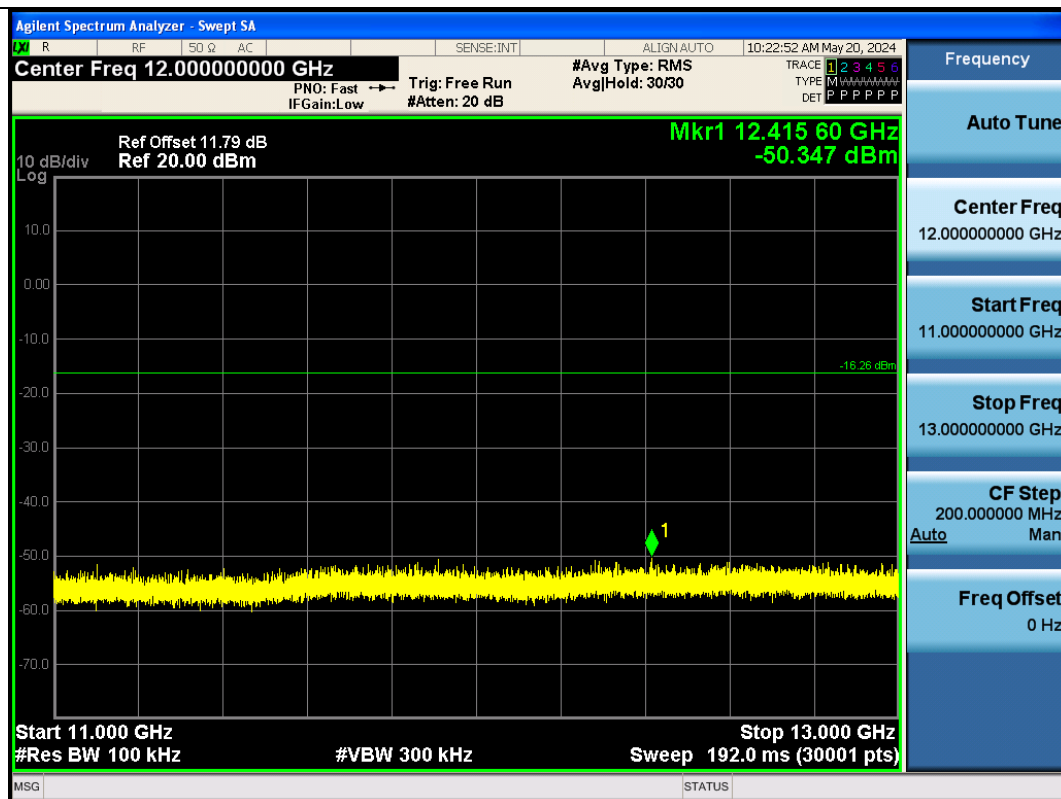
BLE_2M-Ant1-2402-11000~13000-PASS
