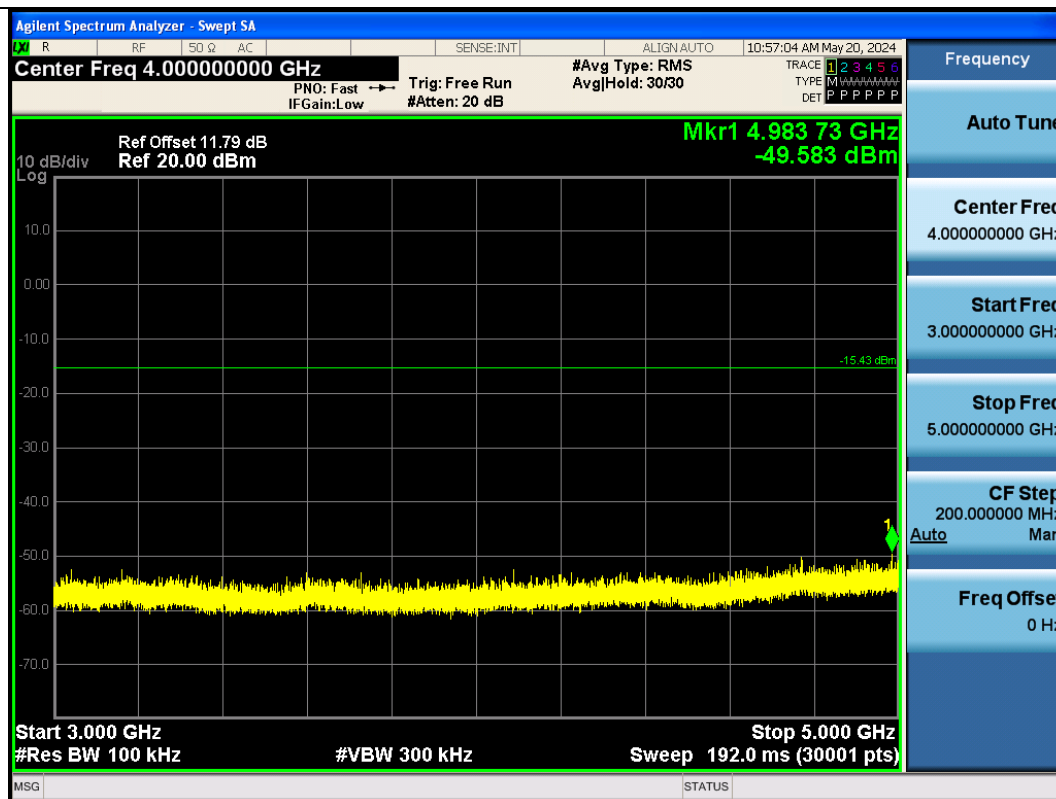
BLE_500K-Ant1-2402-3000~5000-PASS
