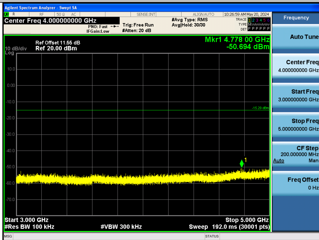
BLE_2M-Ant1-2440-3000~5000-PASS
