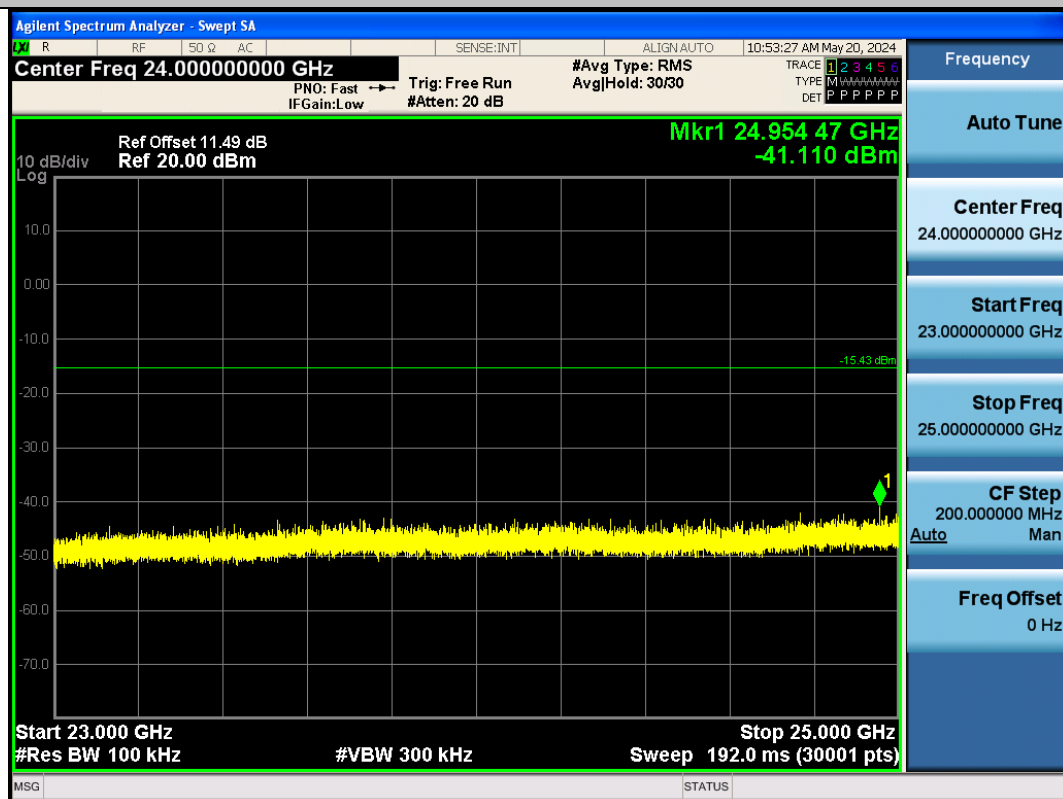
BLE_125K-Ant1-2480-23000~25000-PASS
