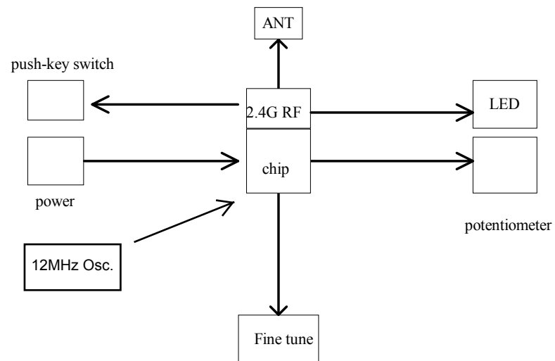
44647TXV2 block diagram
