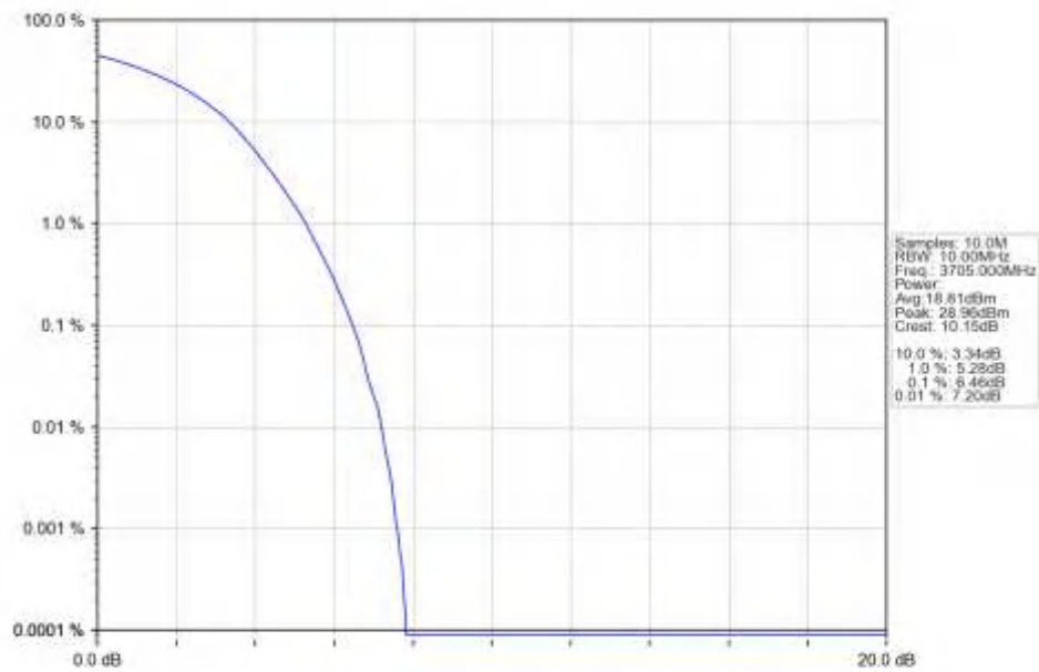
n78a_15kHz_SISO_NTNV_10MHz_DFT-s-OFDM_256_QAM_3705MHz_Outer_Full_Ant1
