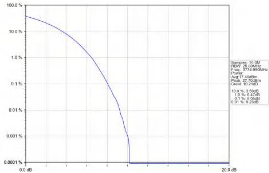
n78a_15kHz_SISO_NTNV_50MHz_CP-OFDM_16_QAM_3774.99MHz_Outer_Full_Ant1
