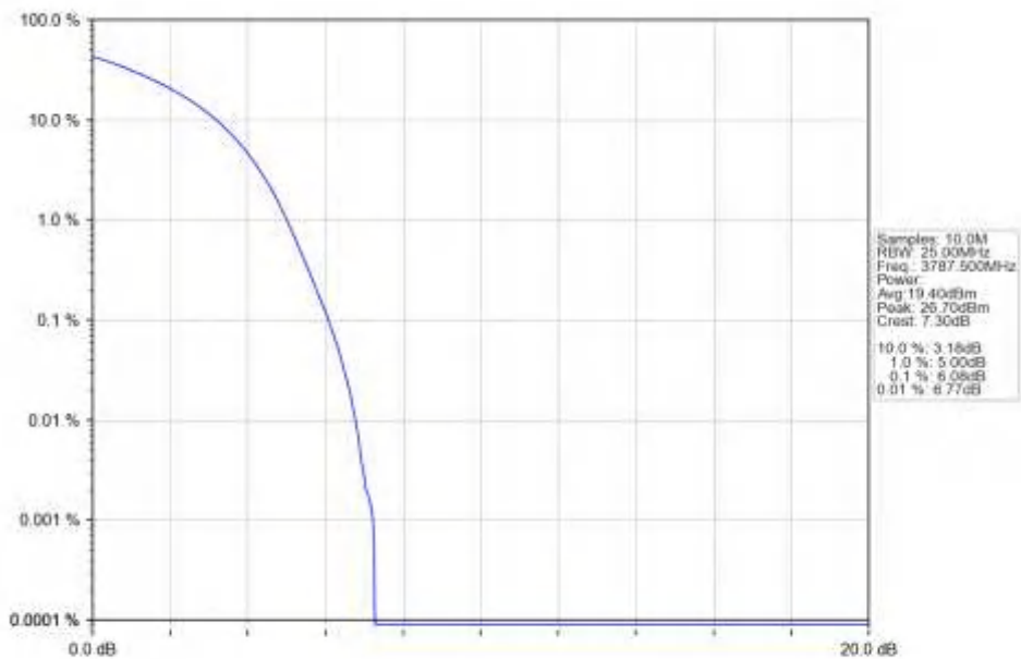
n78a_15kHz_SISO_NTNV_25MHz_DFT-s-OFDM_64_QAM_3787.5MHz_Outer_Full_Ant1
