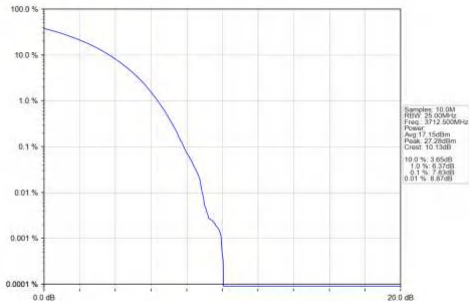
n78a_15kHz_SISO_NTNV_25MHz_CP-OFDM_256_QAM_3712.5MHz_Outer_Full_Ant1
