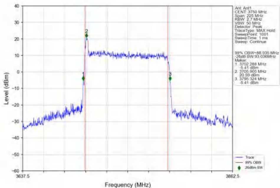
n78a_30kHz_SISO_NTNV_90MHz_DFT-s-OFDM QPSK_3750MHz_Outer_Full_Ant1
