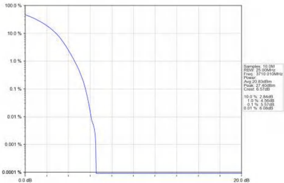
n78a_15kHz_SISO_NTNV_20MHz_DFT-s-OFDM_16_QAM_3710.01MHz_Outer_Full_Ant1
