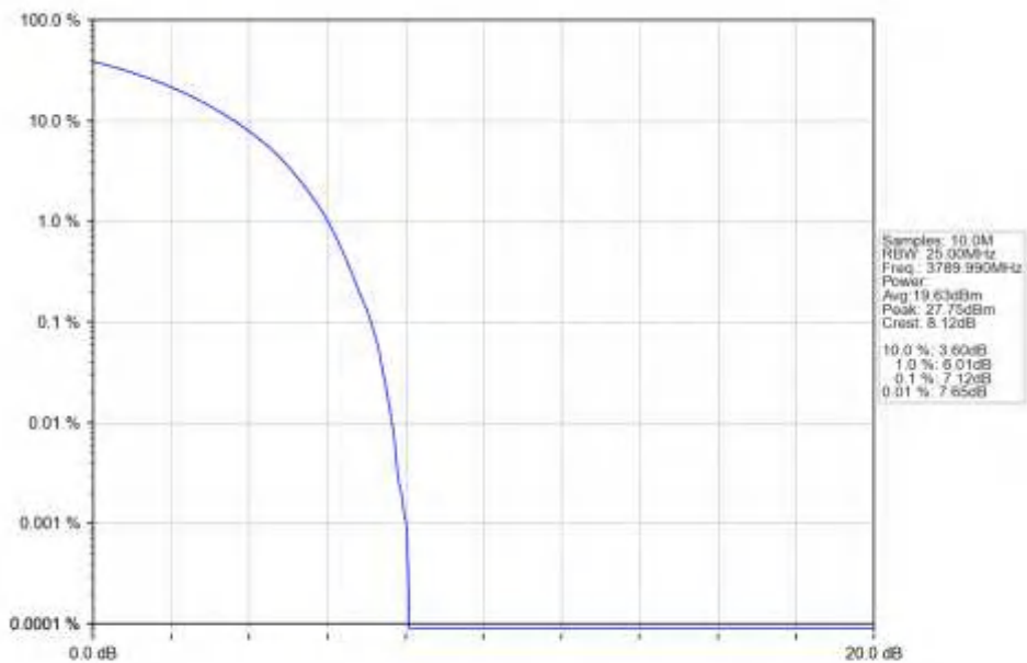
n78a_15kHz_SISO_NTNV_20MHz_CP-OFDM_QPSK_3789.99MHz_Outer_Full_Ant1
