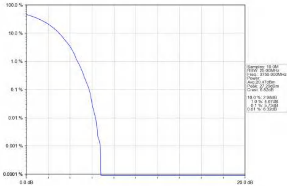
n78a_30kHz_SISO_NTNV_15MHz_DFT-s-OFDM_16_QAM_3750MHz_Outer_Full_Ant1
