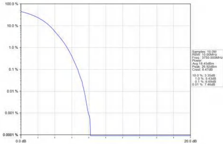
n78a_15kHz_SISO_NTNV_10MHz_DFT-s-OFDM_256_QAM_3750MHz_Outer_Full_Ant1
