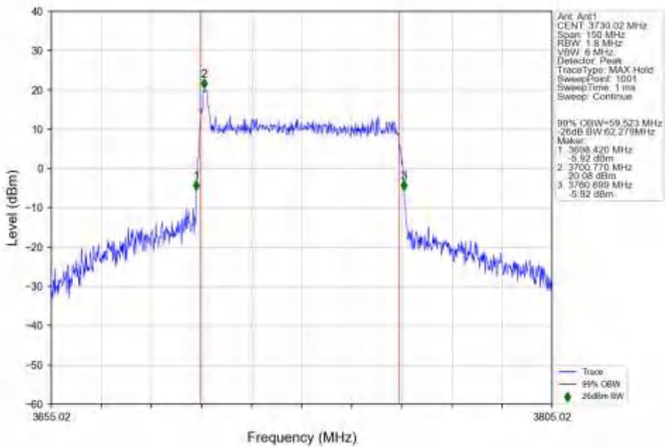
n78a_30kHz_SISO_NTNV_60MHz_CP-OFDM_16_QAM_3730.02MHz_Outer_Full_Ant1
