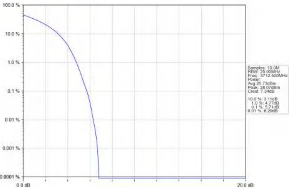
n78a_15kHz_SISO_NTNV_25MHz_DFT-s-OFDM_16_QAM_3712.5MHz_Outer_Full_Ant1
