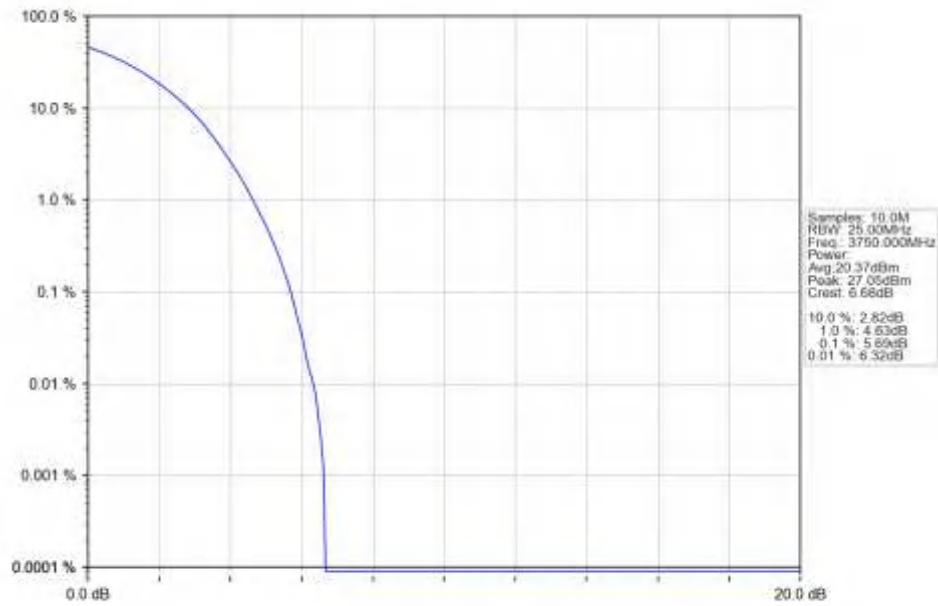
n78a_15kHz_SISO_NTNV_15MHz_DFT-s-OFDM_16_QAM_3750MHz_Outer_Full_Ant1
