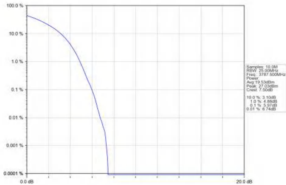
n78a_15kHz_SISO_NTNV_25MHz_DFT-s-OFDM_16_QAM_3787.5MHz_Outer_Full_Ant1
