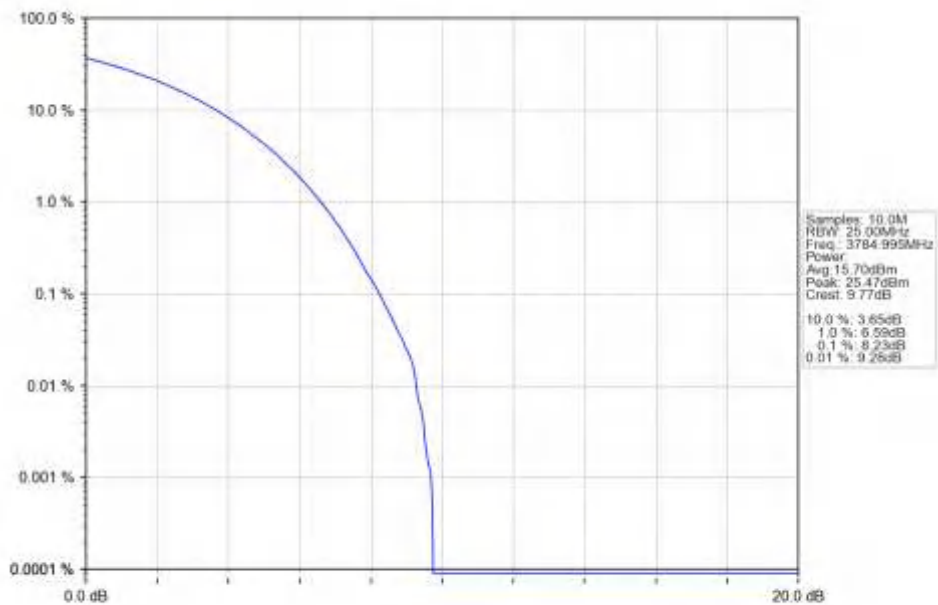
n78a_15kHz_SISO_NTNV_30MHz_CP-OFDM_256_QAM_3784.995MHz_Outer_Full_Ant1
