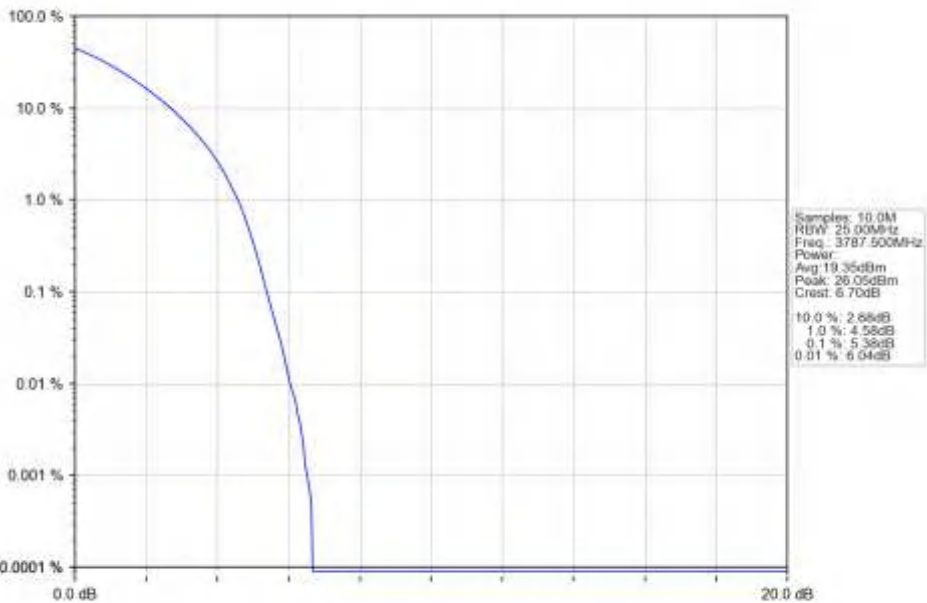
n78a_15kHz_SISO_NTNV_25MHz_DFT-s-OFDM_QPSK_3787.5MHz_Outer_Full_Ant1
