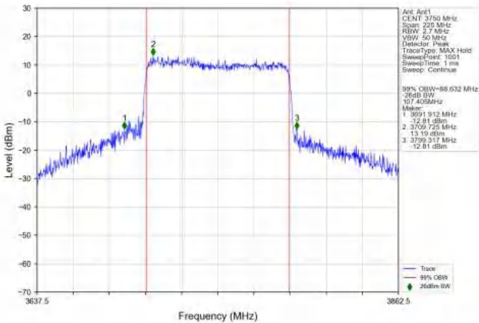
n78a 30kHz SISO_NTNV_90MHz_CP-OFDM_QPSK_3750MHz_Outer_Full_Ant1
