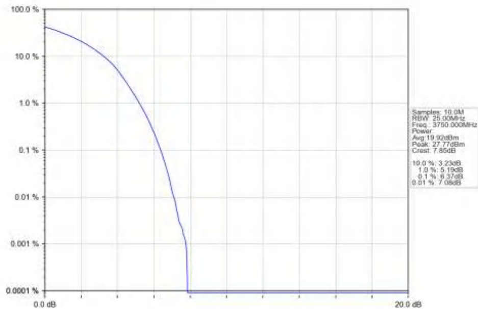
n78a_15kHz_SISO_NTNV_30MHz_DFT-s-OFDM_64_QAM_3750MHz_Outer_Full_Ant1
