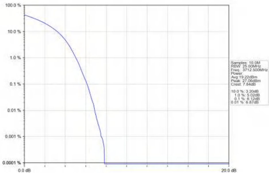
n78a_15kHz_SISO_NTNV_25MHz_DFT-s-OFDM_256_QAM_3712.5MHz_Outer_Full_Ant1
