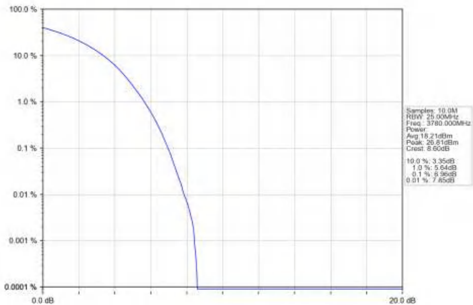
n78a_15kHz_SISO_NTNV_40MHz_DFT-s-OFDM_16_QAM_3780MHz_Outer_Full_Ant1
