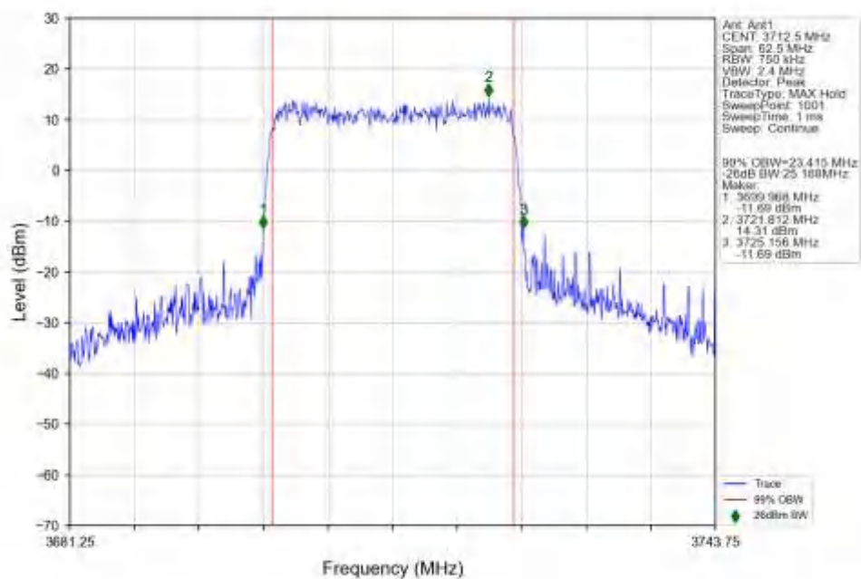
n78a_30kHz_SISO_NTNV_25MHz_CP-OFDM_256_QAM_3712.5MHz_Outer_Full_Ant1
