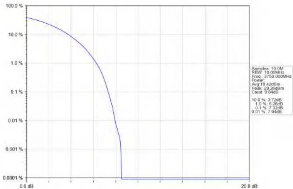
n78a_15kHz_SISO_NTNV_10MHz_CP-OFDM_64_QAM_3750MHz_Outer_Full_Ant1
