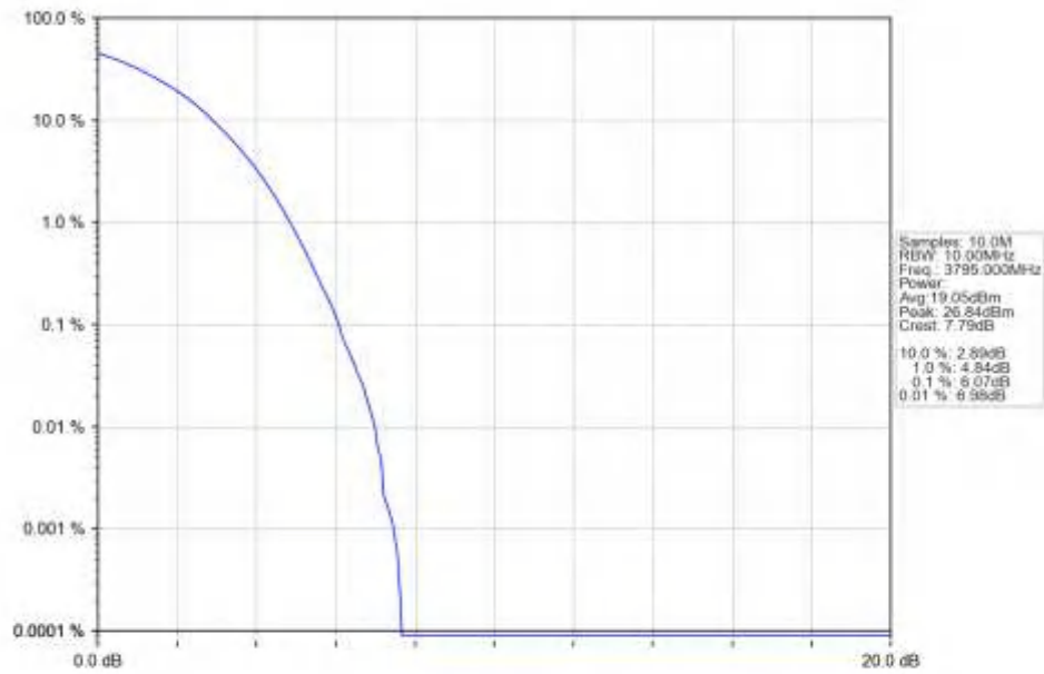
n78a_15kHz_SISO_NTNV_10MHz_DFT-s-OFDM_64_QAM_3795MHz_Outer_Full_Ant1
