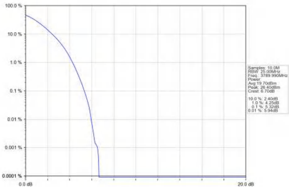
n78a_15kHz_SISO_NTNV_20MHz_DFT-s-OFDM_QPSK_3789.99MHz_Outer_Full_Ant1
