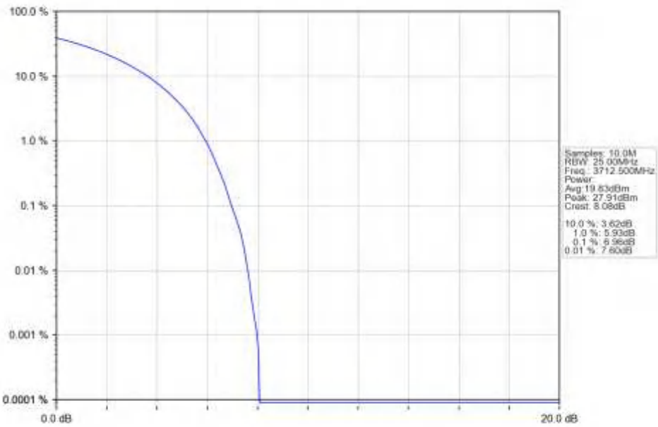
n78a_15kHz_SISO_NTNV_25MHz_CP-OFDM_64_QAM_3712.5MHz_Outer_Full_Ant1
