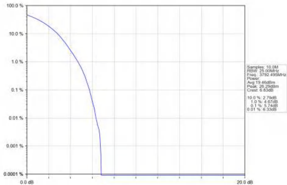
n78a_15kHz_SISO_NTNV_15MHz_DFT-s-OFDM_16_QAM_3792.495MHz_Outer_Full_Ant1
