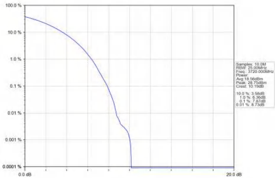
n78a_15kHz_SISO_NTNV_40MHz_CP-OFDM_64_QAM_3720MHz_Outer_Full_Ant1
