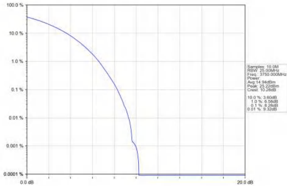
n78a_15kHz_SISO_NTNV_50MHz_CP-OFDM_256_QAM_3750MHz_Outer_Full_Ant1
