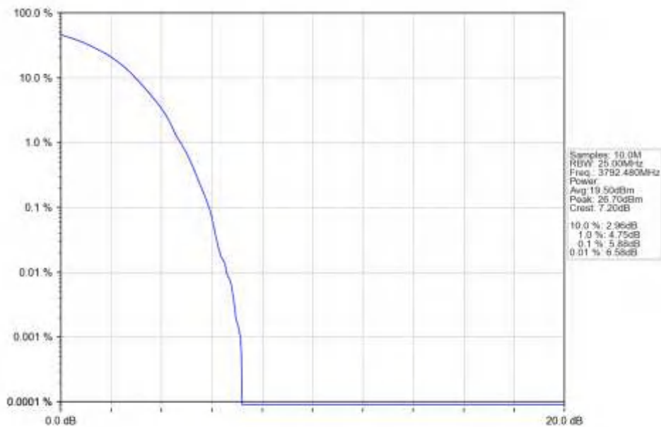
n78a_30kHz_SISO_NTNV_15MHz_DFT-s-OFDM_16_QAM_3792.48MHz_Outer_Full_Ant1
