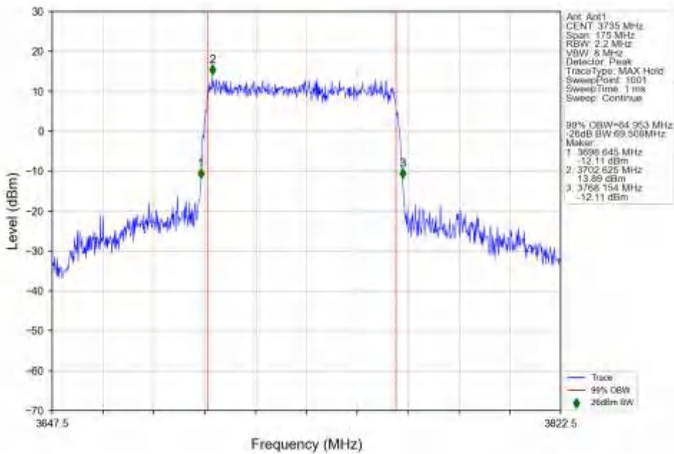
n78a_30kHz_SISO_NTNV_70MHz_DFT-s-OFDM_16_QAM_3735MHz_Outer_Full_Ant1
