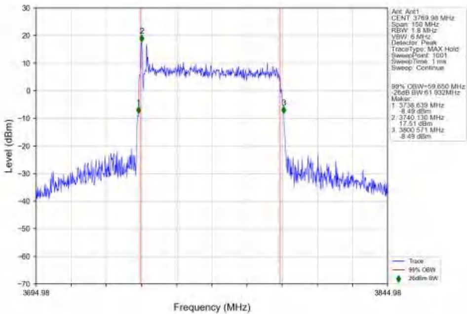
n78a_30kHz_SISO_NTNV_60MHz_CP-OFDM_256_QAM_3769.98MHz_Outer_Full_Ant1
