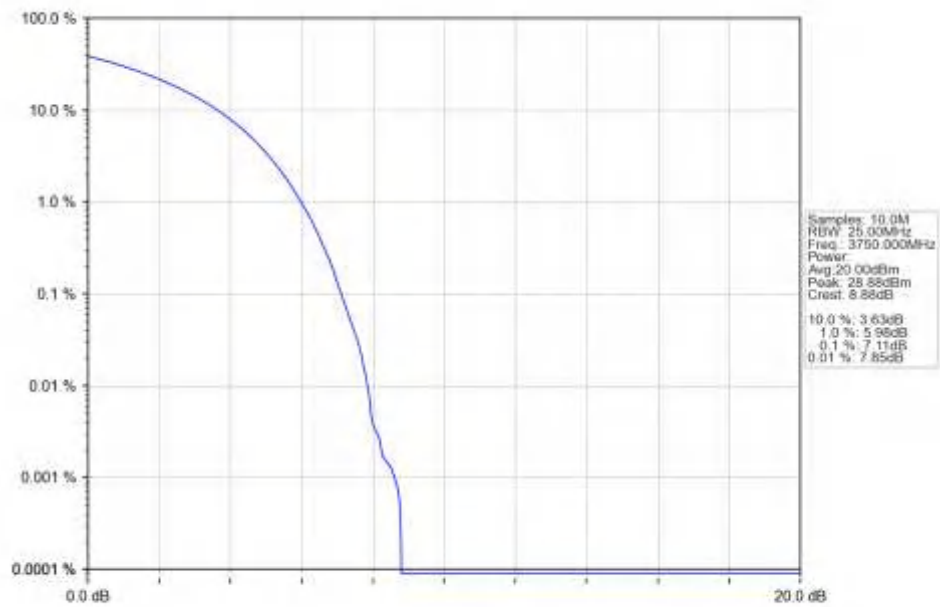
n78a_15kHz_SISO_NTNV_25MHz_CP-OFDM_QPSK_3750MHz_Outer_Full_Ant1
