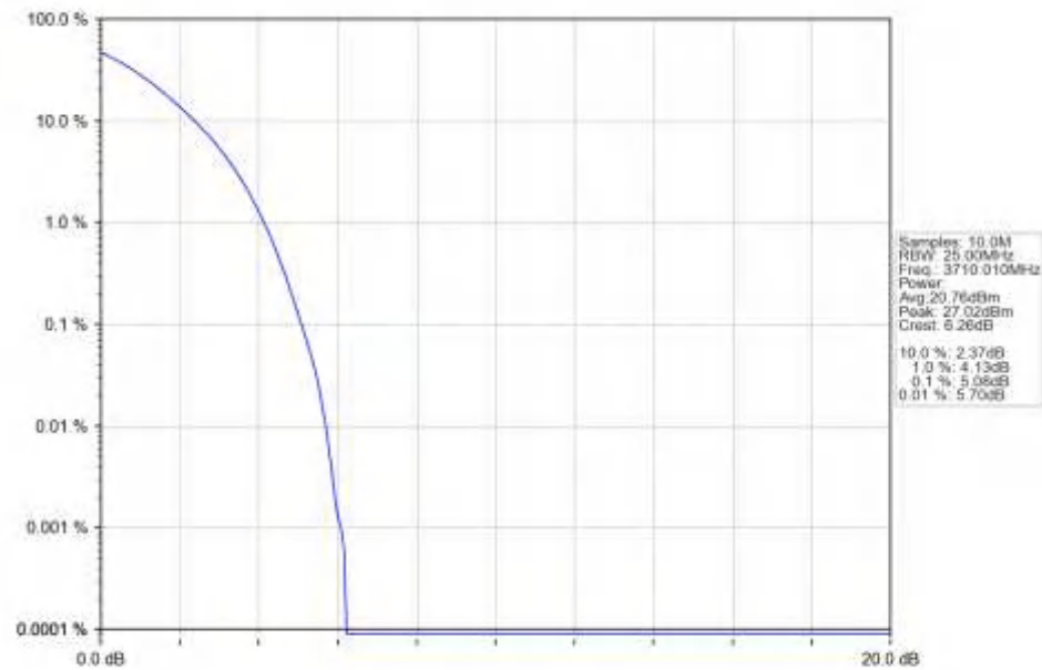
n78a_15kHz_SISO_NTNV_20MHz_DFT-s-OFDM_QPSK_3710.01MHz_Outer_Full_Ant1
