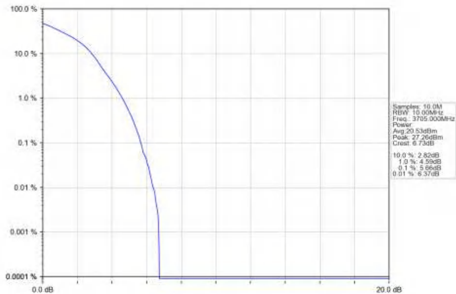
n78a_15kHz_SISO_NTNV_10MHz_DFT-s-OFDM_16_QAM_3705MHz_Outer_Full_Ant1
