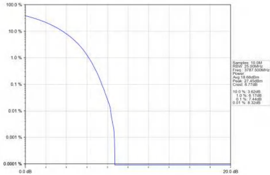
n78a_15kHz_SISO_NTNV_25MHz_CP-OFDM_64_QAM_3787.5MHz_Outer_Full_Ant1
