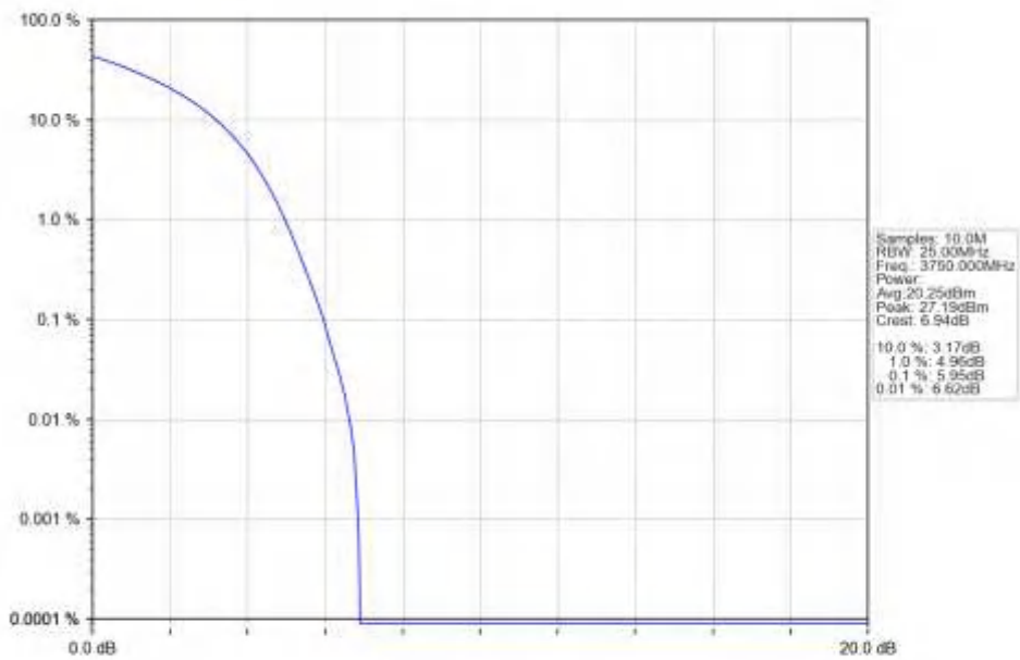
n78a_15kHz_SISO_NTNV_25MHz_DFT-s-OFDM_64_QAM_3750MHz_Outer_Full_Ant1
