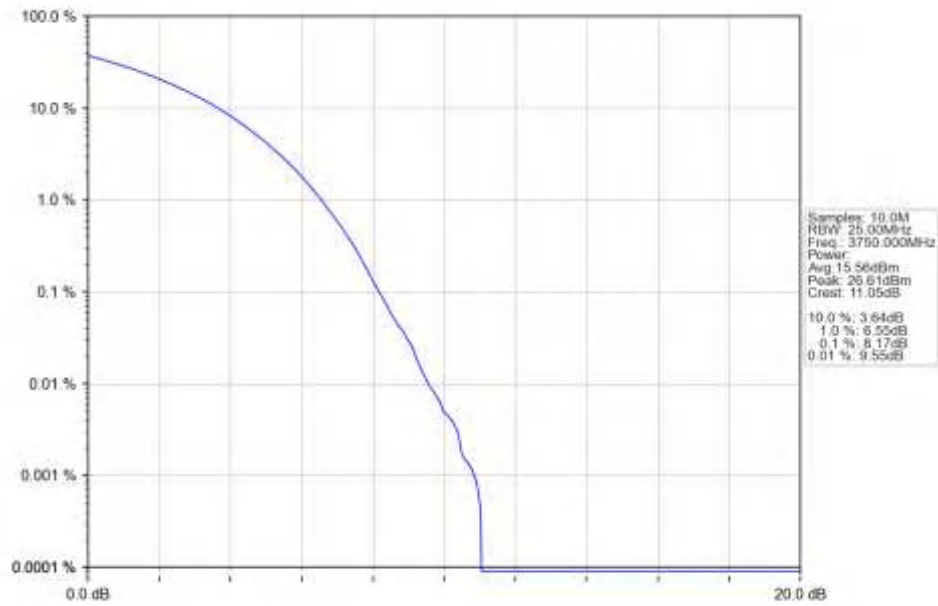
n78a_15kHz_SISO_NTNV_40MHz_CP-OFDM_256_QAM_3750MHz_Outer_Full_Ant1
