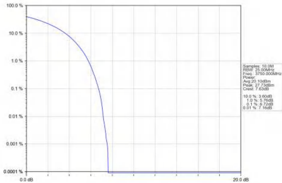
n78a_15kHz_SISO_NTNV_15MHz_CP-OFDM_QPSK_3750MHz_Outer_Full_Ant1
