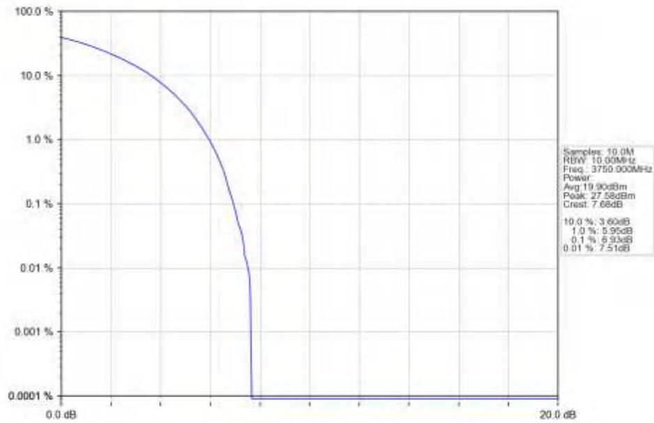
n78a 15kHz SISO NTN 10MHz CP-OFDM 16 QAM 3750MHz Outer Full Ant1
