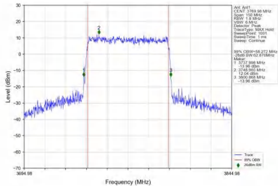
n78a_30kHz_SISO_NTNV_60MHz_DFT-s-OFDM_256_QAM_3769.98MHz_Outer_Full_Ant1
