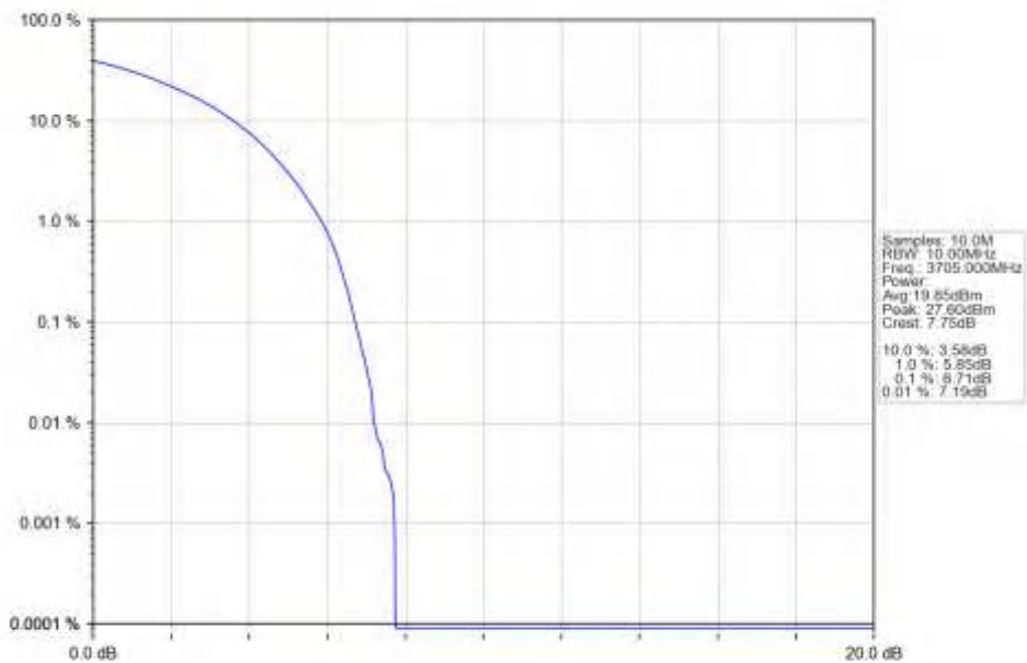
n78a_15kHz_SISO_NTNV_10MHz_CP-OFDM_64_QAM_3705MHz_Outer_Full_Ant1
