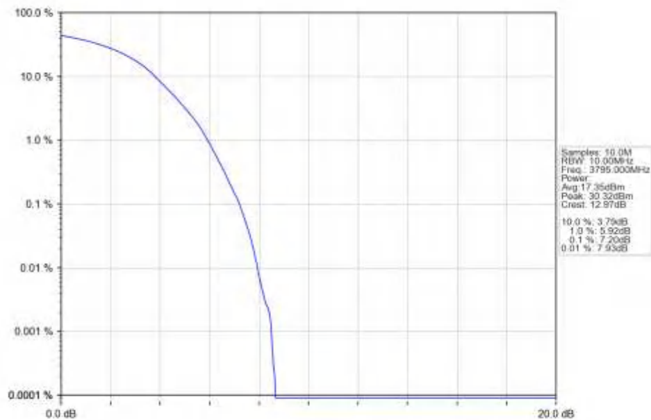
n78a_15kHz_SISO_NTNV_10MHz_DFT-s-OFDM_256_QAM_3795MHz_Outer_Full_Ant1
