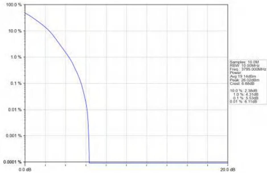
n78a_15kHz_SISO_NTNV_10MHz_DFT-s-OFDM_QPSK_3795MHz_Outer_Full_Ant1
