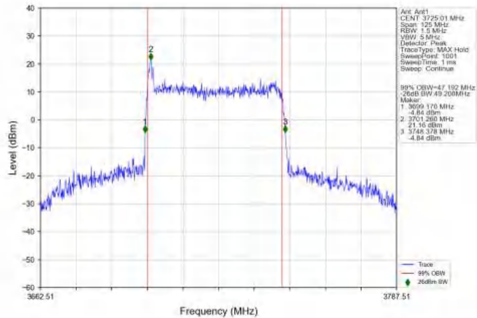
n78a_30kHz_SISO_NTNV_50MHz_DFT-s-OFDM_16_QAM_3725.01MHz_Outer_Full_Ant1
