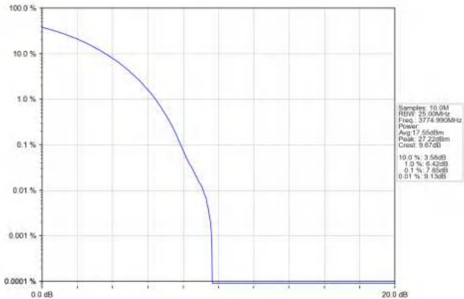
n78a_15kHz_SISO_NTNV_50MHz_CP-OFDM_QPSK_3774.99MHz_Outer_Full_Ant1
