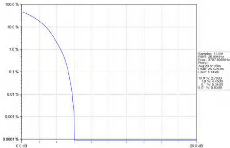
n78a_15kHz_SISO_NTNV_15MHz_DFT-s-OFDM_16_QAM_3707.505MHz_Outer_Full_Ant1
