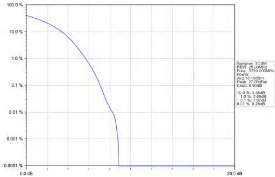
n78a_15kHz_SISO_NTNV_40MHz_DFT-s-OFDM_64_QAM_3780MHz_Outer_Full_Ant1
