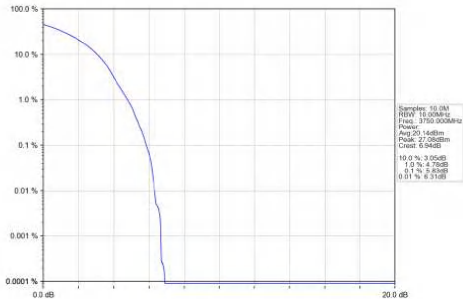
n78a_30kHz_SISO_NTNV_10MHz_DFT-s-OFDM_64_QAM_3750MHz_Outer_Full_Ant1
