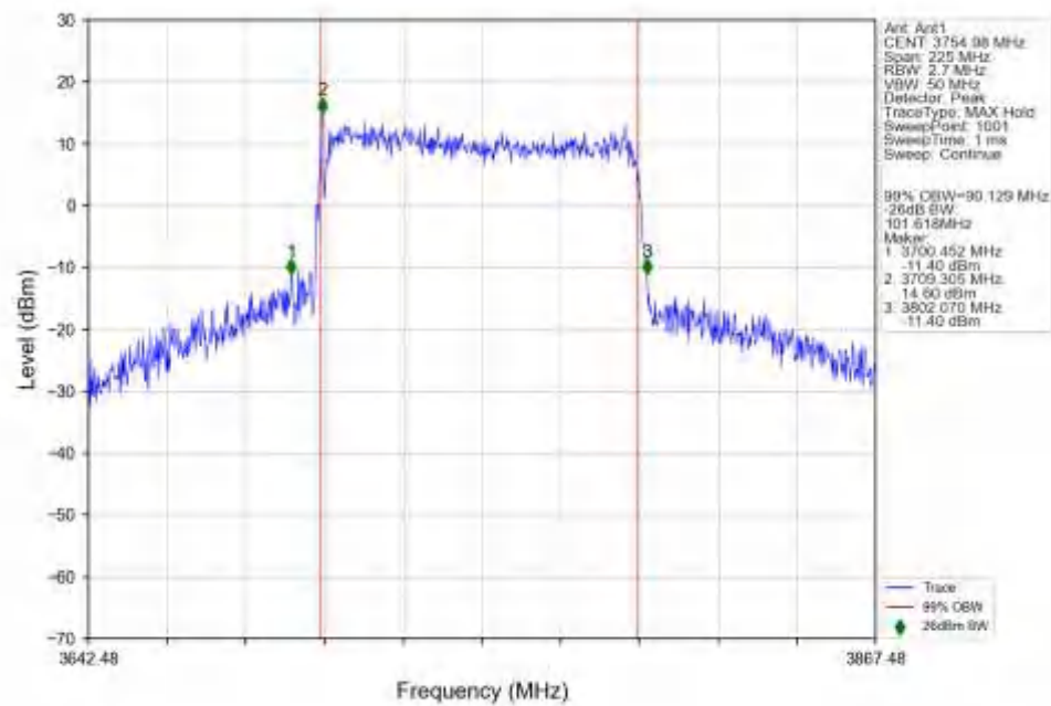
n78a_30kHz_SISO_NTNV_90MHz_CP-OFDM_16_QAM_3754.98MHz_Outer_Full_Ant1
