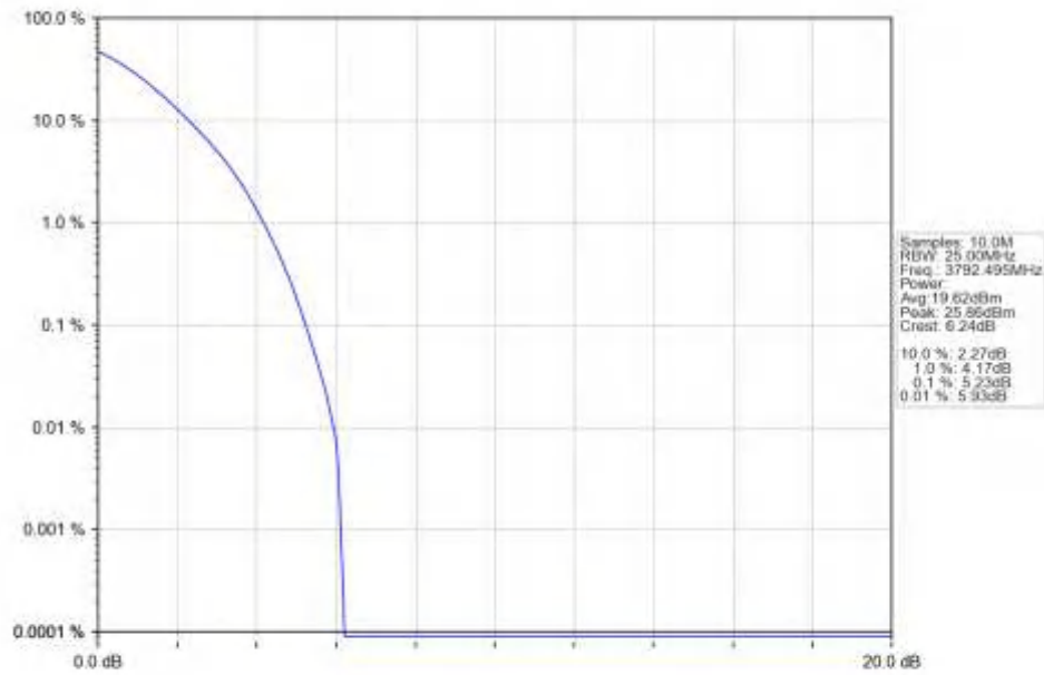
n78a_15kHz_SISO_NTNV_15MHz_DFT-s-OFDM_QPSK_3792.495MHz_Outer_Full_Ant1
