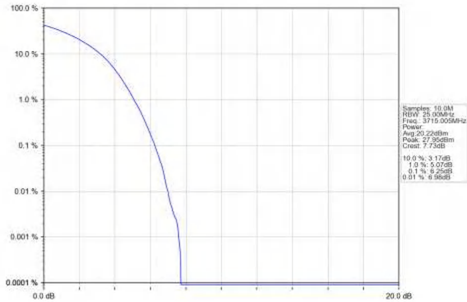
n78a_15kHz_SISO_NTNV_30MHz_DFT-s-OFDM_64_QAM_3715.005MHz_Outer_Full_Ant1
