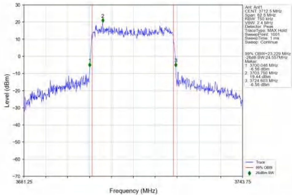
n78a 30kHz SISO NTN 25MHz DFT-s-OFDM 16 QAM 3712.5MHz Outer Full Ant1
