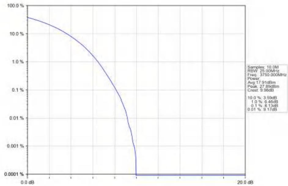
n78a_15kHz_SISO_NTNV_50MHz_CP-OFDM_16_QAM_3750MHz_Outer_Full_Ant1
