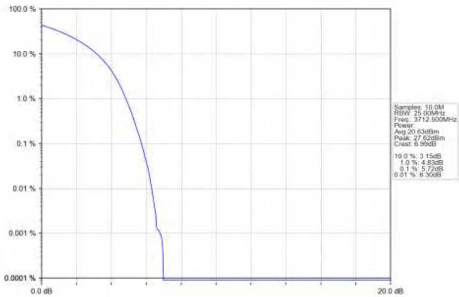
n78a_15kHz_SISO_NTNV_25MHz_DFT-s-OFDM_64_QAM_3712.5MHz_Outer_Full_Ant1
