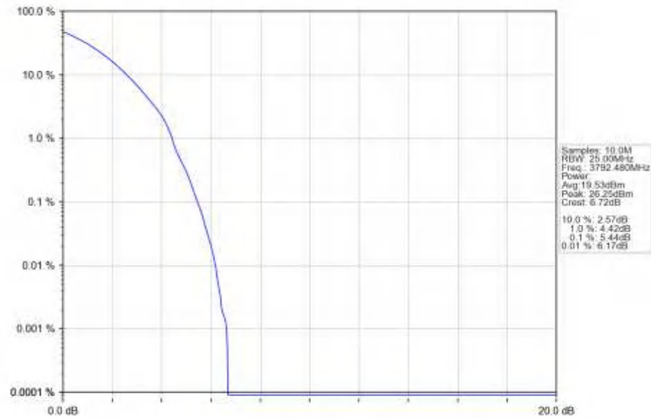
n78a_30kHz_SISO_NTNV_15MHz_DFT-s-OFDM_QPSK_3792.48MHz_Outer_Full_Ant1
