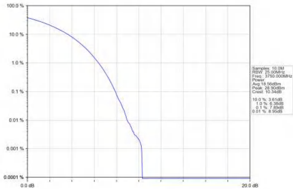
n78a 15kHz SISO NTN 40MHz CP-OFDM QPSK 3750MHz Outer Full Ant1
