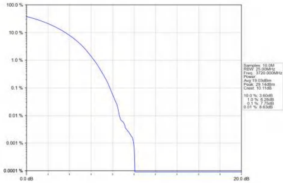
n78a 15kHz SISO NTN 40MHz CP-OFDM QPSK 3720MHz Outer Full Ant1
