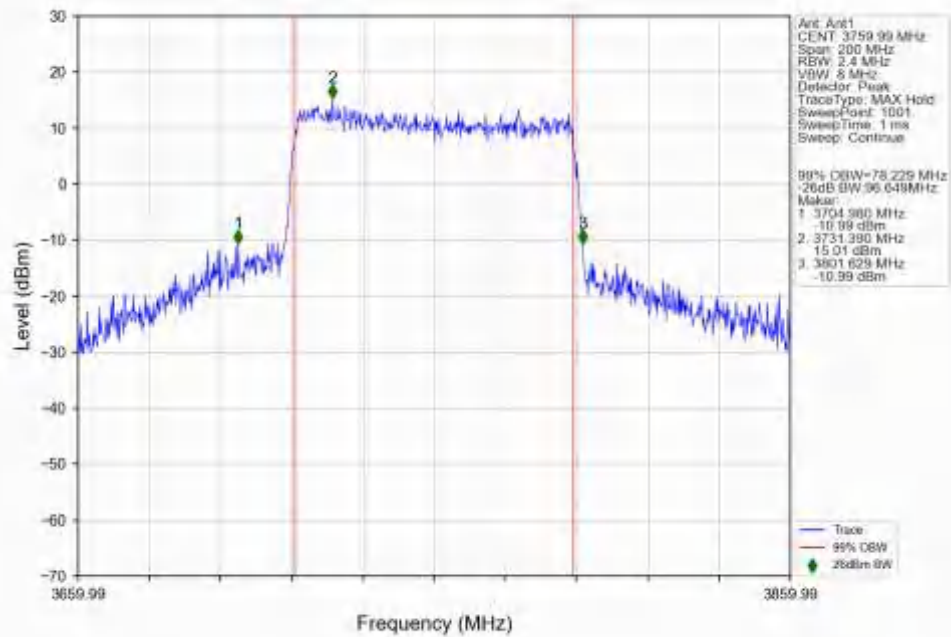
n78a_30kHz_SISO_NTNV_80MHz_CP-OFDM_16_QAM_3759.99MHz_Outer_Full_Ant1
