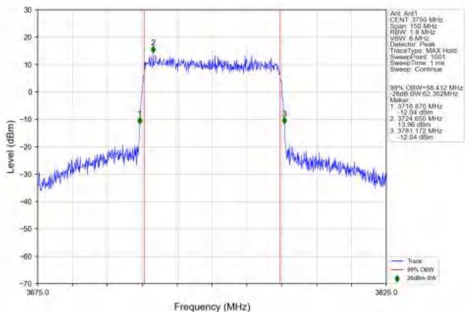
n78a_30kHz_SISO_NTNV_60MHz_DFT-s-OFDM_QPSK_3750MHz_Outer_Full_Ant1
