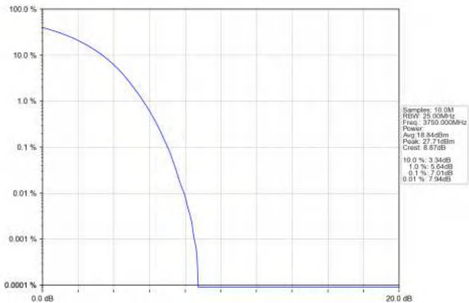
n78a_15kHz_SISO_NTNV_40MHz_DFT-s-OFDM_16_QAM_3750MHz_Outer_Full_Ant1
