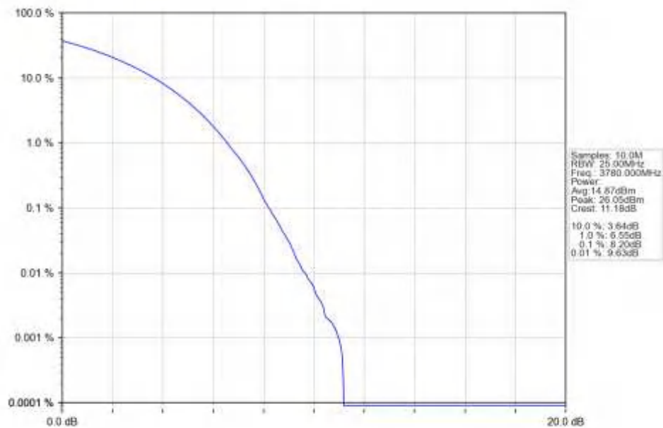
n78a_15kHz_SISO_NTNV_40MHz_CP-OFDM_256_QAM_3780MHz_Outer_Full_Ant1
