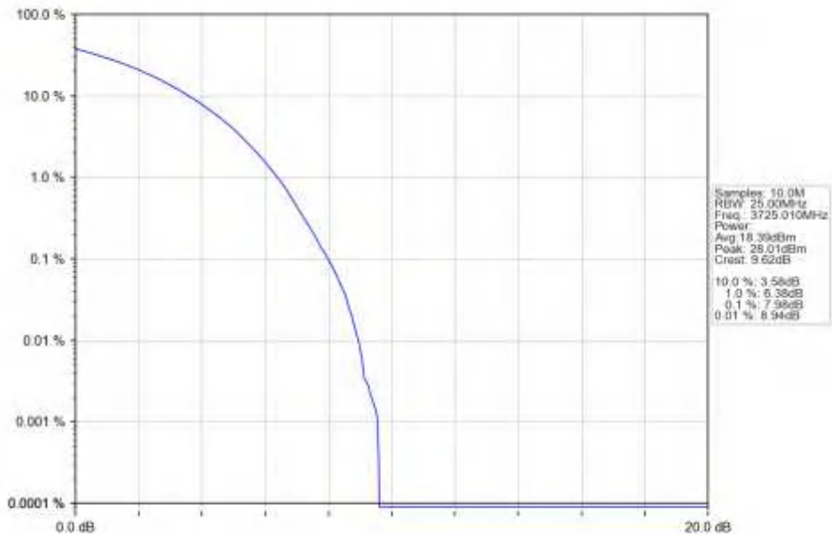
n78a_15kHz_SISO_NTNV_50MHz_CP-OFDM_16_QAM_3725.01MHz_Outer_Full_Ant1
