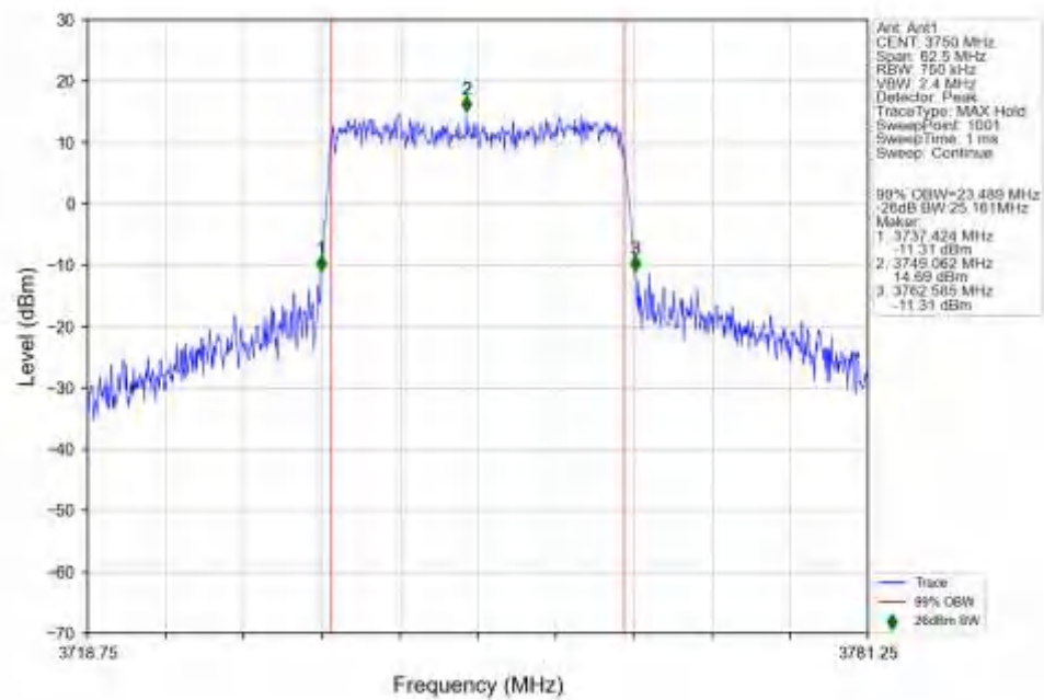
n78a_30kHz_SISO_NTNV_25MHz_CP-OFDM_64_QAM_3750MHz_Outer_Full_Ant1
