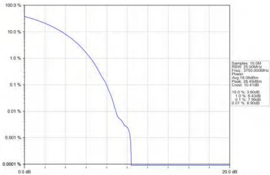
n78a_15kHz_SISO_NTNV_40MHz_CP-OFDM_64_QAM_3750MHz_Outer_Full_Ant1
