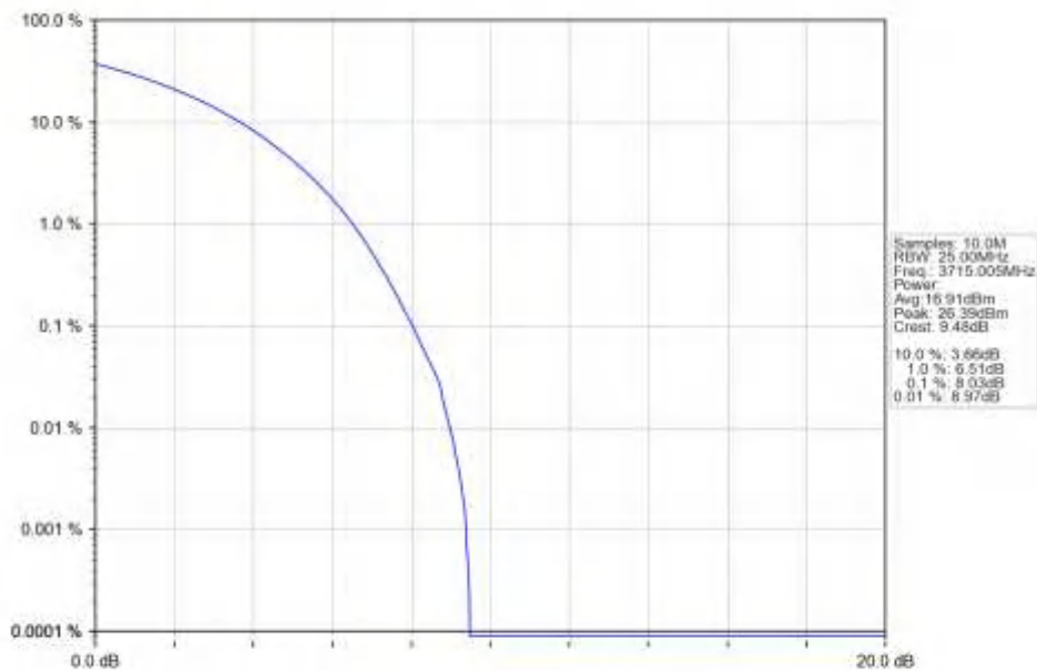
n78a_15kHz_SISO_NTNV_30MHz_CP-OFDM_256_QAM_3715.005MHz_Outer_Full_Ant1
