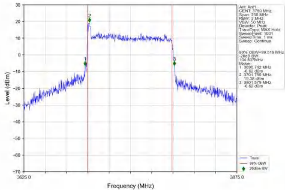
n78a_30kHz_SISO_NTNV_100MHz_CP-OFDM_16_QAM_3750MHz_Outer_Full_Ant1
