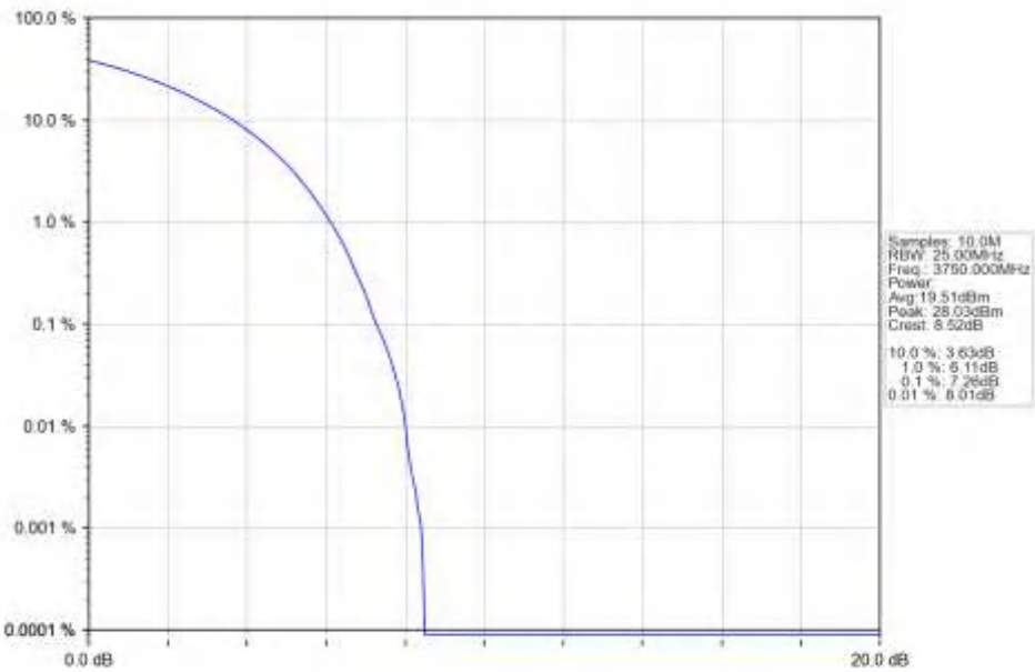
n78a_15kHz_SISO_NTNV_25MHz_CP-OFDM_64_QAM_3750MHz_Outer_Full_Ant1
