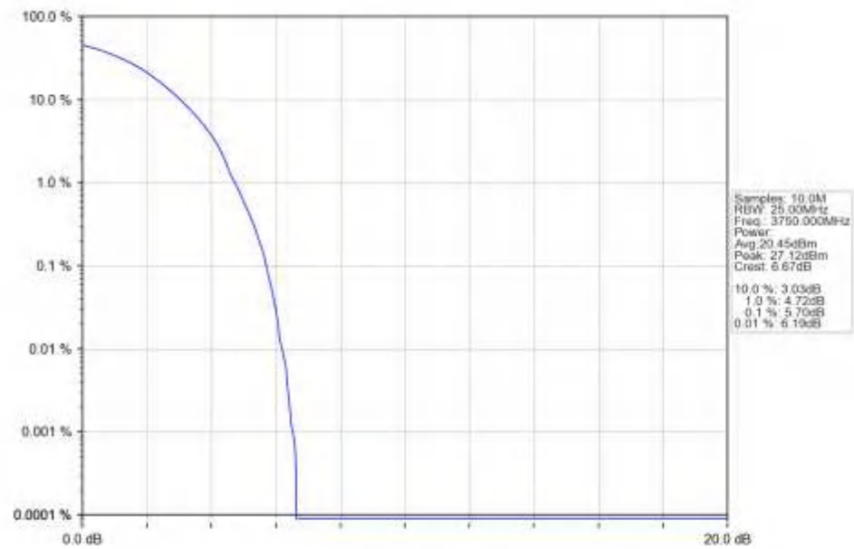
n78a_30kHz_SISO_NTNV_15MHz_DFT-s-OFDM_64_QAM_3750MHz_Outer_Full_Ant1
