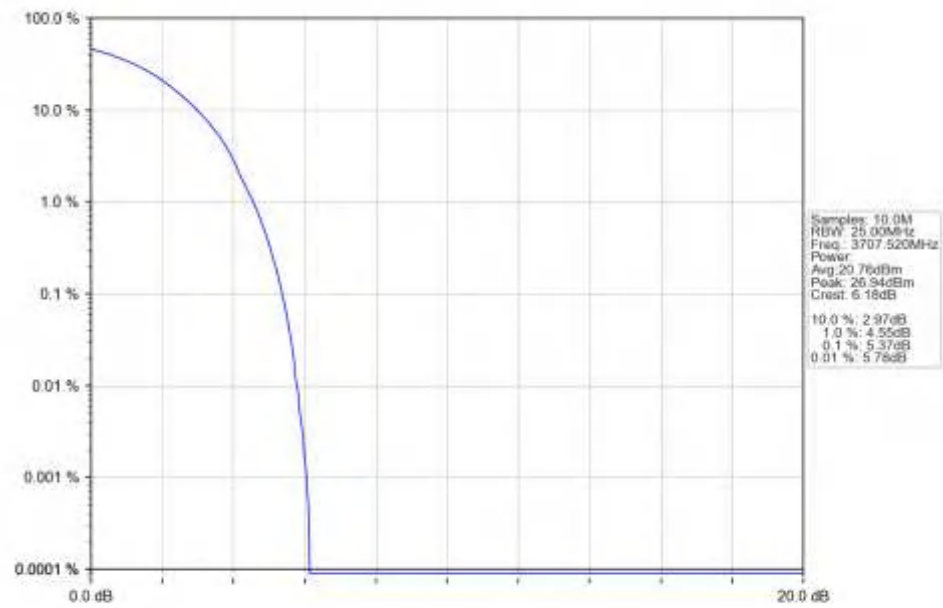
n78a_30kHz_SISO_NTNV_15MHz_DFT-s-OFDM_64_QAM_3707.52MHz_Outer_Full_Ant1
