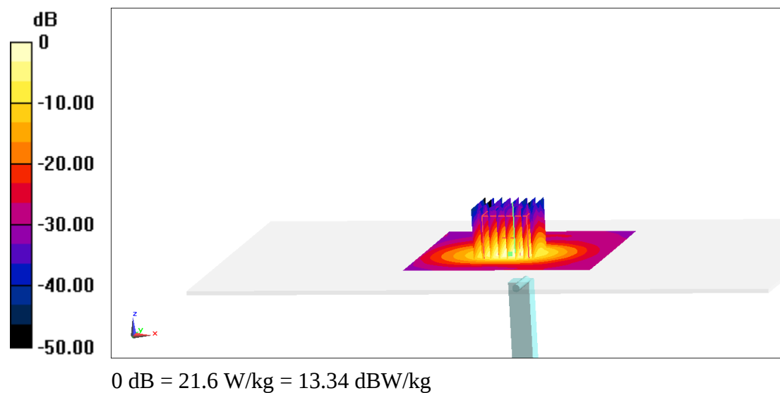
Fig.B.6 validation 5600 MHz 100mW
