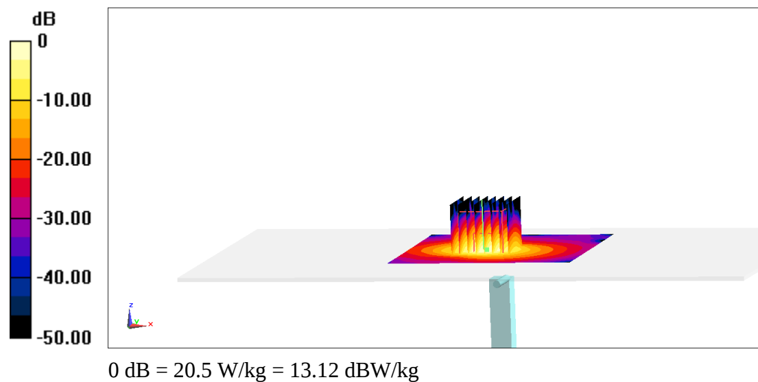
Fig.B.7 validation 5750 MHz 100mW
