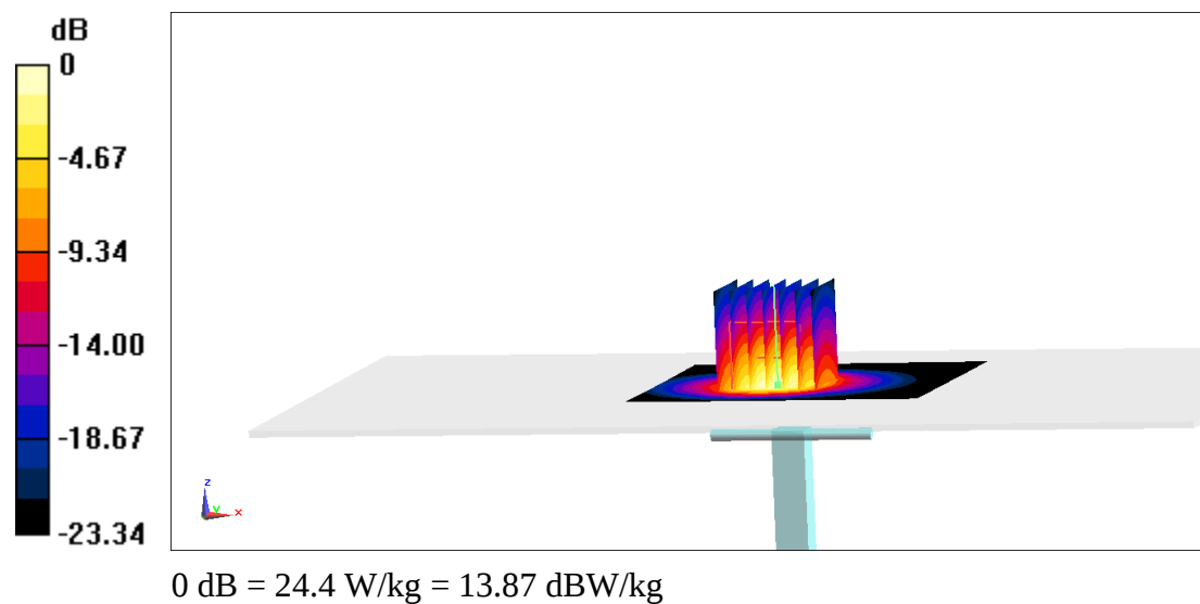
Fig.B.4 validation 2600 MHz 250mW
