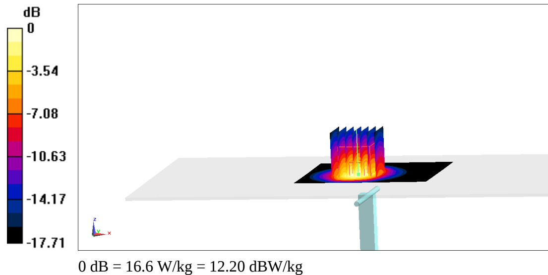
Fig.B.2 validation 1900 MHz 250mW
