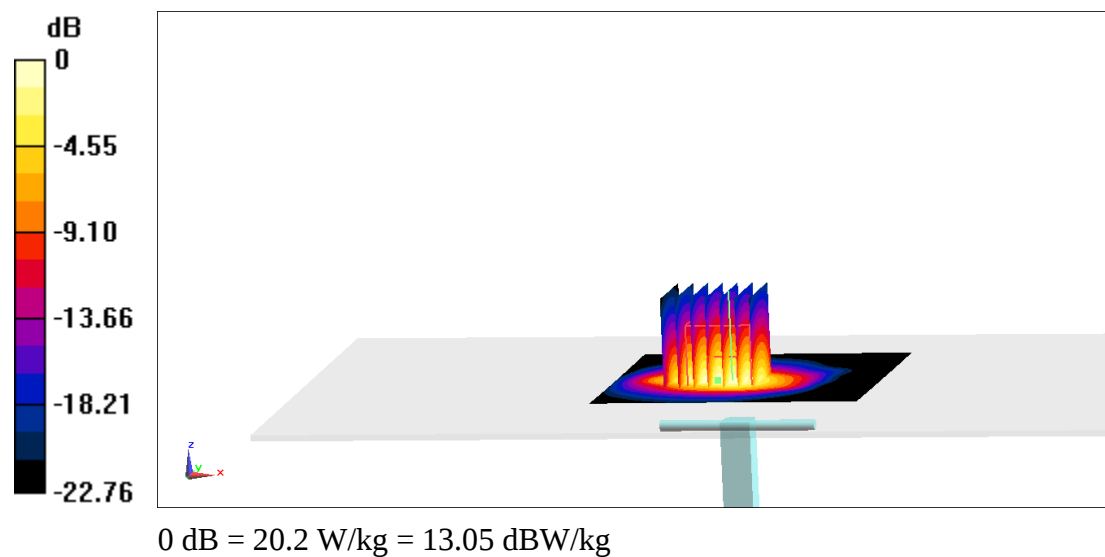
Fig.B.3 validation 2450 MHz 250mW
