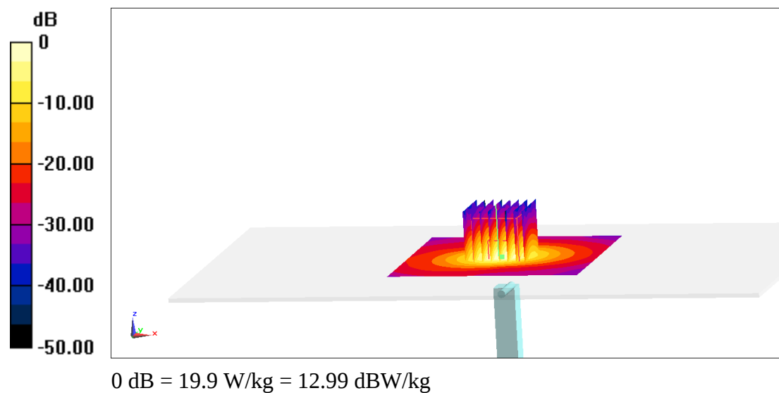
Fig.B.5 validation 5250 MHz 100mW
