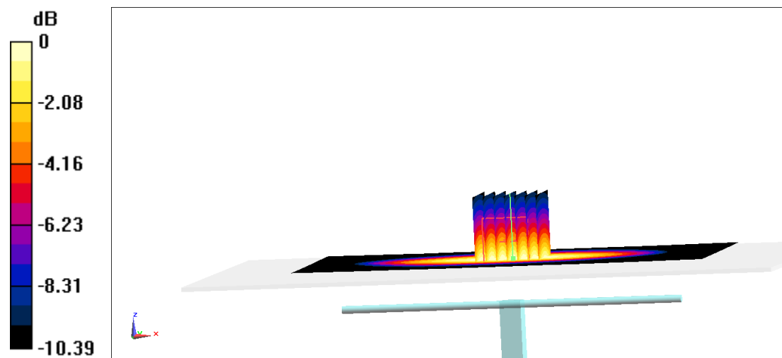
Fig.B.1 validation 835 MHz 250mW
