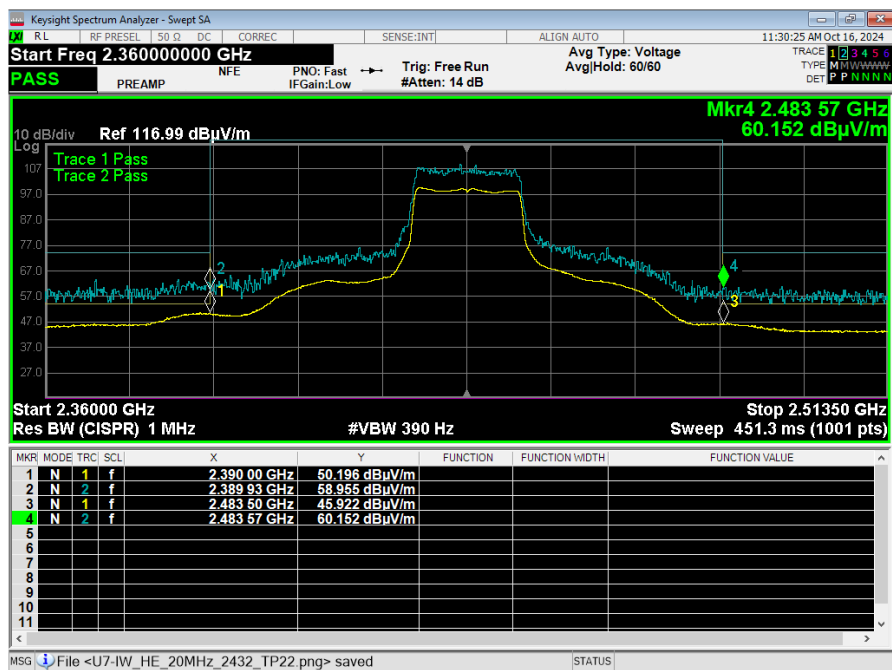
Graph 4: Radiated Middle Band Edge Plot ax 20 MHz
