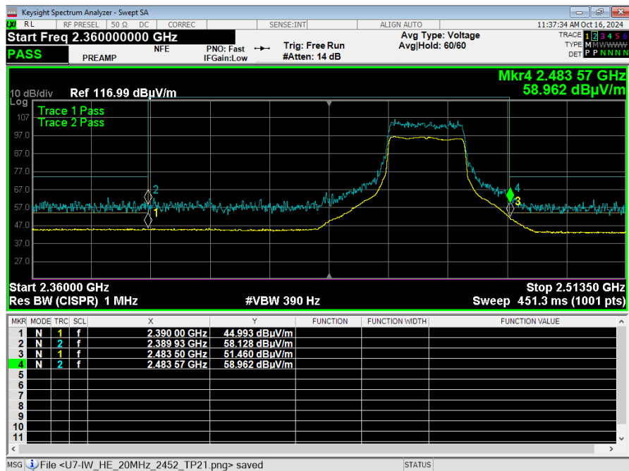
Graph 5: Radiated Upper Band Edge Plot ax 20 MHz
