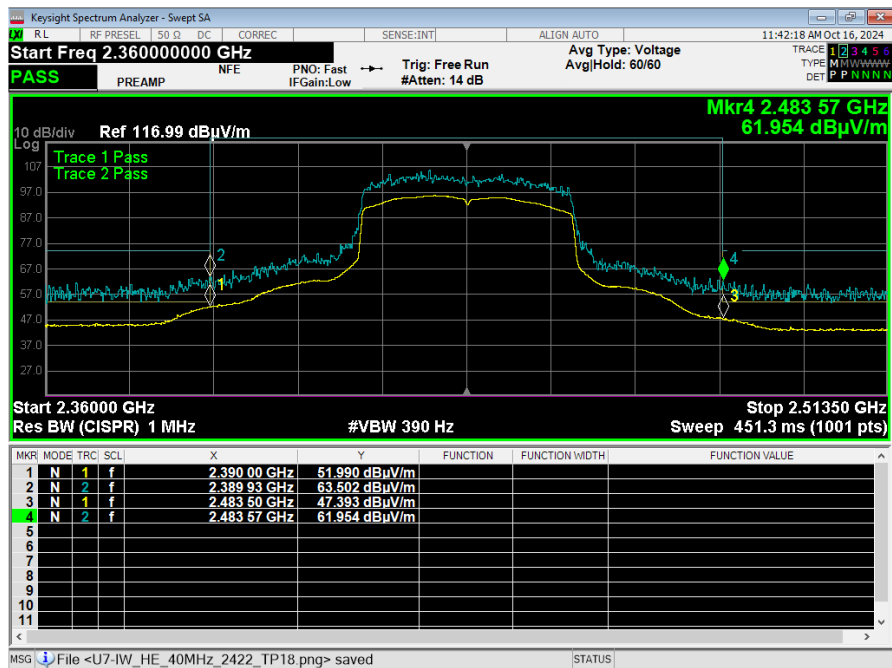
Graph 7: Radiated Middle Band Edge Plot ax 40 MHz
