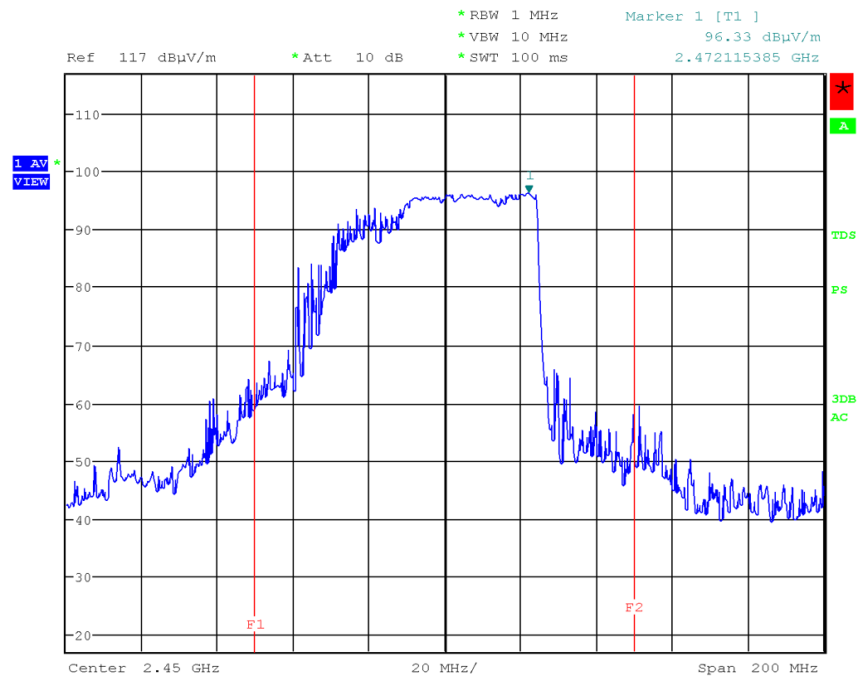
< Fig 9. Frequency Measurements_Load (Maximum Frequency Observed: 2.472 GHz) >
