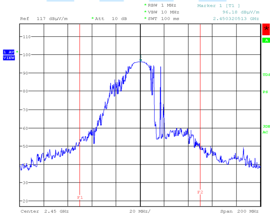
< Fig 8. Frequency Measurements _ Voltage (Minimum Frequency Observed: 2.450 GHz) >
