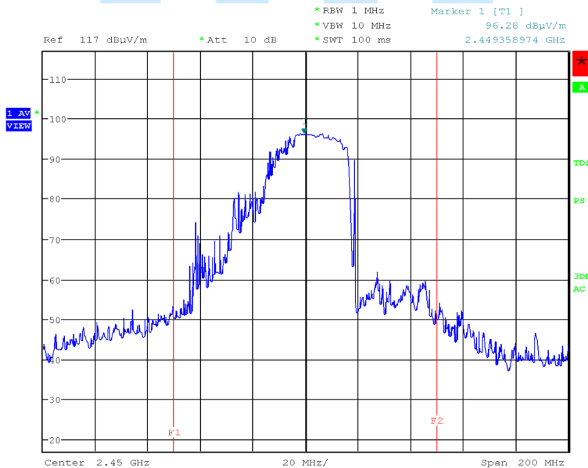
< Fig 10. Frequency Measurements_Load (Minimum Frequency Observed: 2.449 GHz) >
