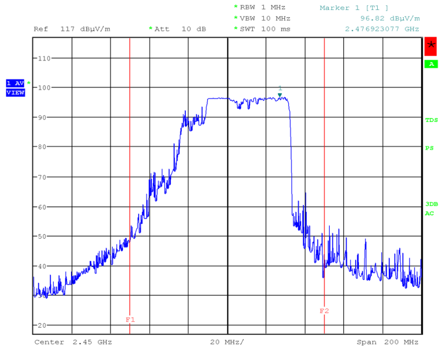
< Fig 7. Frequency Measurements _ Voltage (Maximum Frequency Observed: 2.476 GHz) >
