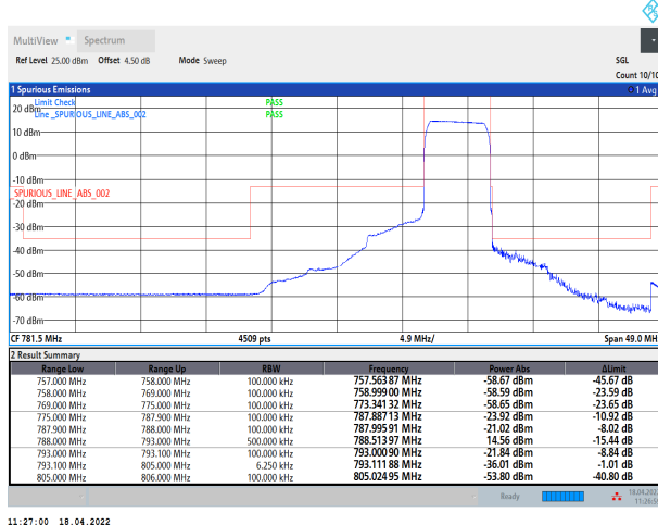
Band14-5MHz-QPSK-23305-25RB#0
