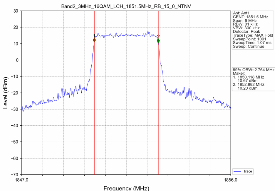
Band2_3MHz_16QAM_LCH_1851.5MHz_RB_15_0_NTNV
