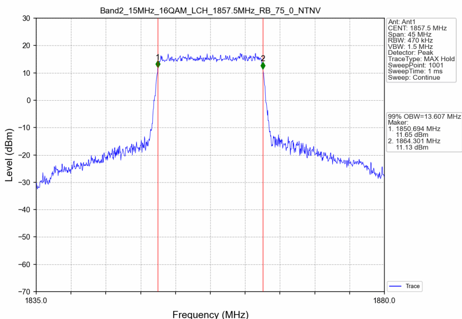
Band2_15MHz_16QAM_LCH_1857.5MHz_RB_75_0_NTNV
