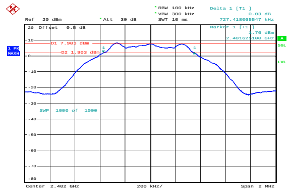
Low 0.727MHz
