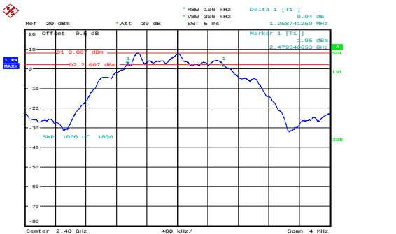
High 1.259MHz
