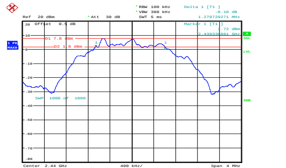
Middle 1.271MHz
