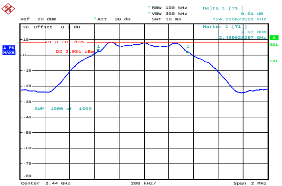
Middle 0.724MHz
