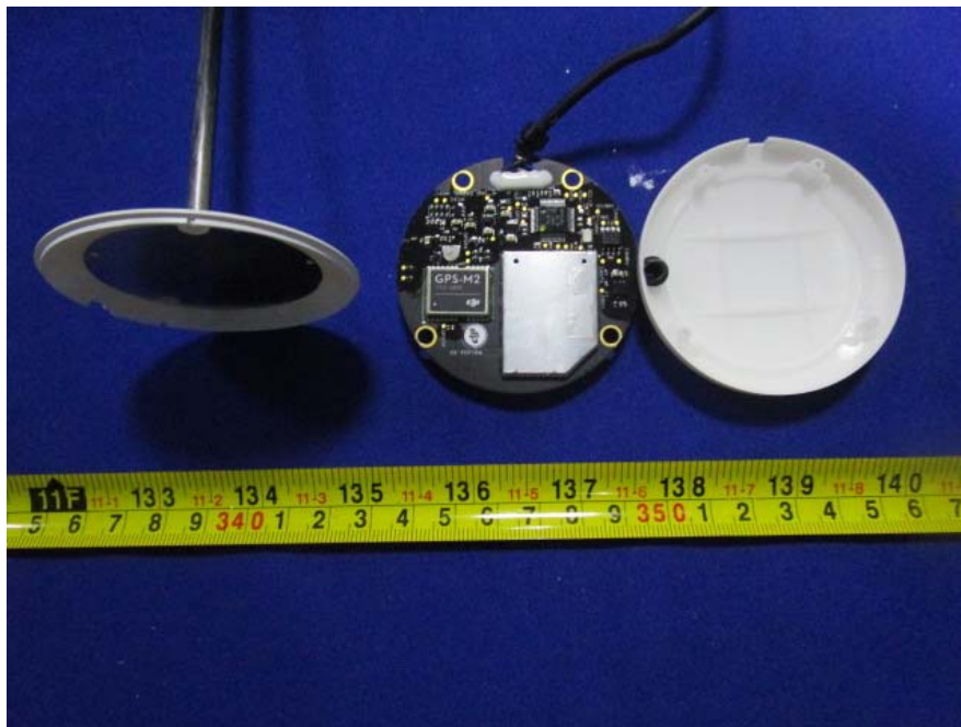
EUT –GPS Uncover View
