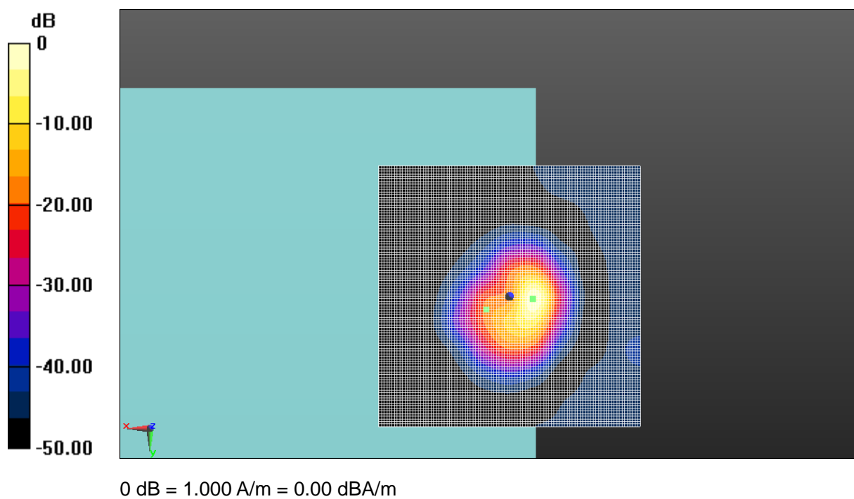
Fig A.37 T-Coil GSM 1900
