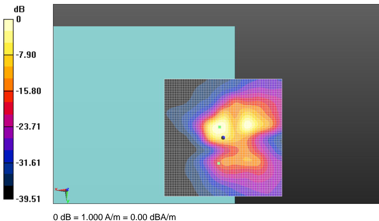
Fig A.48 T-Coil WIFI 2.4G
