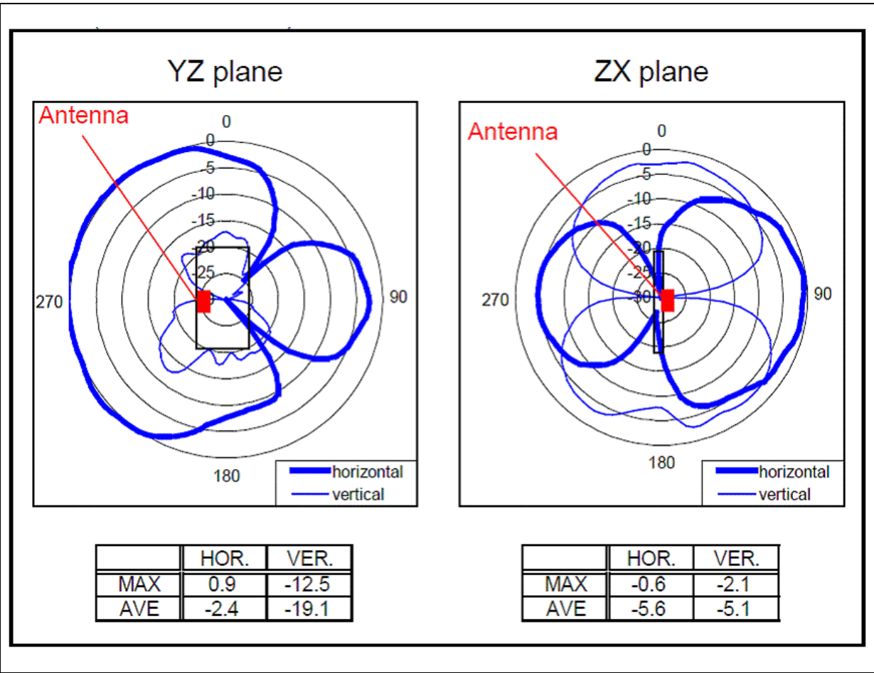
Figure 20. Radiation patterns of the built in antenna.
