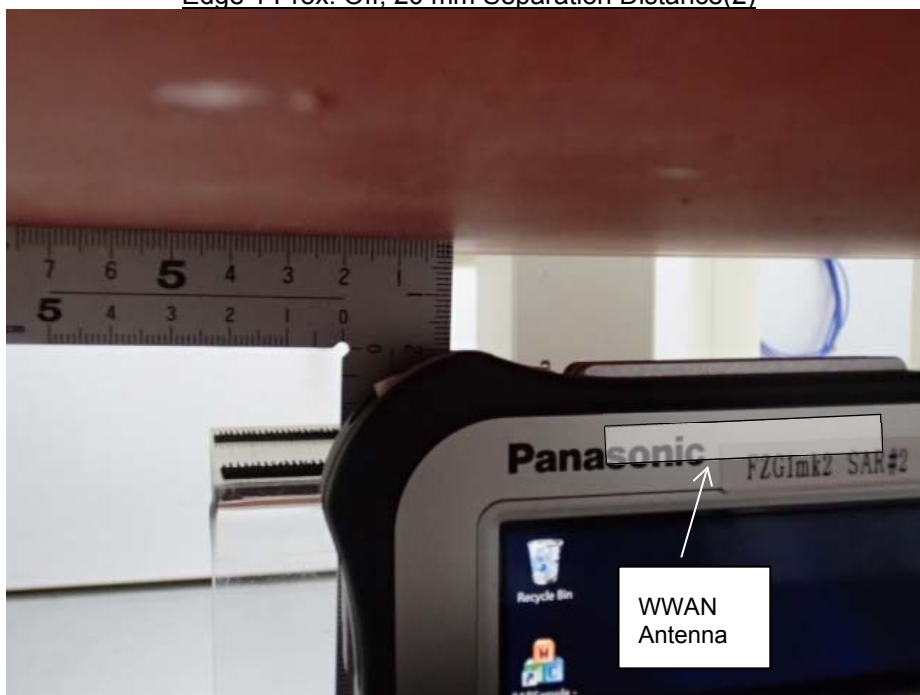
Edge 1 Prox. Off, 20 mm Separation Distance(2)
