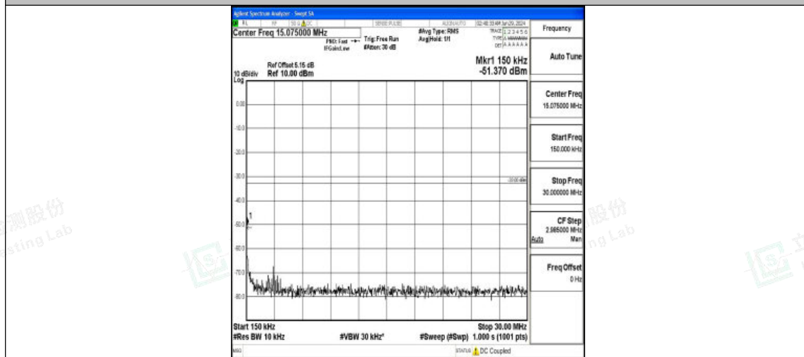
Band4_15MHz_16QAM_20325_1RB#0_0.15~30_0.15~30
