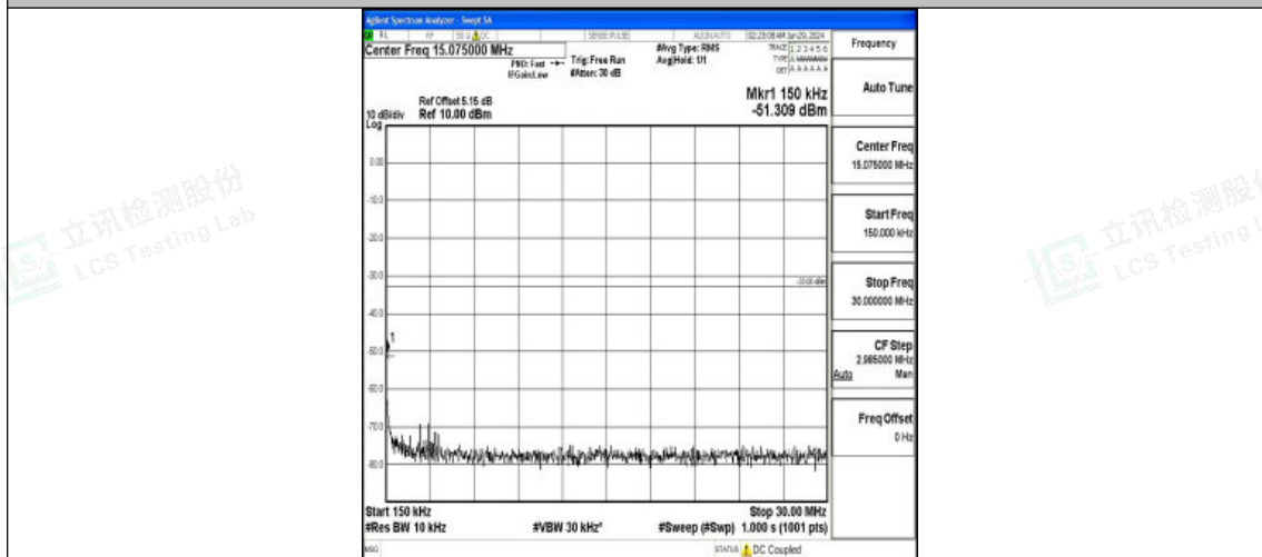
Band4_10MHz_QPSK_20350_1RB#0_0.15~30_0.15~30
