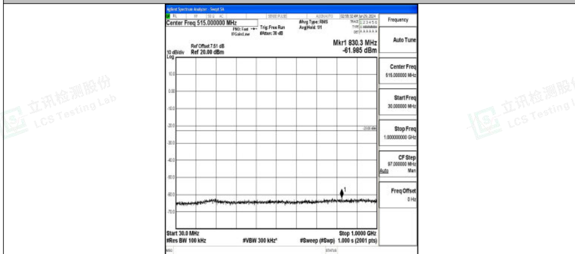
Band4_20MHz_QPSK_20175_1RB#0_30~1000_30~1000
