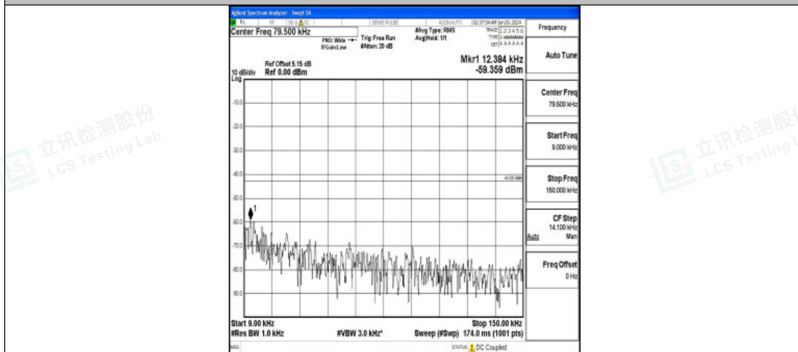
Band4_15MHz_QPSK_20025_1RB#0_0.009~0.15_0.009~0.15
