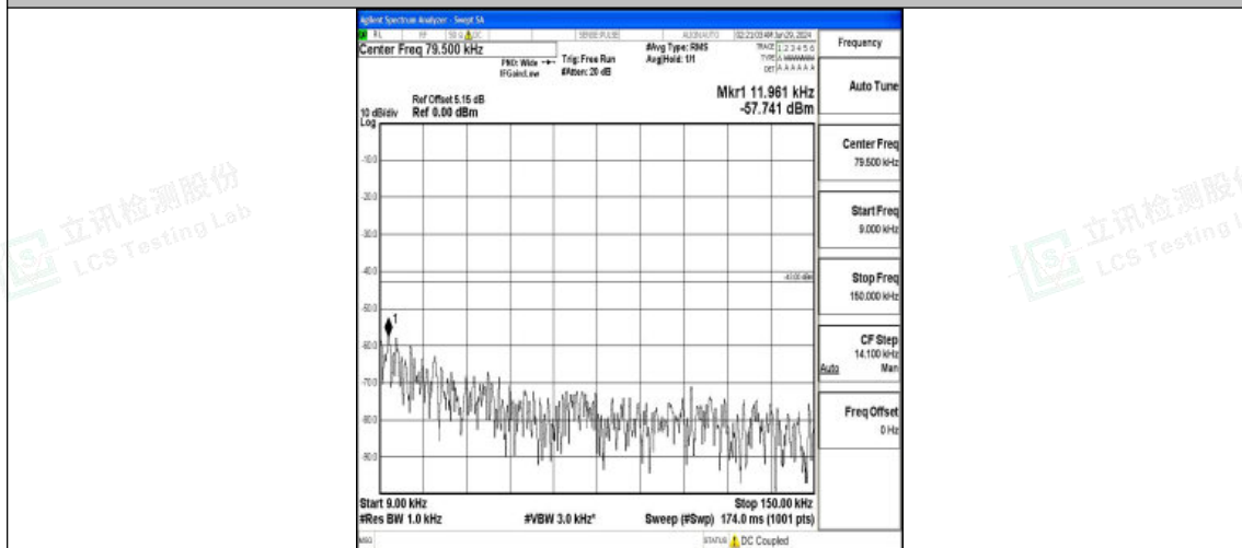
Band4_10MHz_QPSK_20000_1RB#0_0.009~0.15_0.009~0.15
