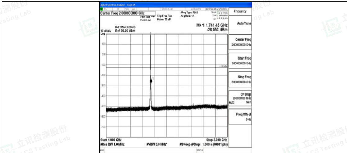
Band4_3MHz_QPSK_20175_1RB#0_1000~3000_1000~3000
