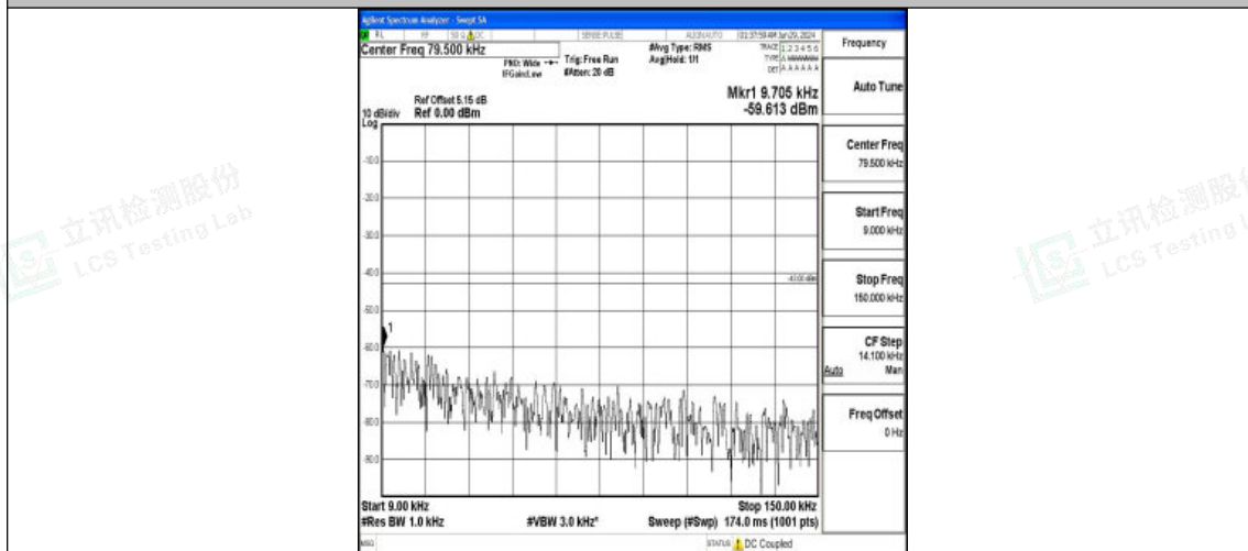
Band4_3MHz_16QAM_20175_1RB#0_0.009~0.15_0.009~0.15
