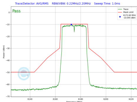
Plot 7-990. SP In-Band Emission Plot Antenna WF7b (20MHz 802.11ax (UNII Band 5) – Ch. 45, MCS4)
