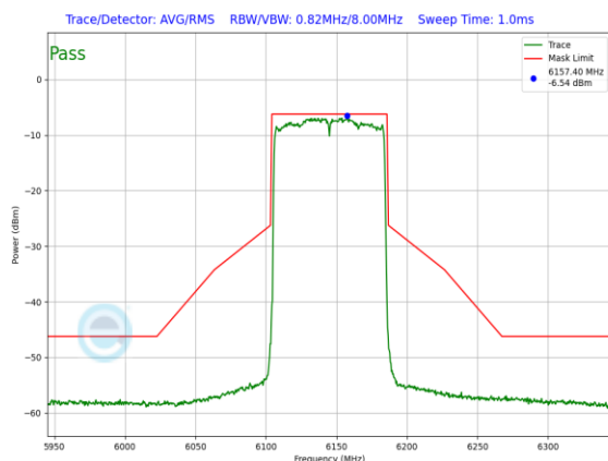
Plot 7-1016. LPI In-Band Emission Plot SDM Primary Antenna WF2a (80MHz 802.11ax (UNII Band 5) – Ch. 39, MCS2)
