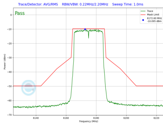
Plot 7-902. SP In-Band Emission Plot Antenna WF2a (20MHz 802.11ax (UNII Band 5) – Ch. 45, MCS4)
