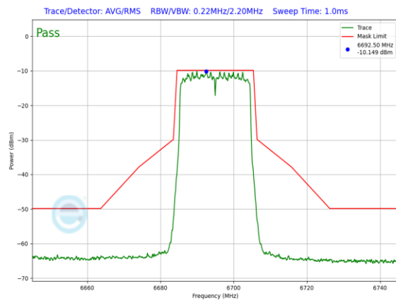
Plot 7-878. LPI In-Band Emission Plot Antenna WF2a (20MHz 802.11ax (UNII Band 7) – Ch. 149, MCS11)
