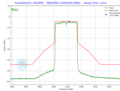
Plot 7-981. SP In-Band Emission Plot Antenna WF7b (80MHz 802.11ax (UNII Band 5) – Ch. 39, MCS2)
