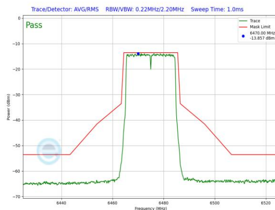
Plot 7-1020. LPI In-Band Emission Plot SDM Primary Antenna WF2a (20MHz 802.11ax (UNII Band 6) – Ch. 105, MCS2)
