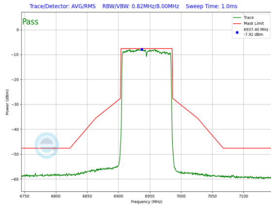
Plot 7-1039. LPI In-Band Emission Plot SDM Primary Antenna WF7a (80MHz 802.11ax (UNII Band 8) – Ch. 199, MCS2)
