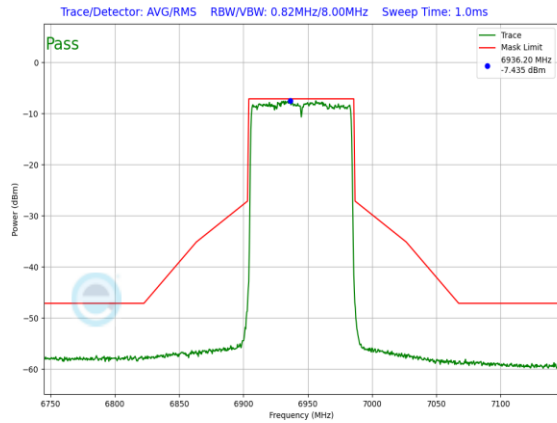
Plot 7-1040. LPI In-Band Emission Plot SDM Primary Antenna WF2a (80MHz 802.11ax (UNII Band 8) – Ch. 199, MCS2)
