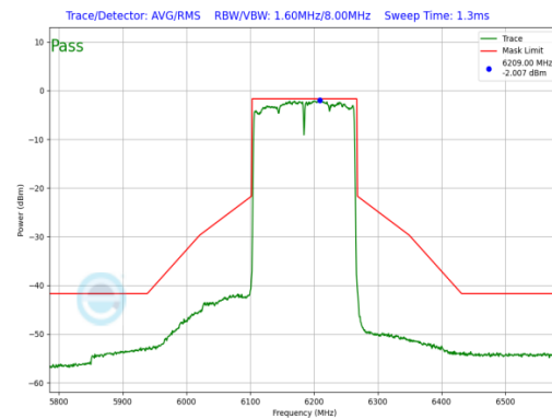
Plot 7-982. SP In-Band Emission Plot Antenna WF7b (160MHz 802.11ax (UNII Band 5) – Ch. 47, MCS2)
