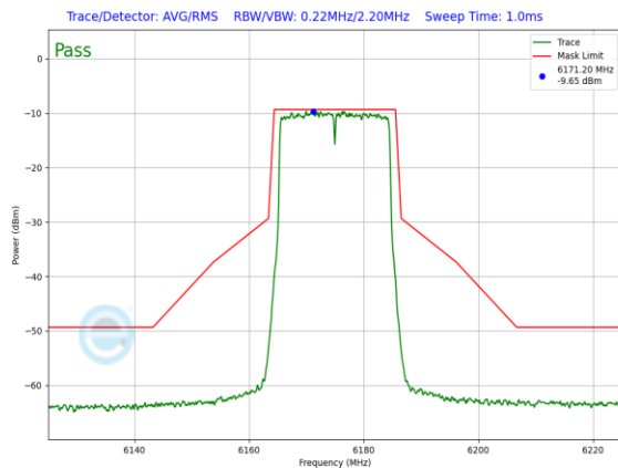
Plot 7-920. LPI In-Band Emission Plot Antenna WF7b (20MHz 802.11ax (UNII Band 5) – Ch. 45, MCS2)
