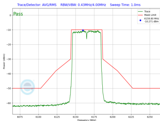
Plot 7-1045. LPI In-Band Emission Plot SDM Primary Antenna WF7a (40MHz 802.11ax (UNII Band 5) – Ch. 43, MCS4)
