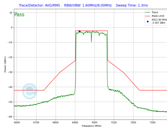
Plot 7-890. LPI In-Band Emission Plot Antenna WF2a (160MHz 802.11ax (UNII Band 8) – Ch. 207, MCS11)
