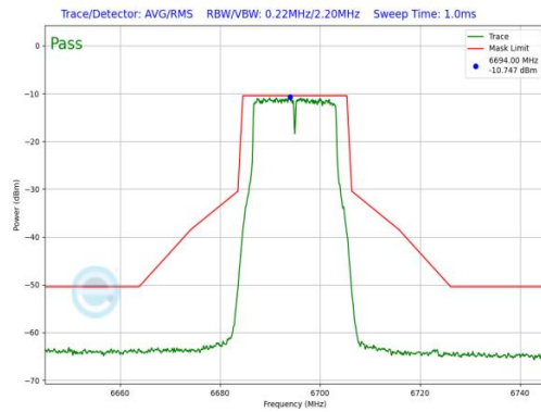
Plot 7-905. SP In-Band Emission Plot Antenna WF2a (20MHz 802.11a (UNII Band 7) – Ch. 149, 24Mbps)
