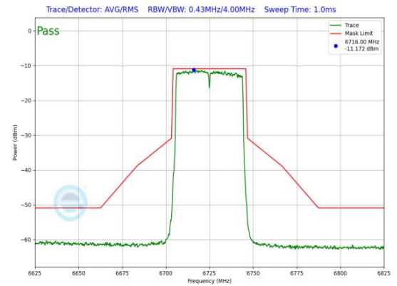
Plot 7-1030. LPI In-Band Emission Plot SDM Primary Antenna WF2a (40MHz 802.11ax (UNII Band 7) – Ch. 155, MCS2)
