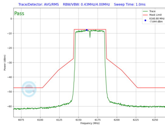
Plot 7-984. SP In-Band Emission Plot Antenna WF7b (40MHz 802.11ax (UNII Band 5) – Ch. 43, MCS2)
