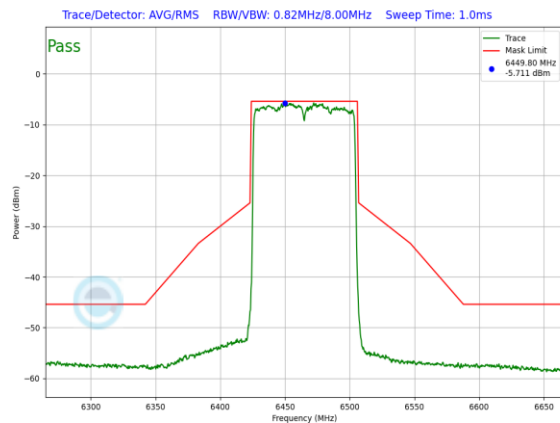
Plot 7-947. LPI In-Band Emission Plot Antenna WF7b (80MHz) 802.11ax (UNII Band 6) – Ch. 103, MCS4)
