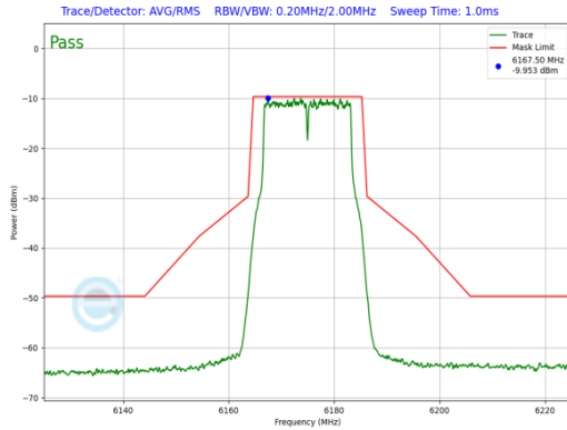
Plot 7-1001. SP In-Band Emission Plot Antenna WF7b (20MHz) 802.11a (UNII Band 5) – Ch. 45, 54Mbps)
