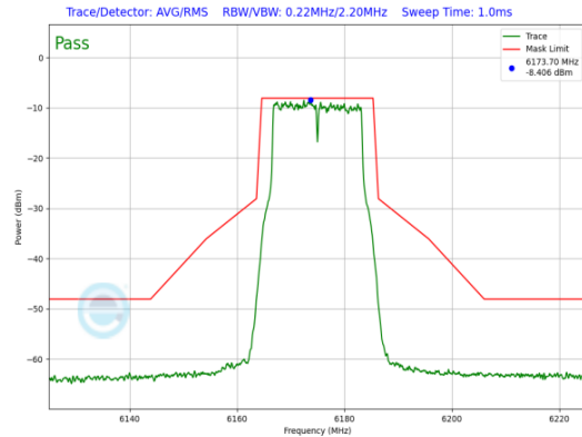
Plot 7-955. LPI In-Band Emission Plot Antenna WF7b (20MHz 802.11a (UNII Band 5) – Ch. 45, 54Mbps)
