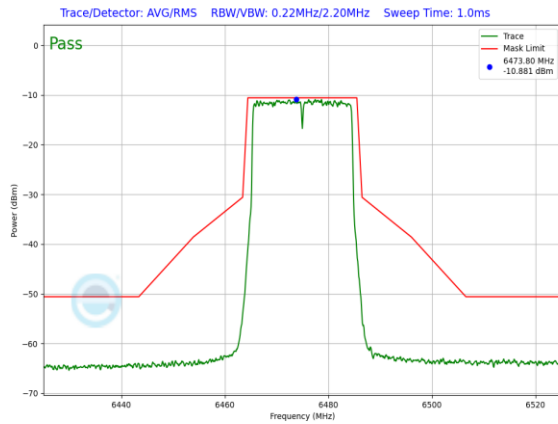
Plot 7-925. LPI In-Band Emission Plot Antenna WF7b (20MHz 802.11ax (UNII Band 6) – Ch. 105, MCS2)
