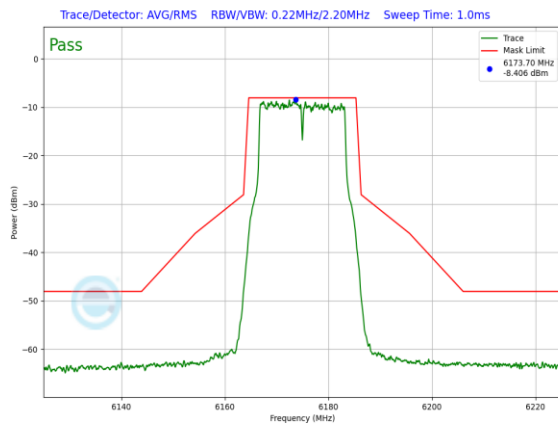
Plot 7-867. LPI In-Band Emission Plot Antenna WF2a (20MHz 802.11a (UNII Band 5) – Ch. 45, 54Mbps)
