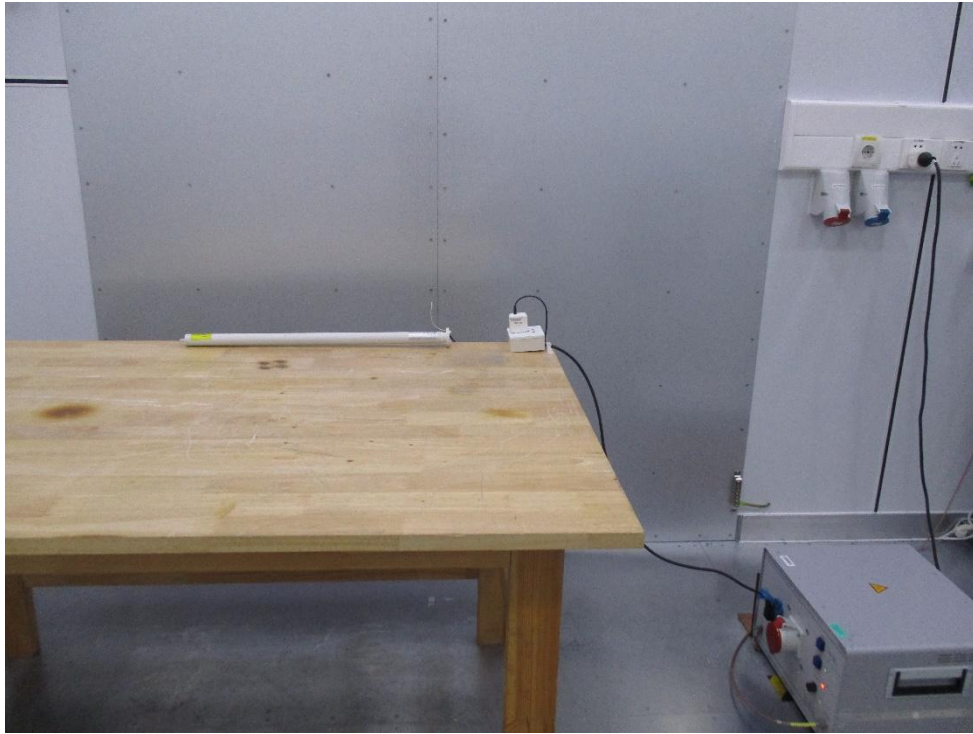
Conduction Emission
