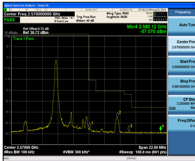
Band7-5MHz-16QAM-21425-1RB#24
