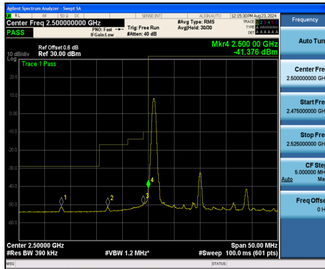
Band7-20MHz-16QAM-20850-27RB#0
