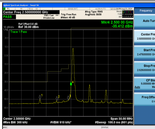
Band7-15MHz-16QAM-20825-27RB#0
