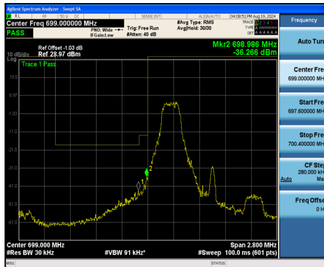
Band12-1.4MHz-QPSK-23017-1RB#5
