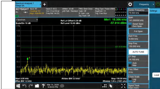
Band13-5MHz-QPSK-23255-1RB#0-0.009~0.15-PASS
