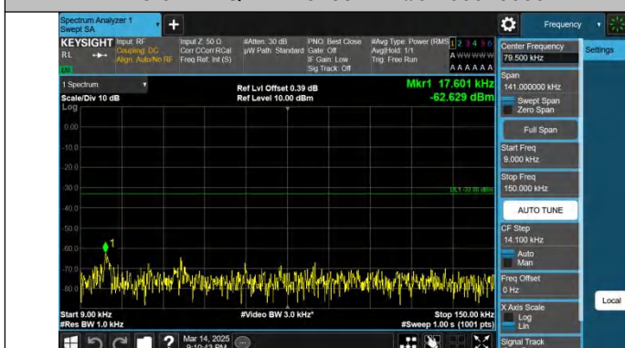
Band13-5MHz-QPSK-23255-1RB#24-0.009~0.15-PASS
