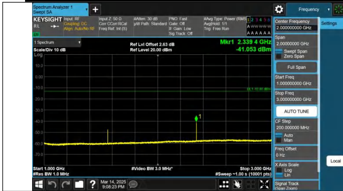
Band13-5MHz-QPSK-23230-1RB#0-1000~3000-PASS
