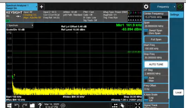
Band13-10MHz-QPSK-23230-1RB#0-0.15~30-PASS
