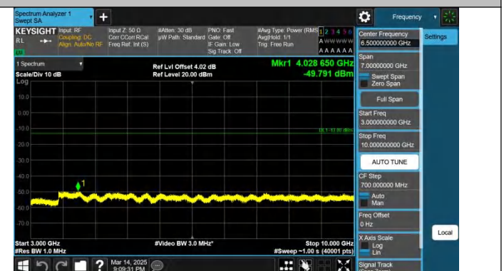
Band13-5MHz-QPSK-23230-1RB#24-3000~10000-PASS
