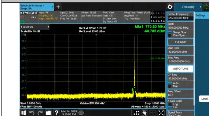
Band13-5MHz-QPSK-23255-1RB#0-30~1000-PASS
