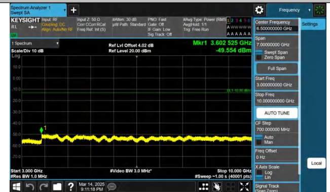
Band13-5MHz-QPSK-23255-1RB#24-3000~10000-PASS
