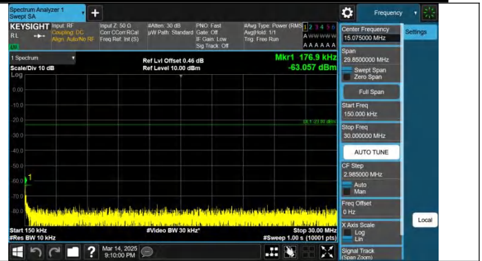
Band13-5MHz-QPSK-23255-1RB#0-0.15~30-PASS
