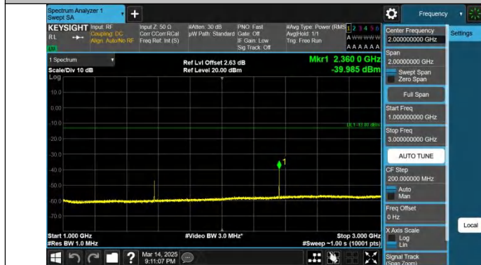
Band13-5MHz-QPSK-23255-1RB#24-1000~3000-PASS
