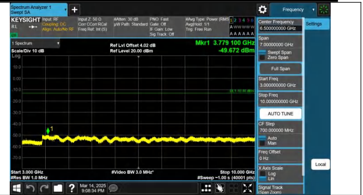
Band13-5MHz-QPSK-23230-1RB#0-3000~10000-PASS
