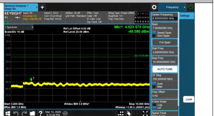
Band13-5MHz-QPSK-23255-1RB#0-3000~10000-PASS
