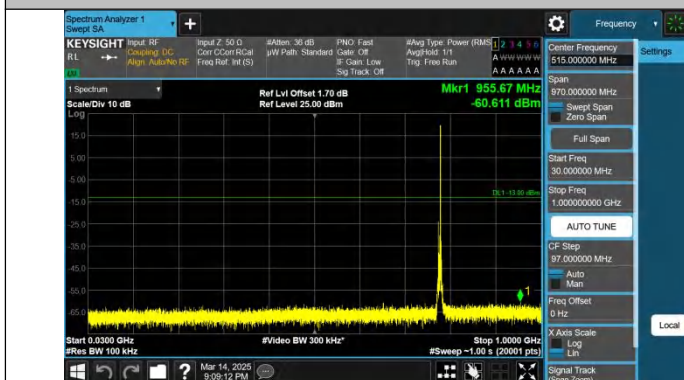
Band13-5MHz-QPSK-23230-1RB#24-30~1000-PASS
