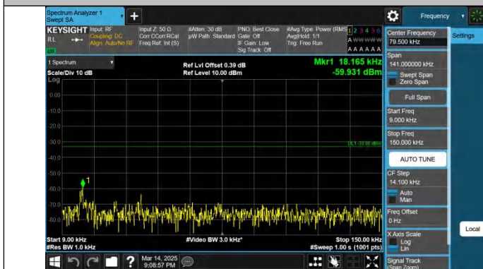
Band13-5MHz-QPSK-23230-1RB#24-0.009~0.15-PASS
