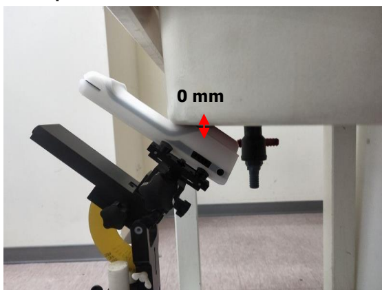
Fig.5 EUT Back (curve) side to flat phantom
