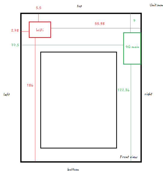
Fig.19 Antenna position of EUT
