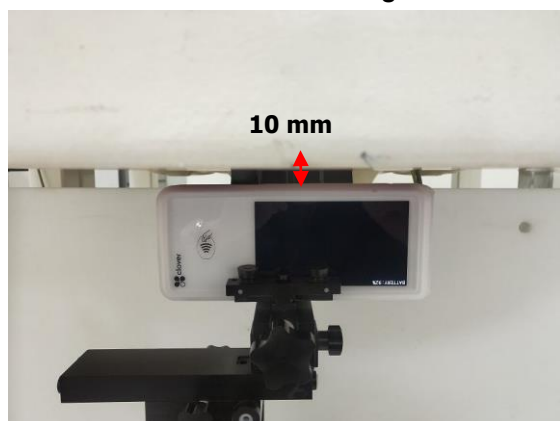
Fig.15 EUT Right side to flat phantom
