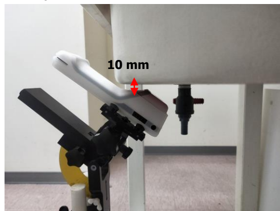
Fig.12 EUT Back (curve) side to flat phantom
