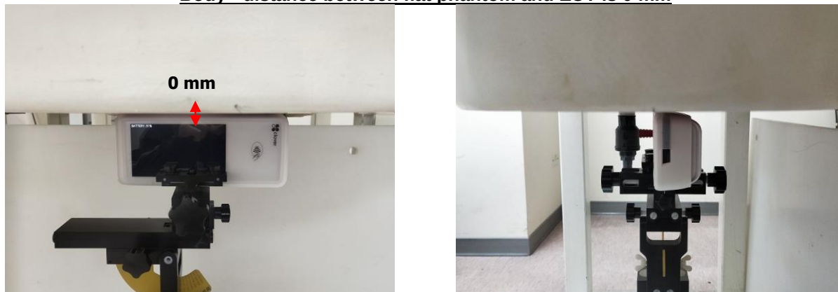
Fig.9 EUT Left side to flat phantom
