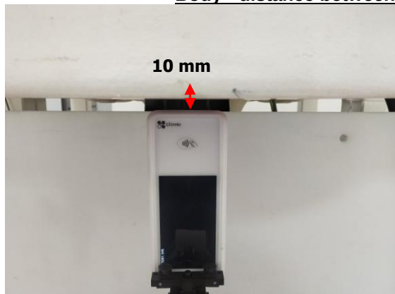
Fig.13 EUT Top side to flat phantom
