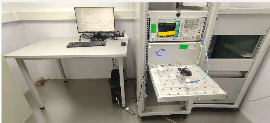
Conducted Test
