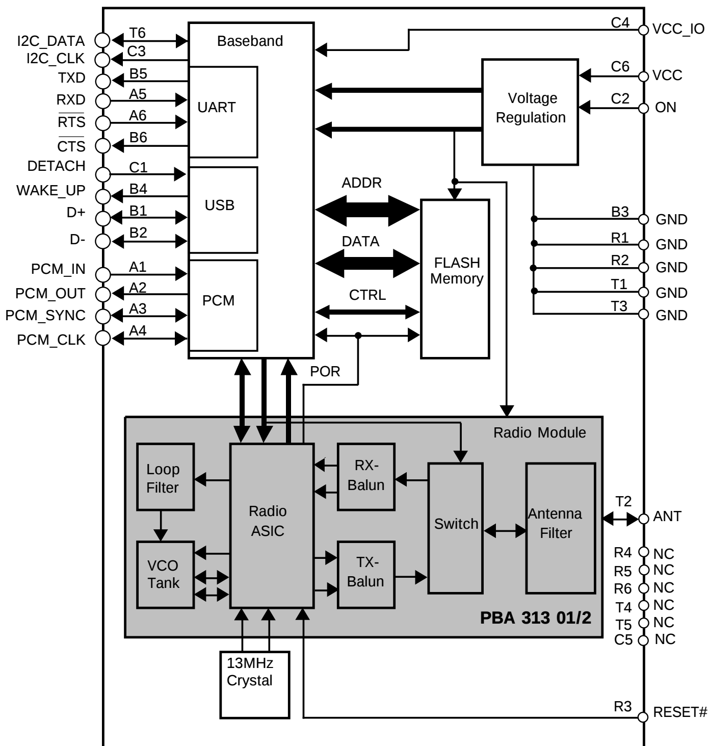
Block diagram for Ericsson Bluetooth modules Rok 101 002/1 Radio set used in Rok 101 007
