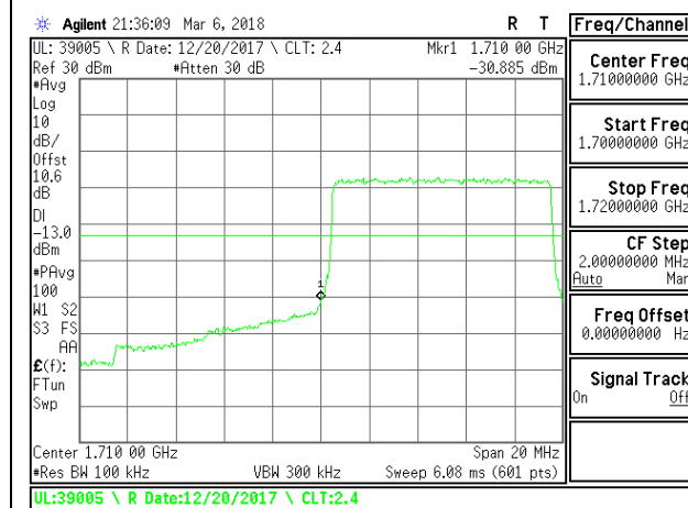
LTE B4 10MHz QPSK Low Channel RB50-0
