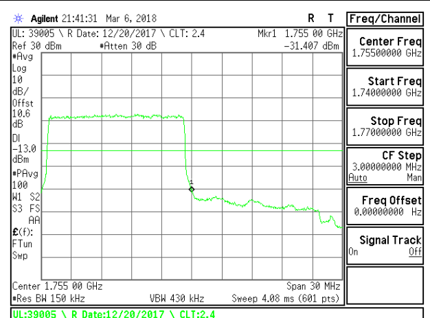
LTE B4 15MHz QPSK High Channel RB75-0
