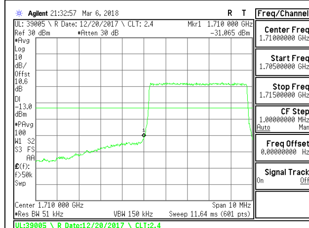
LTE B4 5MHz 16QAM Low Channel RB25-0
