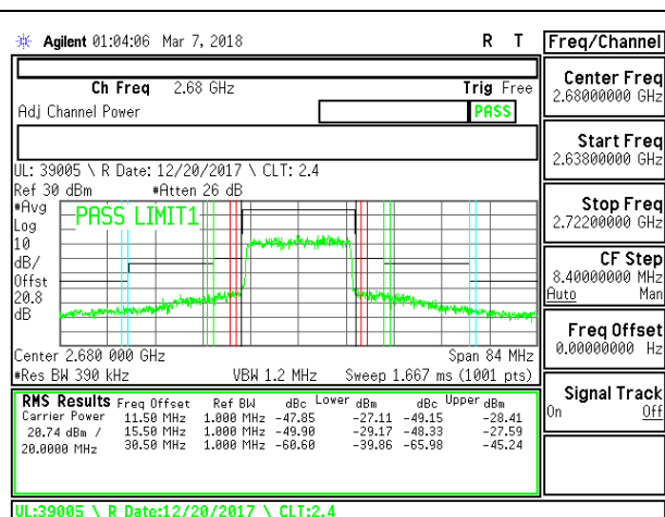
LTE B41 20MHz 16QAM High Channel RB100-0
