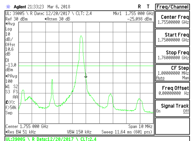
LTE B4 5MHz QPSK High Channel RB1-24
