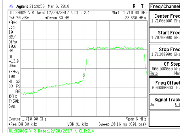
LTE B4 3MHz 16QAM Low Channel RB15-0
