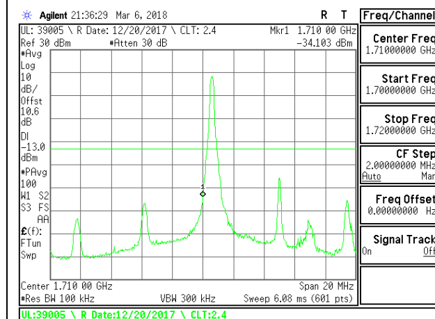
LTE B4 10MHz 16QAM Low Channel RB1-0
