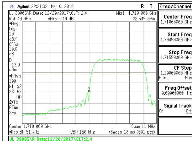
WCDMA Band 4 Rel 99 Low Channel
