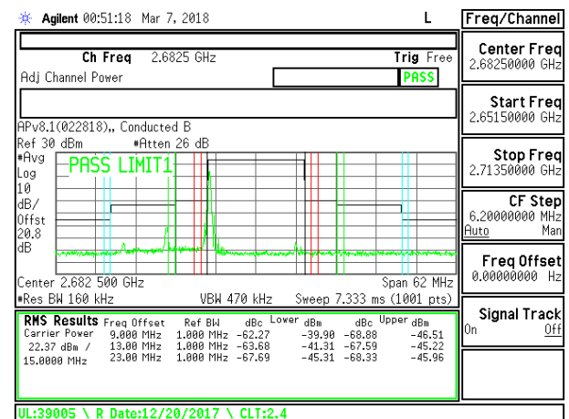
LTE B41 15MHz QPSK High Channel RB1-74
