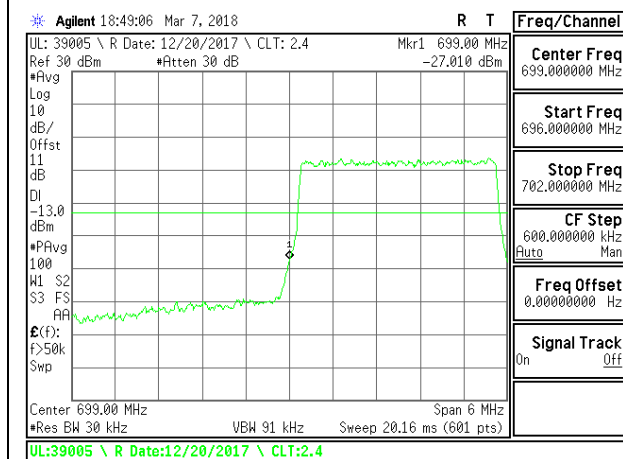
LTE B12 3MHz 16QAM Low Channel RB15-0
