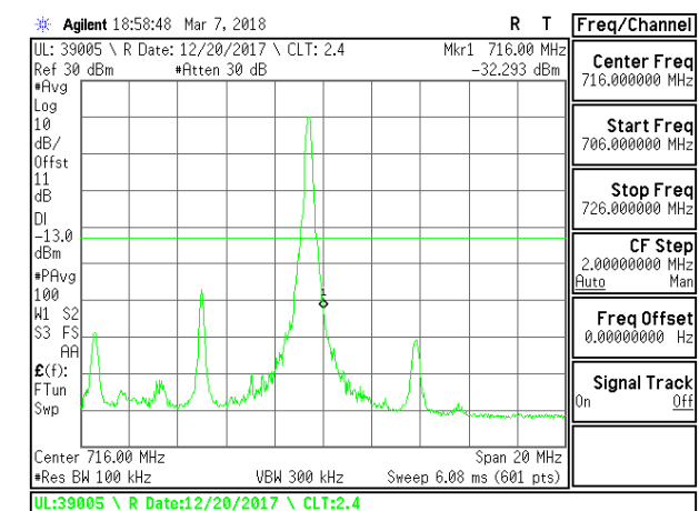
LTE B12 10MHz 16QAM High Channel RB1-49
