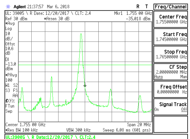
LTE B4 10MHz 16QAM High Channel RB1-49
