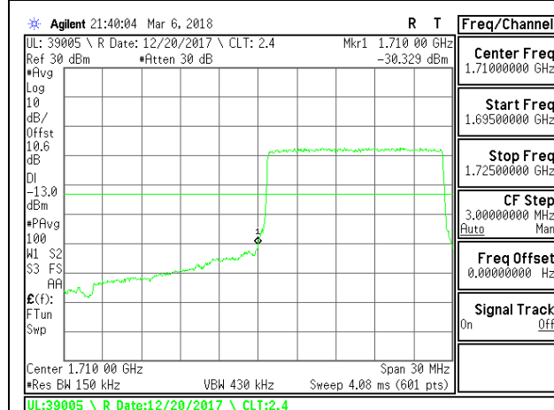
LTE B4 15MHz QPSK Low Channel RB75-0
