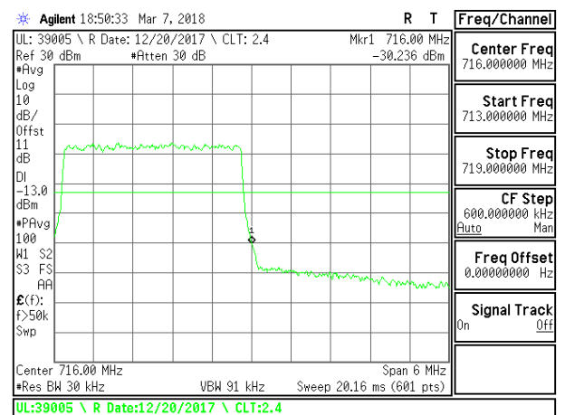
LTE B12 3MHz 16QAM High Channel RB15-0
