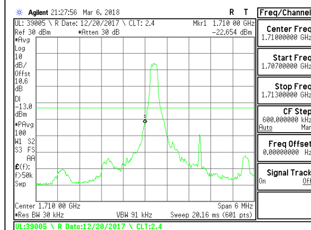
LTE B4 3MHz QPSK Low Channel RB1-0
