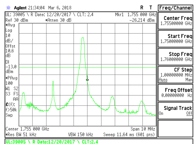
LTE B4 5MHz 16QAM High Channel RB1-24
