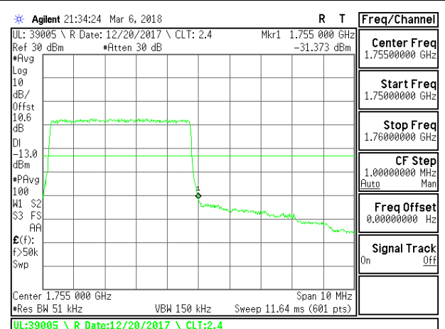
LTE B4 5MHz 16QAM High Channel RB25-0
