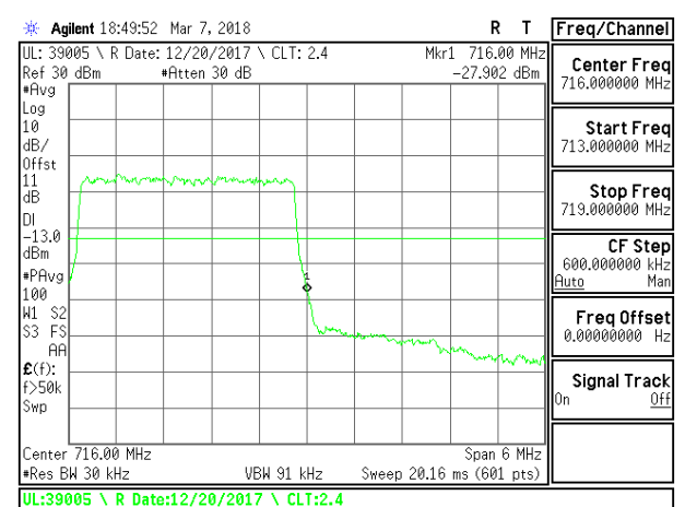
LTE B12 3MHz QPSK High Channel RB15-0
