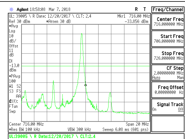
LTE B12 10MHz QPSK High Channel RB1-24
