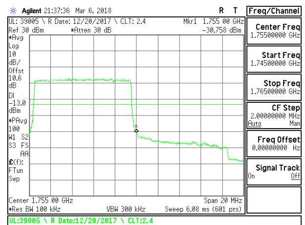
LTE B4 10MHz QPSK High Channel RB50-0
