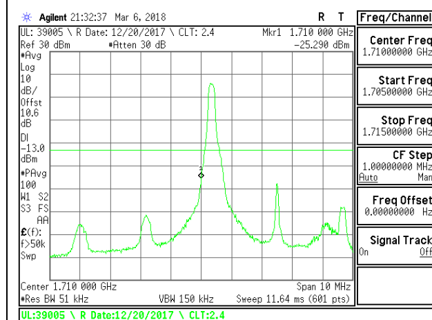
LTE B4 5MHz 16QAM Low Channel RB1-0
