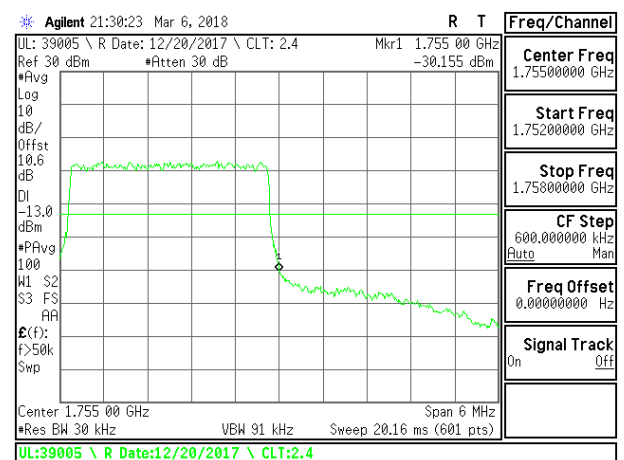
LTE B4 3MHz 16QAM High Channel RB15-0
