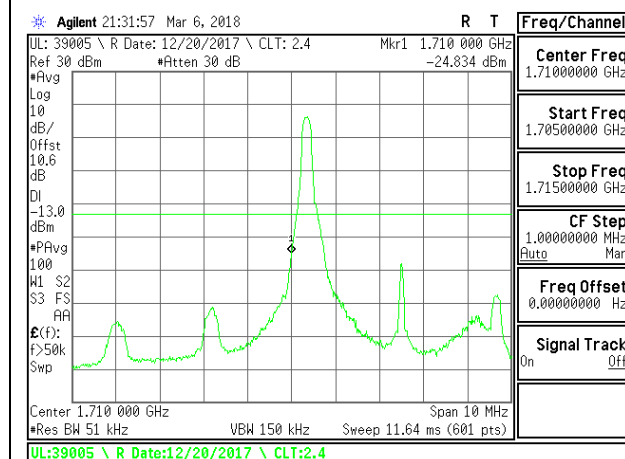
LTE B4 5MHz QPSK Low Channel RB1-0
