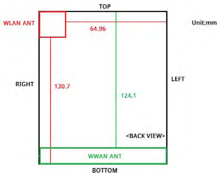
Fig.17 Antenna position of EUT
