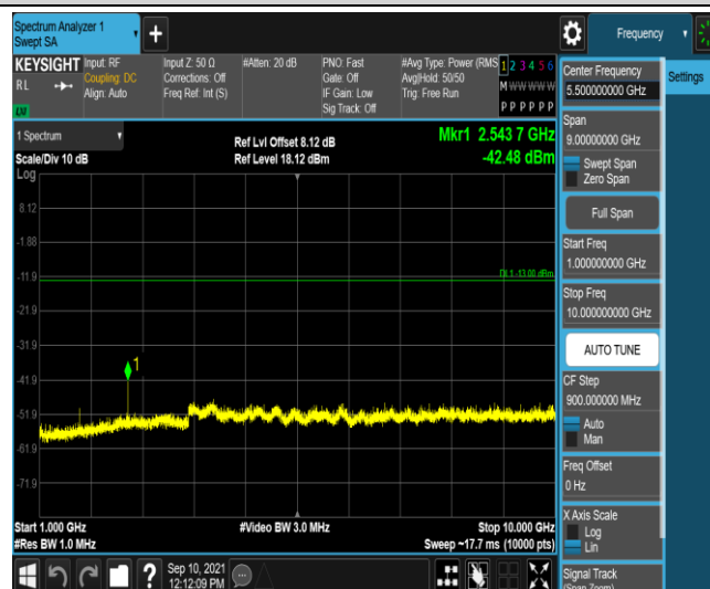
Band5-1.4MHz-QPSK-20643-1RB#0-Range4:1000~10000MHz
