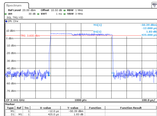
\pi/4 -DQPSK_Hopping_2DH1 0.425ms
