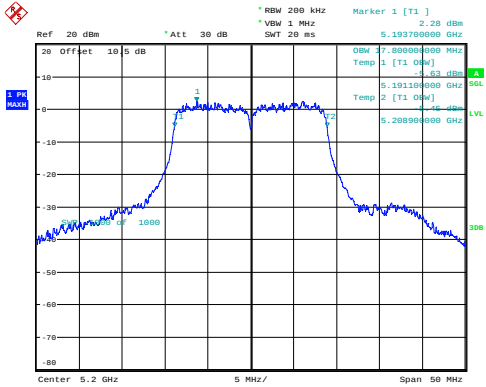
n20_5200MHz_Chain 0 17.800MHz
