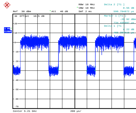
ac80_5210MHz_Chain 0 0.465ms,0.597ms
