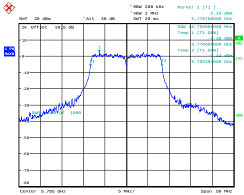
a_5785MHz_Chain 0 16.750MHz
