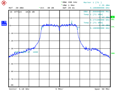
n20_5180MHz_Chain 0 17.800MHz
