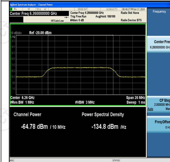
11AX160SISO-Ant2-6185-High-6260-Minimal
