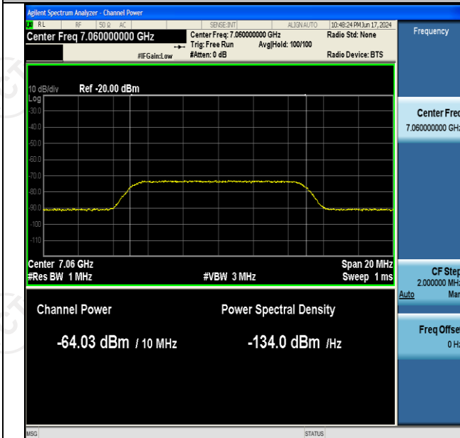
11AX160SISO-Ant2-6985-High-7060-Minimal
