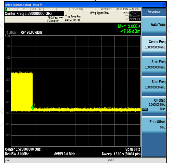
11AX160SISO-Ant2-6505-High-6580-OFF-PASS
