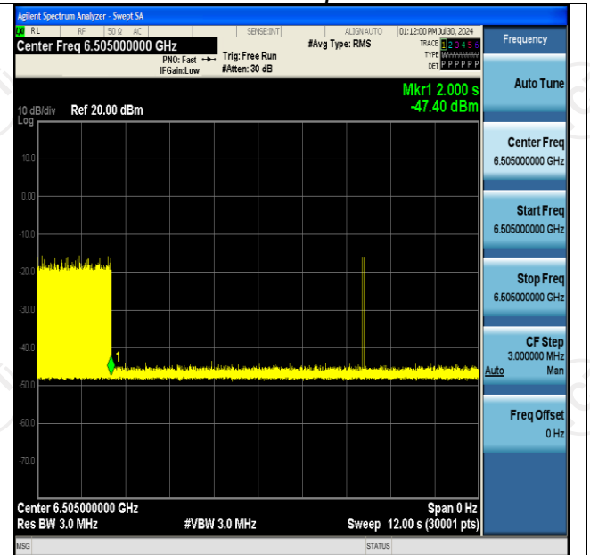
11AX160SISO-Ant2-6505-Center-6505-Minimal
