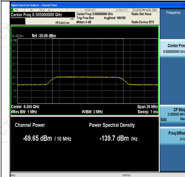
11AX160SISO-Ant2-6505-Center-6505-OFF-PASS
