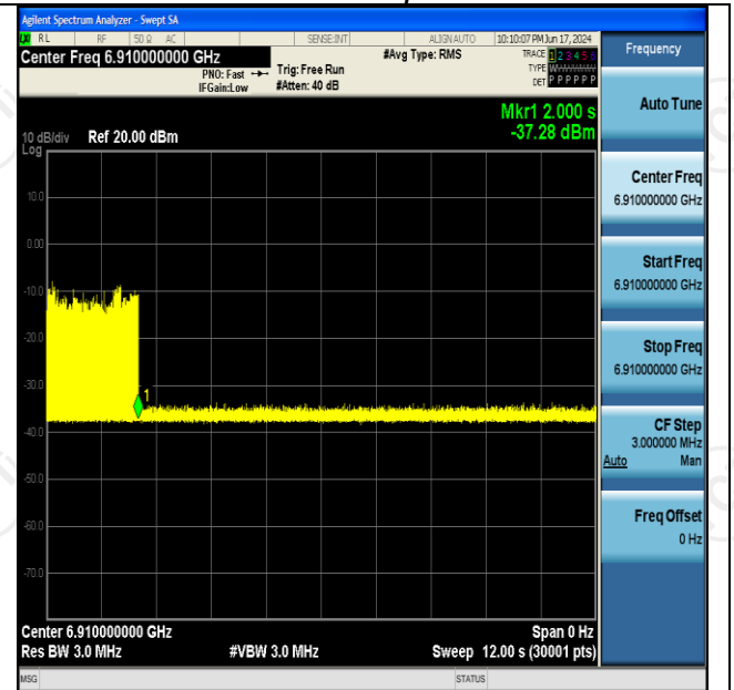
11AX160SISO-Ant2-6985-Low-6910-OFF-PASS
