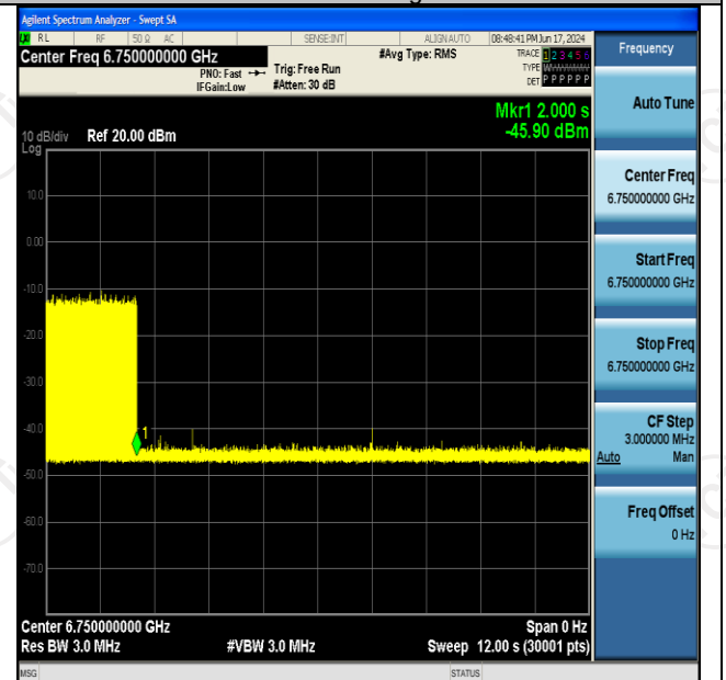
11AX160SISO-Ant2-6825-Low-6750-Minimal
