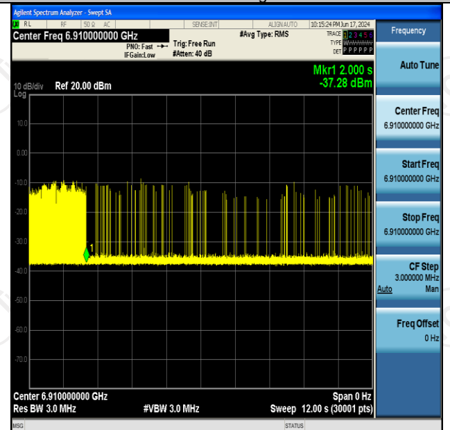
11AX160SISO-Ant2-6985-Low-6910-Minimal
