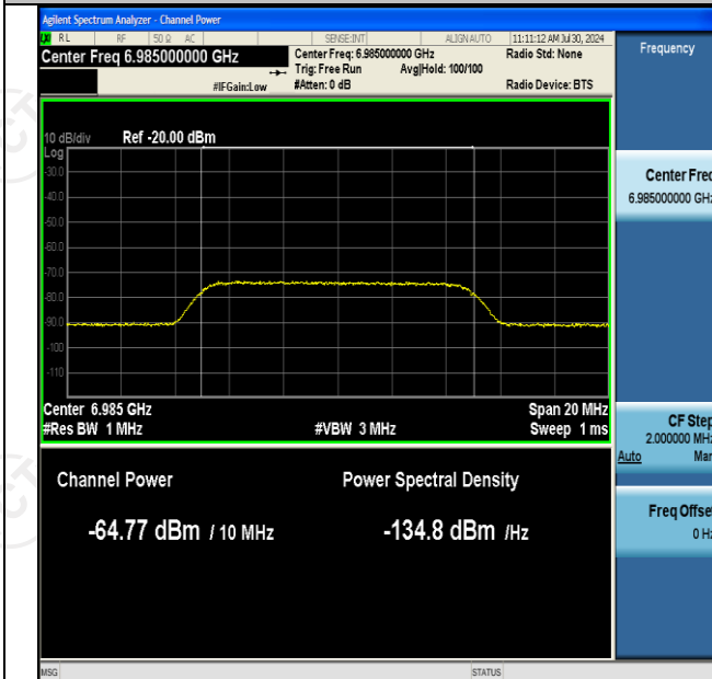
11AX160SISO-Ant2-6985-Center-6985-OFF-PASS
