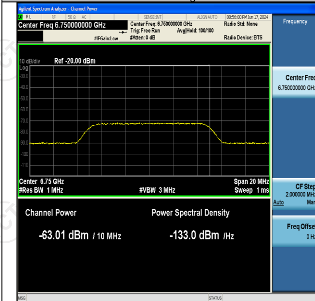
11AX160SISO-Ant2-6825-Low-6750-Minimal
