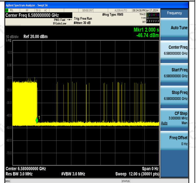
11AX160SISO-Ant2-6505-High-6580-Minimal
