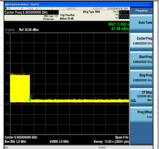
11AX160SISO-Ant2-6985-Center-6985-OFF-PASS
