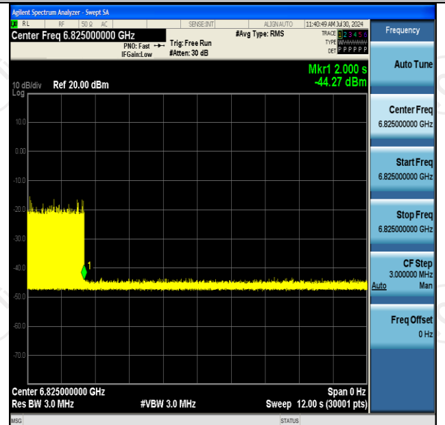
11AX160SISO-Ant2-6825-Center-6825-OFF-PASS
