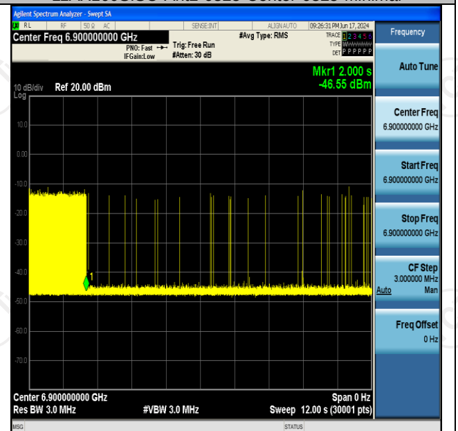
11AX160SISO-Ant2-6825-High-6900-Minimal
