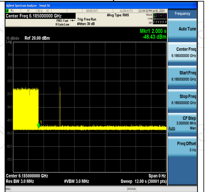
11AX160SISO-Ant2-6185-Center-6185-Minimal
