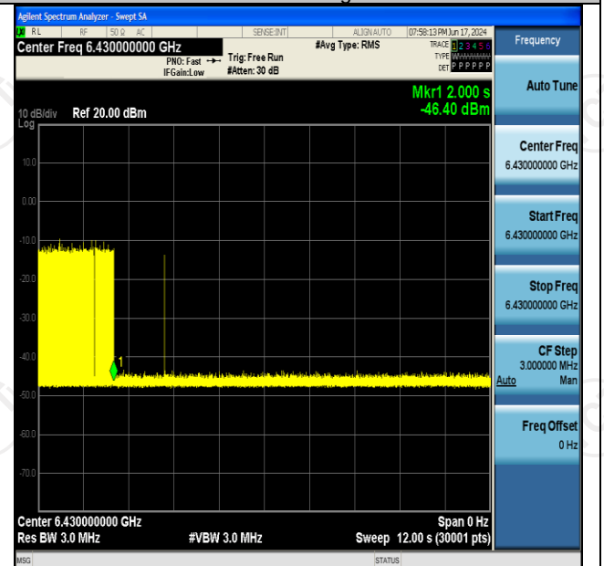
11AX160SISO-Ant2-6505-Low-6430-Minimal
