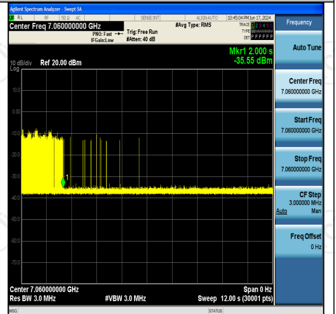
11AX160SISO-Ant2-6985-High-7060-Minimal
