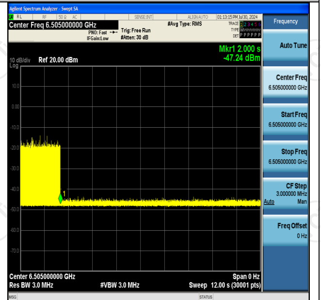
11AX160SISO-Ant2-6505-Center-6505-OFF-PASS
