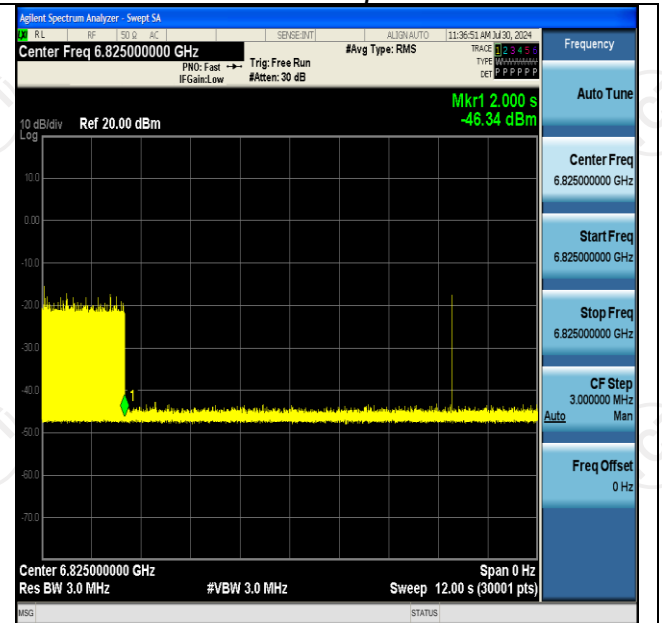
11AX160SISO-Ant2-6825-Center-6825-Minimal
