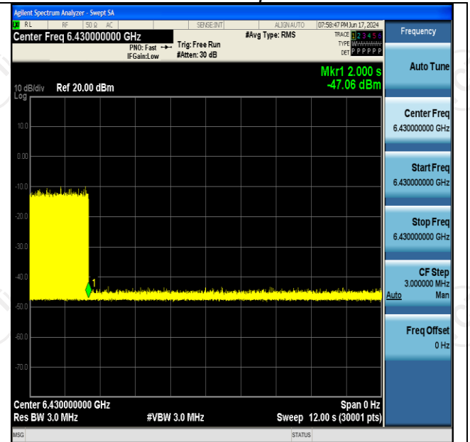
11AX160SISO-Ant2-6505-Low-6430-OFF-PASS
