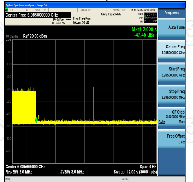
11AX160SISO-Ant2-6985-Center-6985-Minimal
