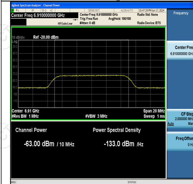
11AX160SISO-Ant2-6985-Low-6910-Minimal
