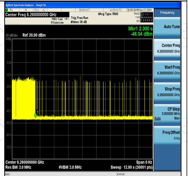
11AX160SISO-Ant2-6185-High-6260-Minimal
