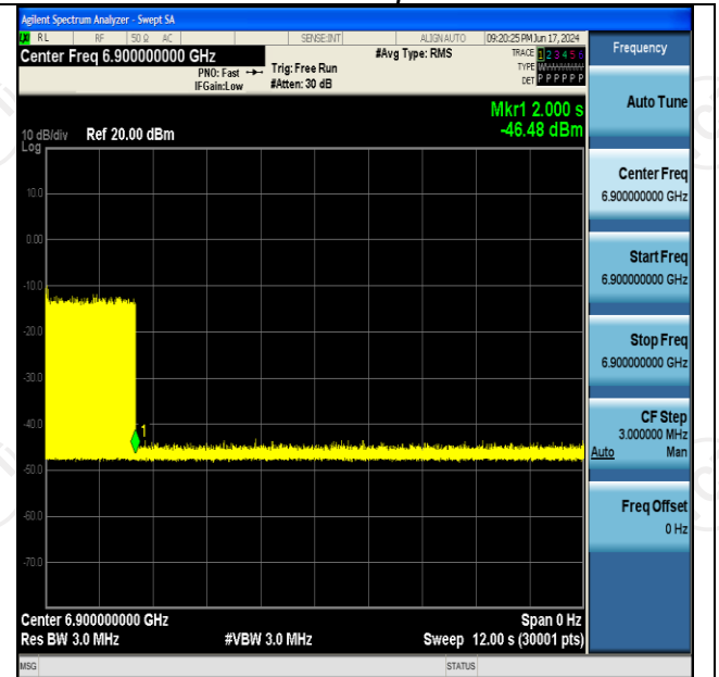
11AX160SISO-Ant2-6825-High-6900-OFF-PASS
