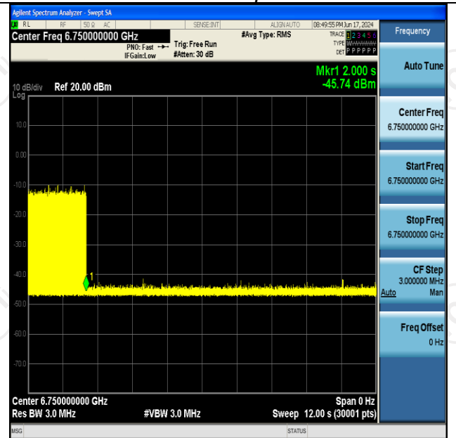
11AX160SISO-Ant2-6825-Low-6750-OFF-PASS
