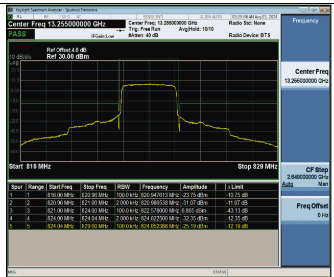
Band26_3MHz_QPSK_26775_15RB#0
