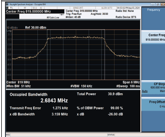
26(814-824)-3MHz-16QAM-26740-15RB#0-PASS
