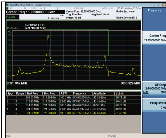
Band26_10MHz_QPSK_26740_1RB#0
