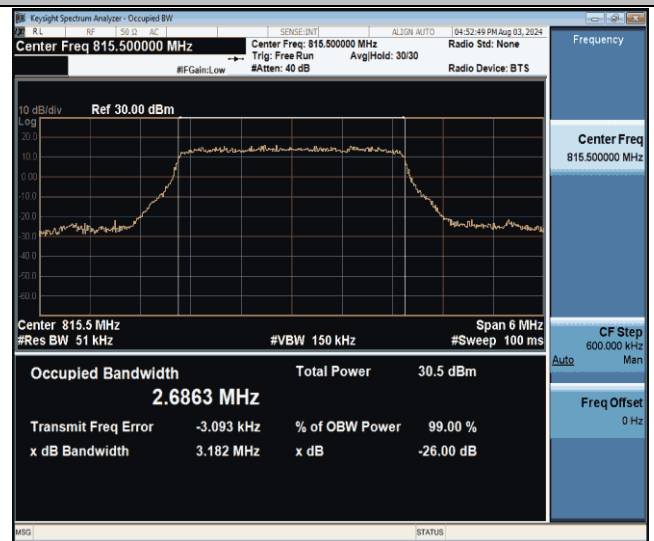
26(814-824)-3MHz-16QAM-26705-15RB#0-PASS
