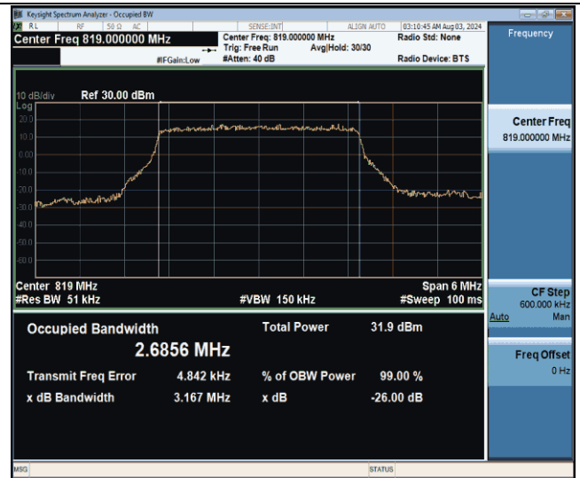
26(814-824)-3MHz-QPSK-26740-15RB#0-PASS
