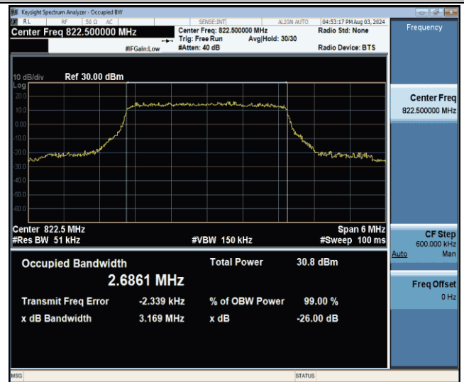
26(814-824)-3MHz-16QAM-26775-15RB#0-PASS
