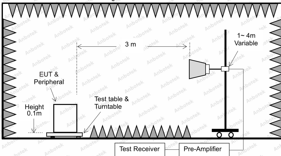
Figure 3. Above 1 GHz
