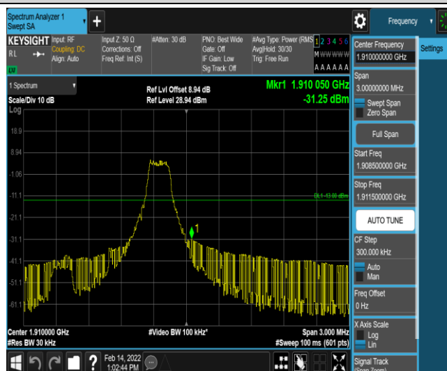
Band2-1.4MHz-16QAM-19193-1-5-High--31.25-PASS
