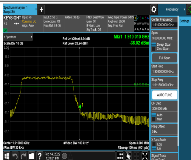
Band2-1.4MHz-16QAM-19193-6-0-High--38.02-PASS
