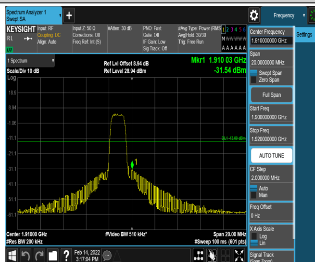
Band2-10MHz-16QAM-19150-6-0-High--31.54-PASS
