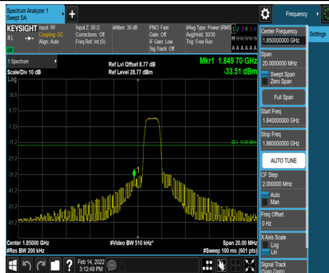
Band2-10MHz-16QAM-18650-6-0-Low--33.51-PASS
