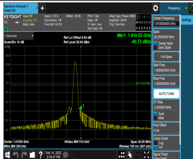
Band2-10MHz-16QAM-19150-1-5-High--40.73-PASS
