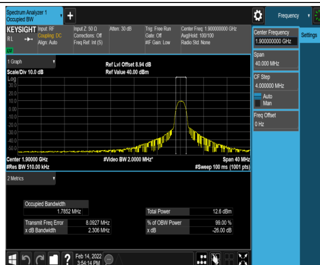
Band2-20MHz-QPSK-19100-6-0-High-1.7852-2.306-PASS
