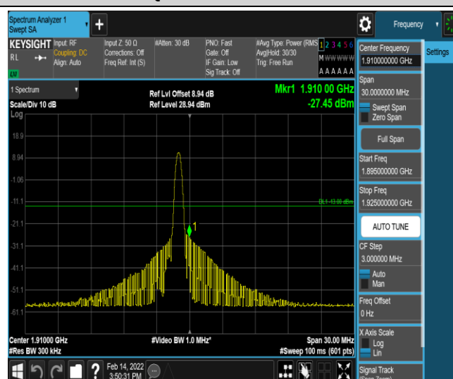
Band2-15MHz-QPSK-19125-1-5-High--27.45-PASS
