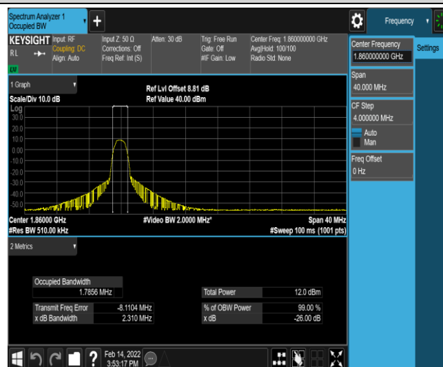
Band2-20MHz-16QAM-18700-6-0-Low-1.7856-2.310-PASS
