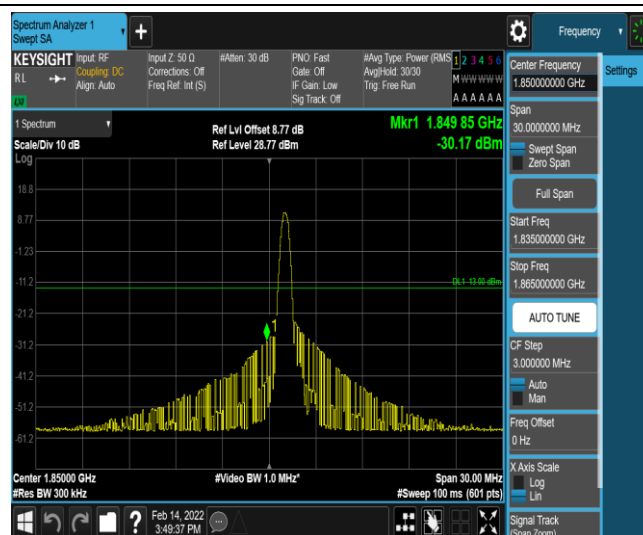
Band2-15MHz-QPSK-18675-1-0-Low--30.17-PASS
