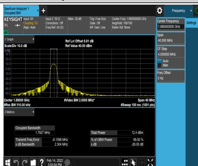
Band2-20MHz-16QAM-18900-6-0-Low-1.7927-2.304-PASS
