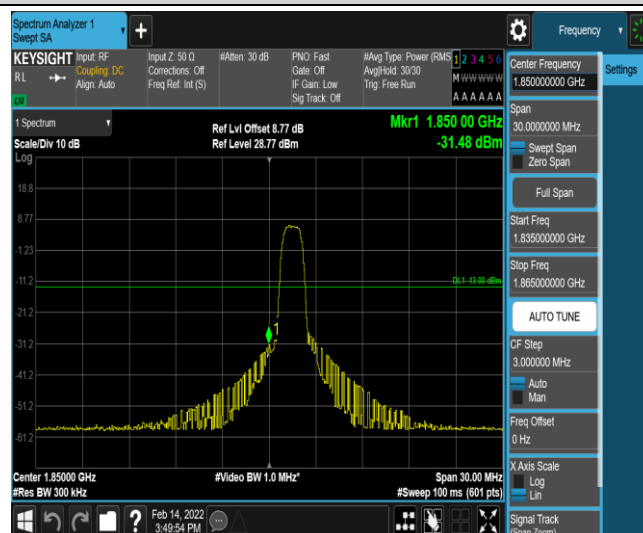
Band2-15MHz-QPSK-18675-6-0-Low--31.48-PASS
