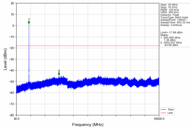
BW 4M_LCH_906MHz_Ant1_NTNV
