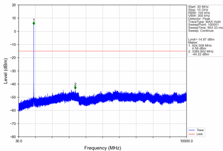
BW 2M_HCH_925MHz_Ant1_NTNV
