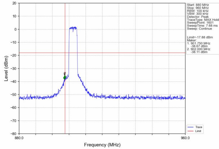
BW 4M_LCH_906MHz_Ant1_NTNV
