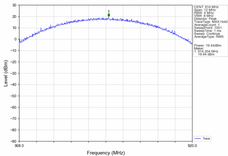
BW 4M_MCH_914MHz_Ant1_NTNV
