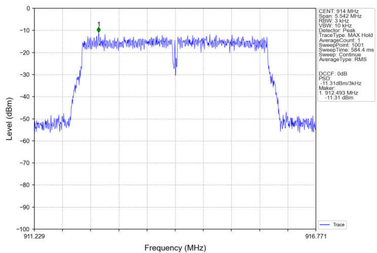
BW 4M_MCH_914MHz_Ant1_NTNV
