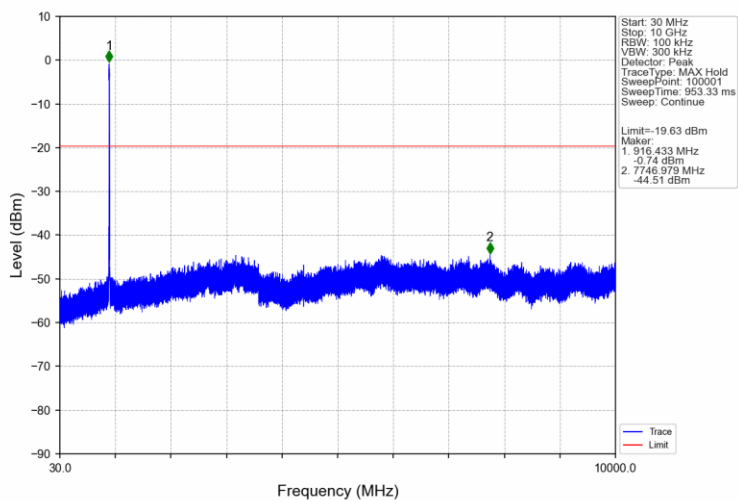
BW 8M_MCH_916MHz_Ant1_NTNV
