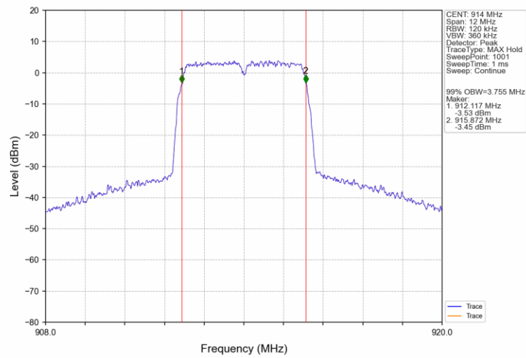
BW 4M_MCH_914MHz_Ant1_NTNV
