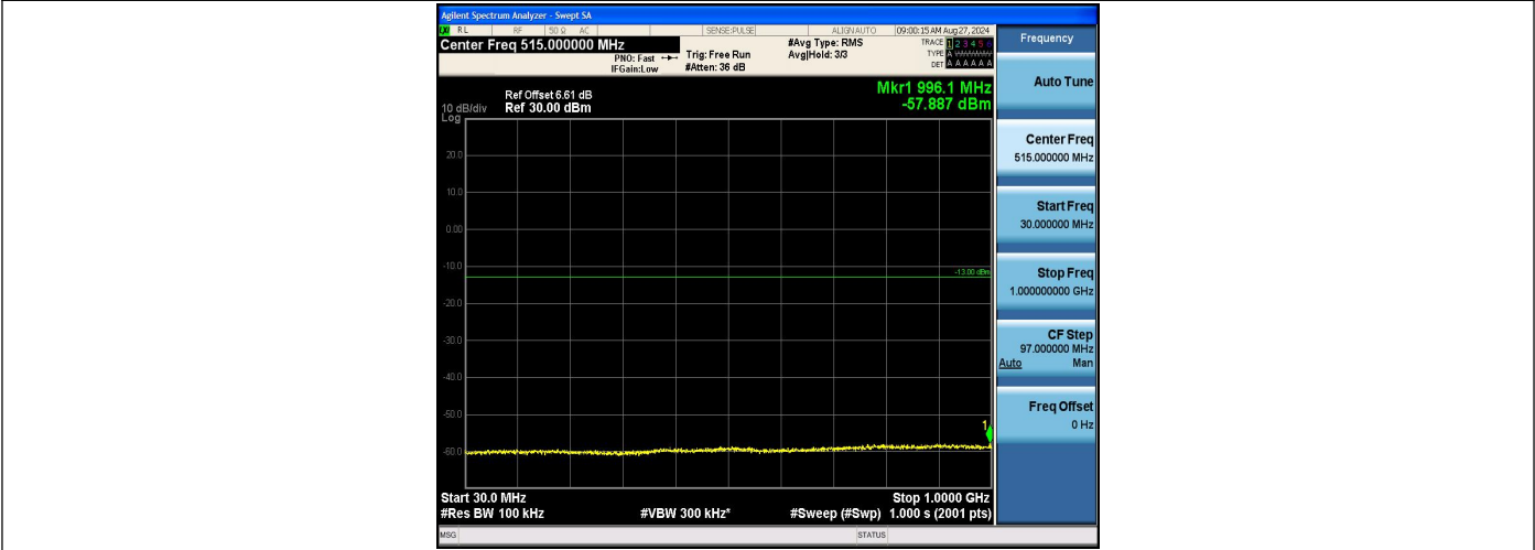
Band2_1.4MHz_16QAM_18607_1RB#0_30~1000_30~1000
