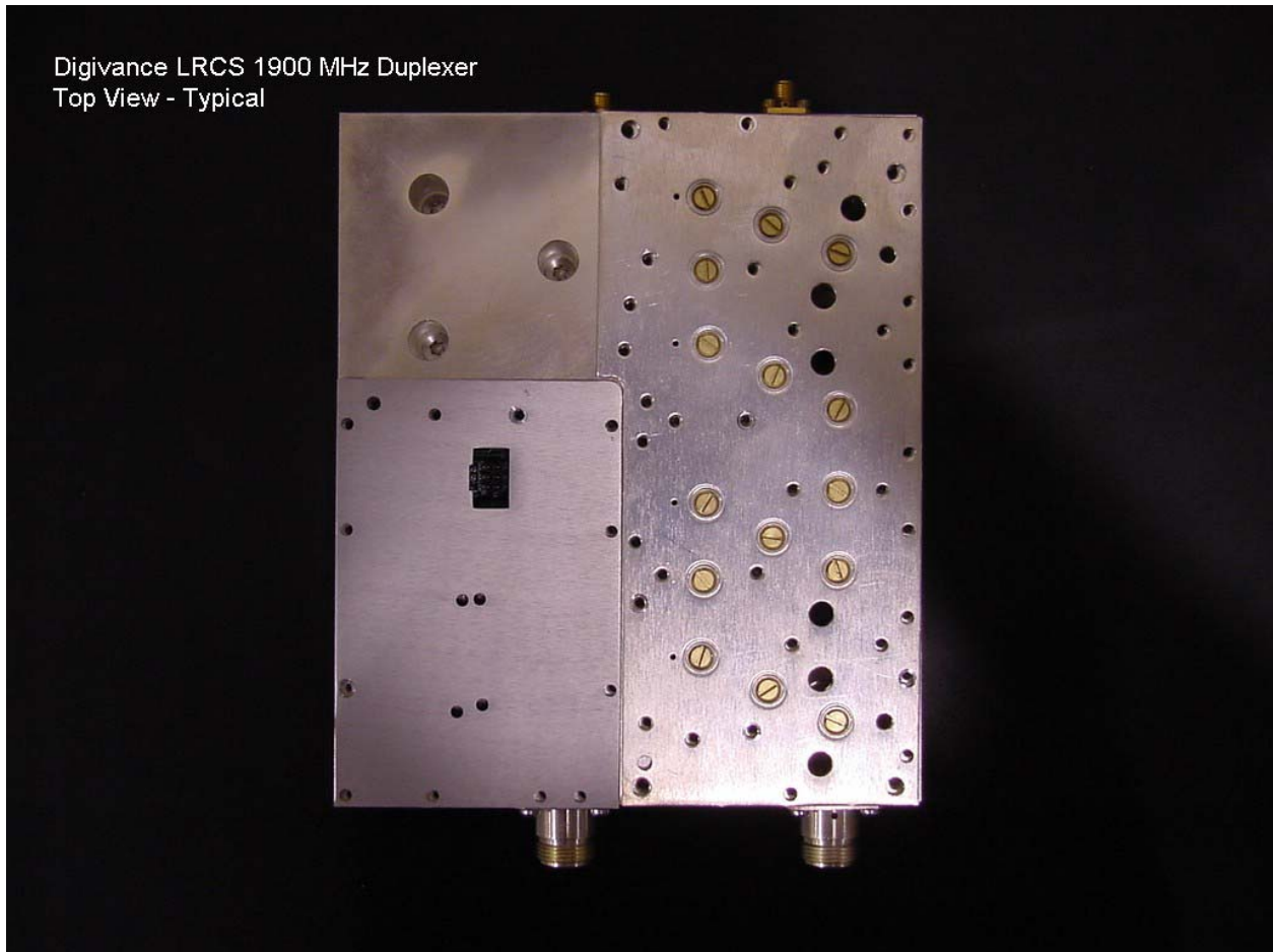
Digivance LRCS 1900 MHz Duplexer Top Open View - Typical
