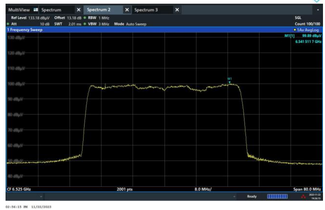
Channel 115 (6525MHz)
