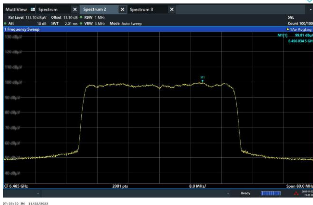
Channel 107 (6485MHz)
