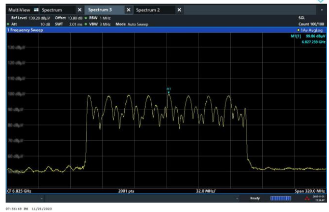
Channel 175 (6825MHz)
