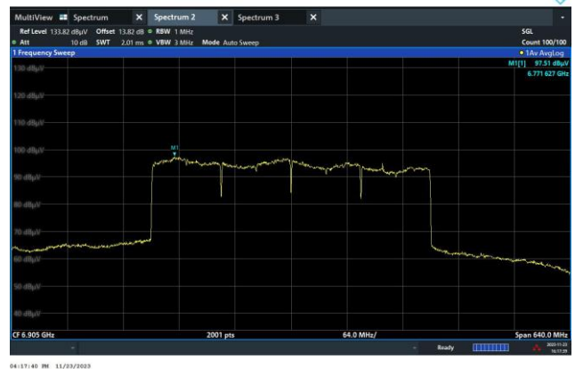
Channel 191 (6905MHz)
