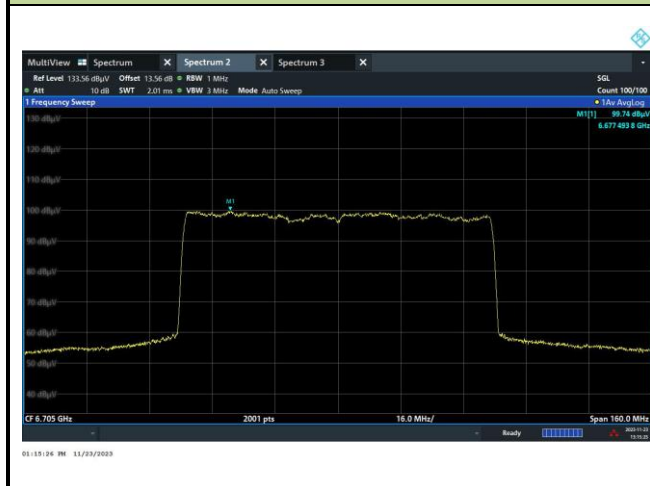
Channel 151 (6705MHz)
