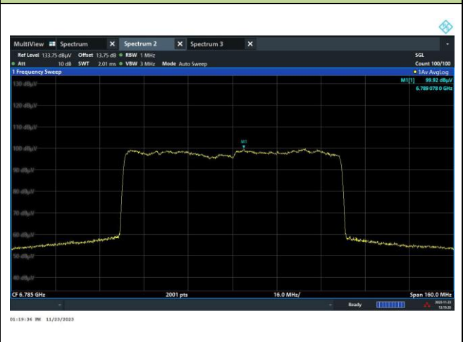
Channel 167 (6785MHz)
