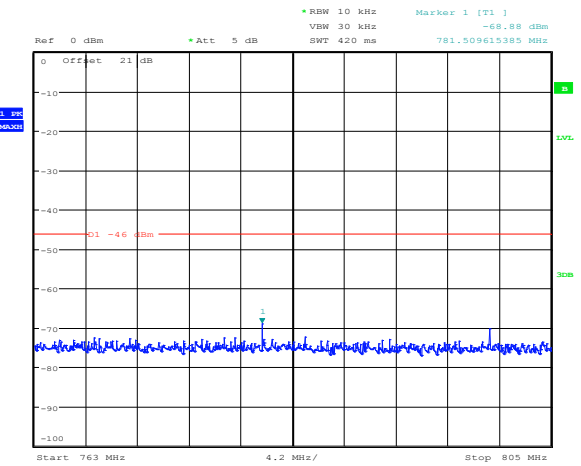
Figure 8.2-10: 1.4 MHz LTE QPSK 763-775 MHz and 793-805 MHz
