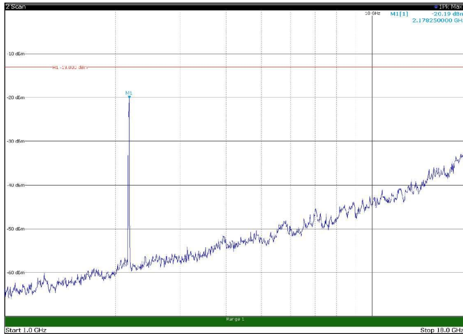
Channel: TOP, Modulation: 256QAM, BW=20MHz, Range: 1GHz - 18GHz, Polarization: Horizontal
