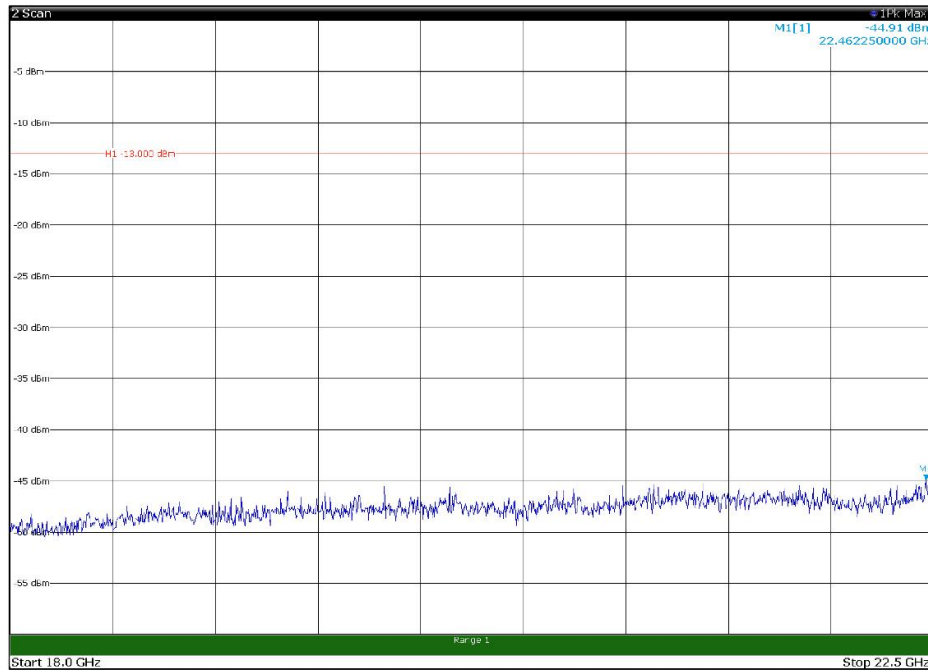
Channel: MIDDLE, Modulation: 256QAM, BW=20MHz, Range: 18GHz - 22.5GHz, Polarization: Horizontal
