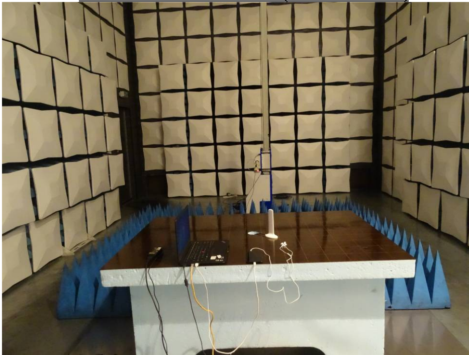
Radiated Disturbance Emissions (26.5GHz to 40GHz)
