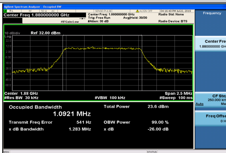
Band2-1.4MHz-16QAM-18900-6RB#0-1.0921
