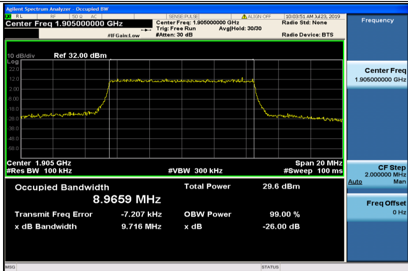
Band2-10MHz-16QAM-19150-50RB#0-8.9659
