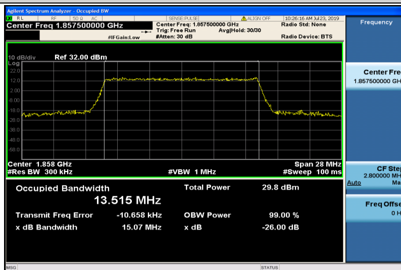
Band2-15MHz-16QAM-18675-75RB#0-13.515
