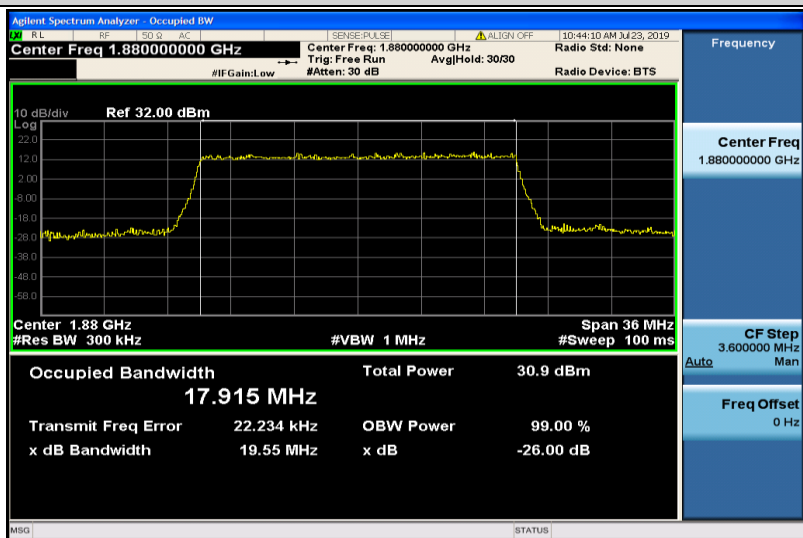
Band2-20MHz-QPSK-18900-100RB#0-17.915
