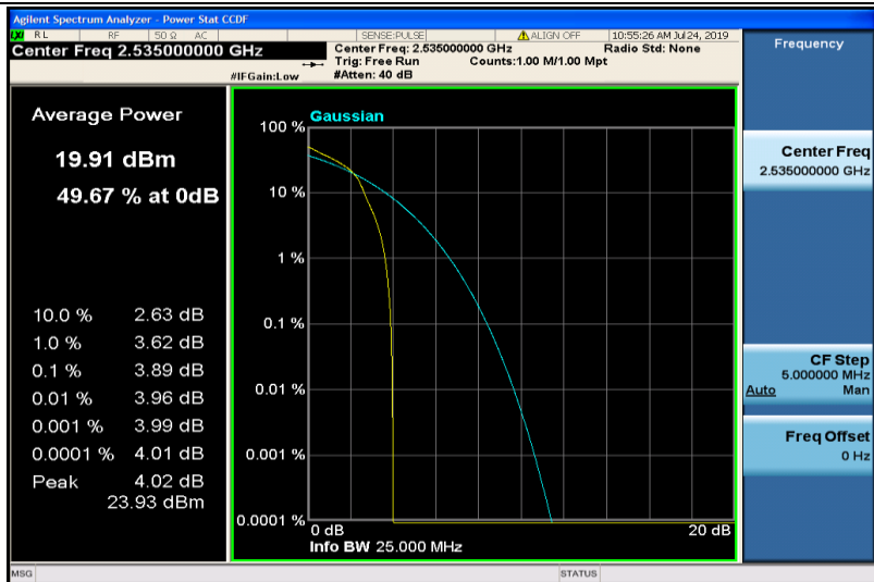
Band7-15MHz-16QAM-21100-1RB#0
