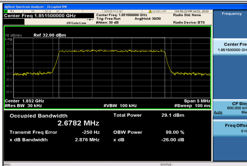
Band2-3MHz-QPSK-18615-15RB#0-2.6782
