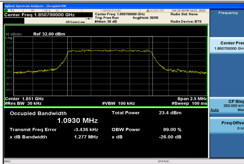
Band2-1.4MHz-QPSK-18607-6RB#0-1.0930
