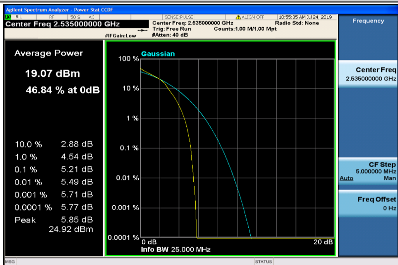
Band7-15MHz-16QAM-21100-75RB#0
