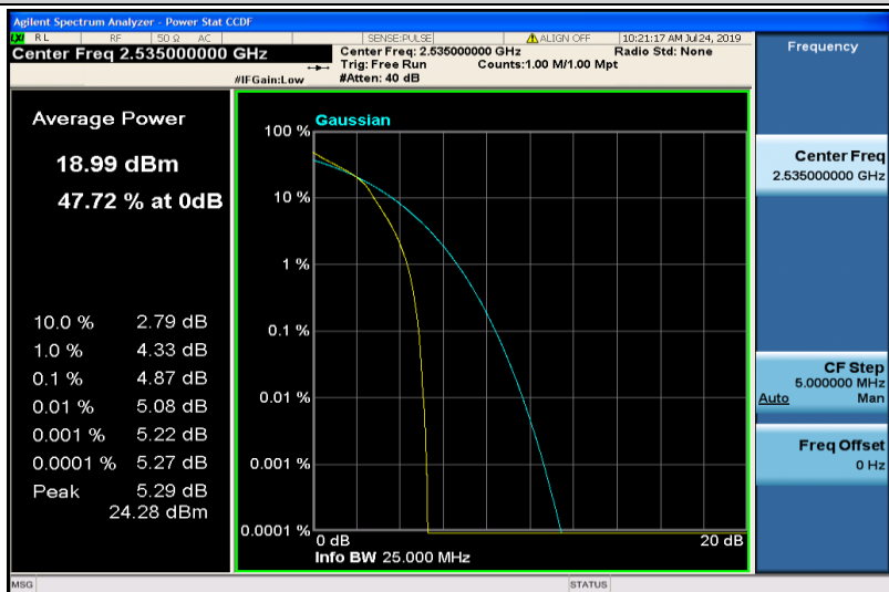
Band7-5MHz-16QAM-21100-25RB#0
