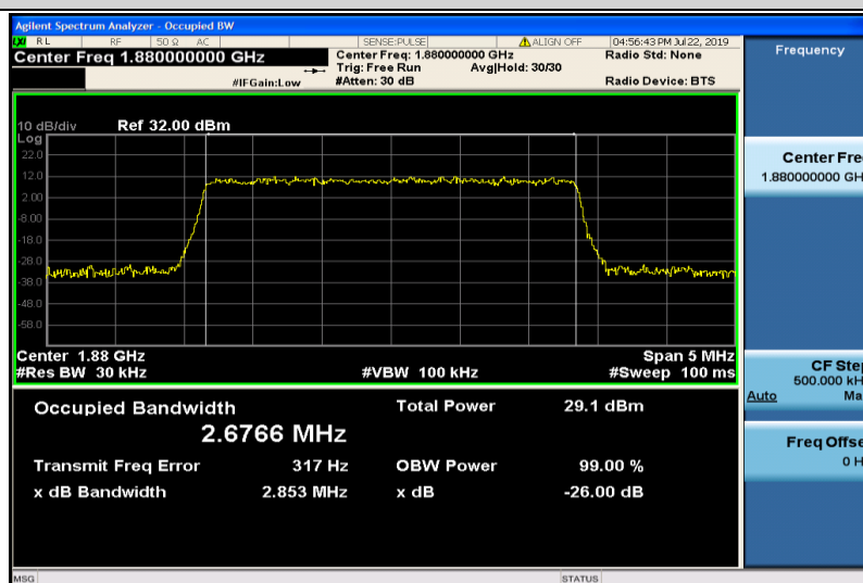
Band2-3MHz-QPSK-18900-15RB#0-2.6766
