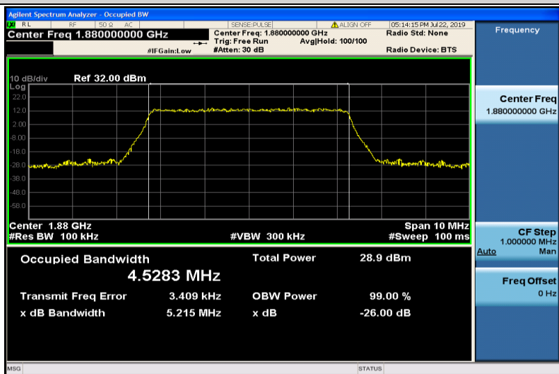
Band2-5MHz-16QAM-18900-25RB#0-4.5283
