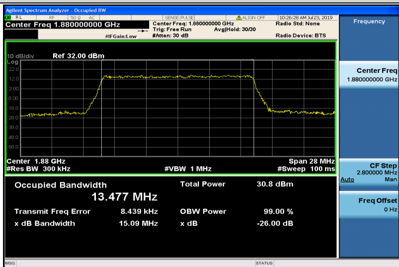
Band2-15MHz-QPSK-18900-75RB#0-13.477
