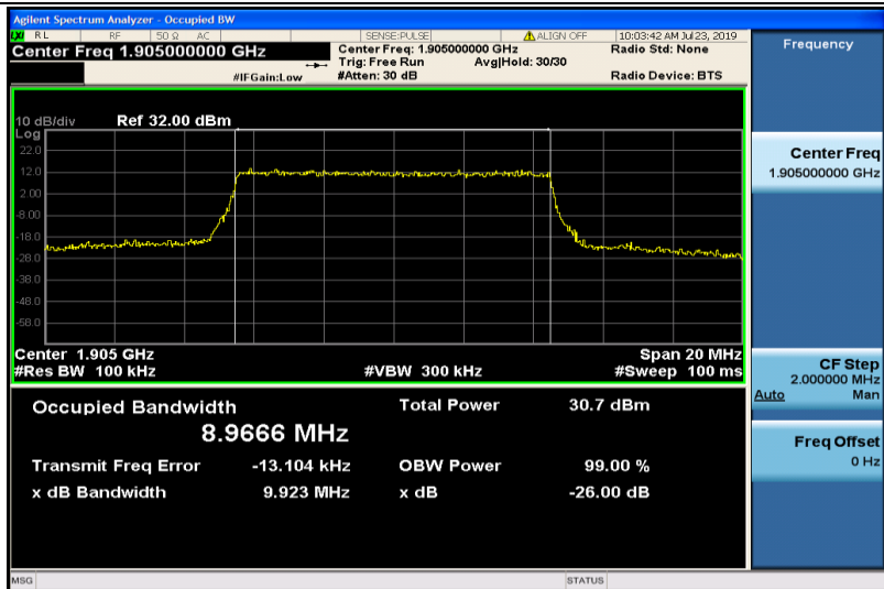
Band2-10MHz-QPSK-19150-50RB#0-8.9666
