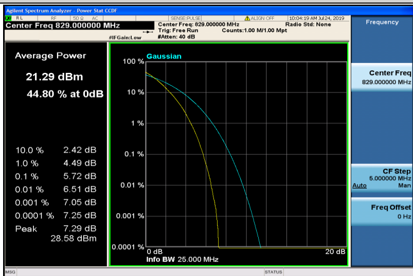
Band5-10MHz-QPSK-20450-50RB#0
