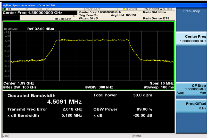
Band2-5MHz-QPSK-18900-25RB#0-4.5091
