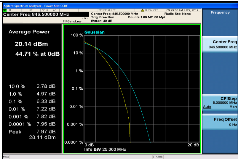
Band5-5MHz-16QAM-20625-25RB#0
