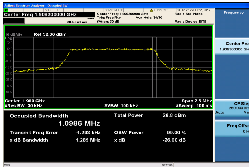
Band2-1.4MHz-QPSK-19193-6RB#0-1.0986
