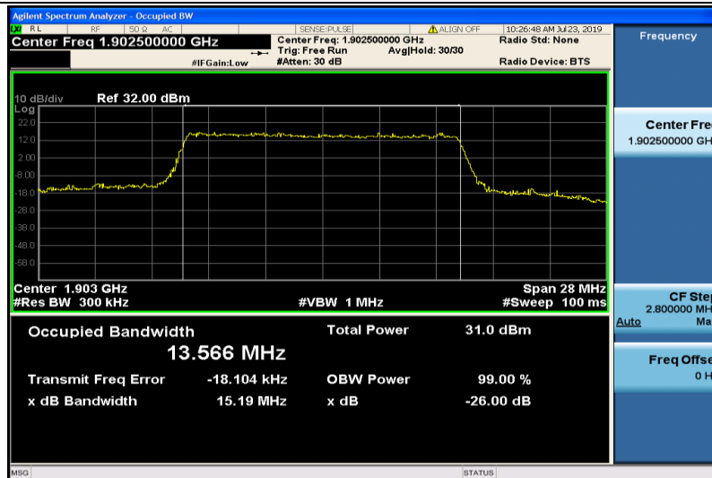
Band2-15MHz-QPSK-19125-75RB#0-13.566
