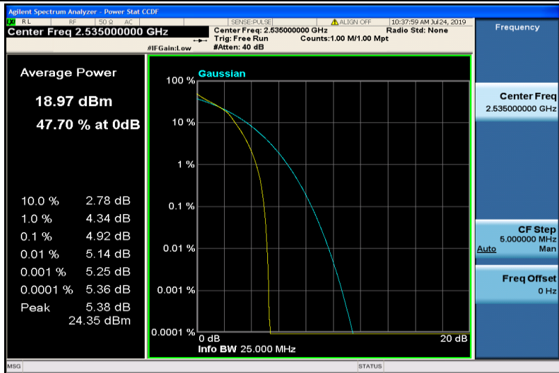
Band7-10MHz-16QAM-21100-50RB#0
