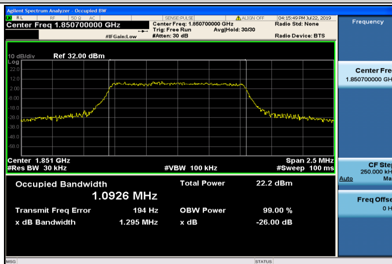
Band2-1.4MHz-16QAM-18607-6RB#0-1.0926
