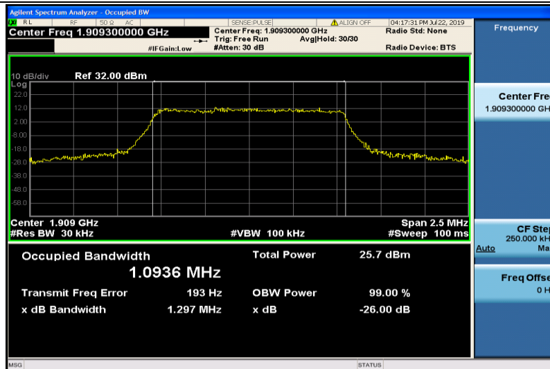
Band2-1.4MHz-16QAM-19193-6RB#0-1.0936
