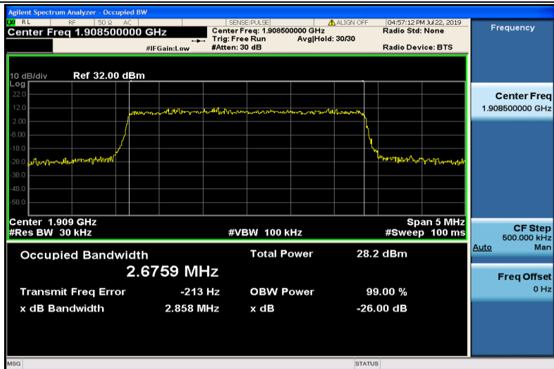
Band2-3MHz-16QAM-19185-15RB#0-2.6759
