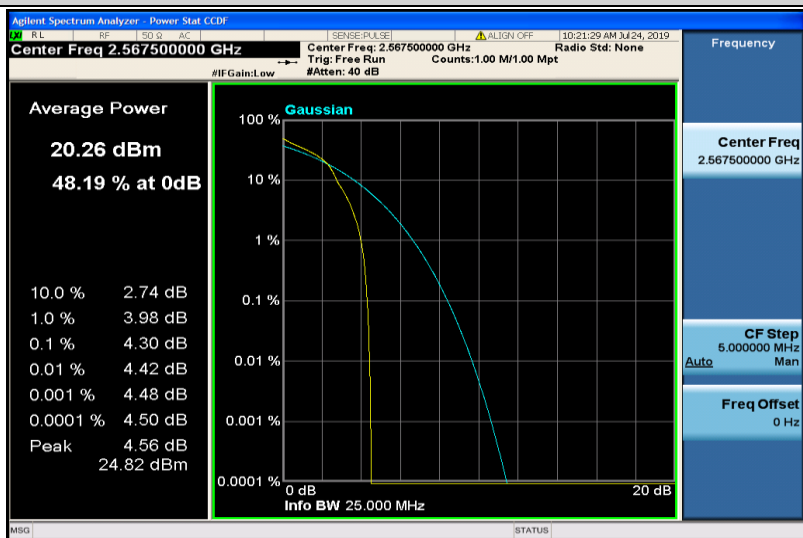
Band7-5MHz-16QAM-21425-1RB#0
