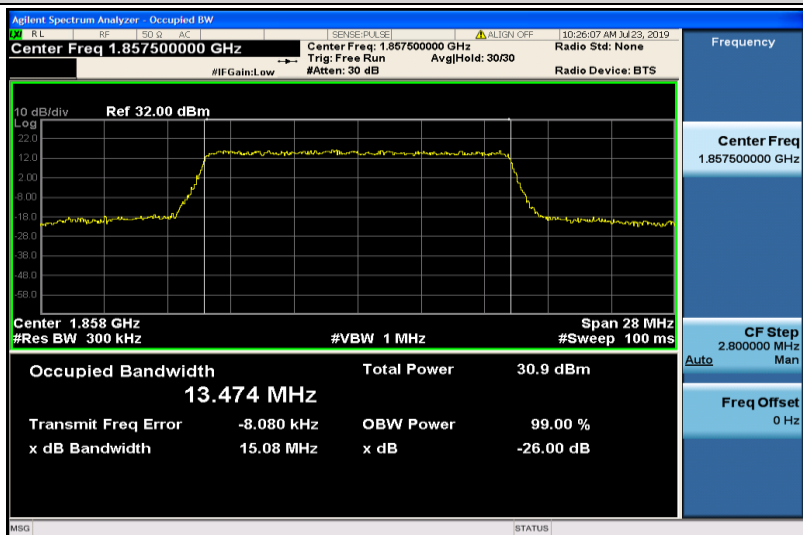
Band2-15MHz-QPSK-18675-75RB#0-13.474
