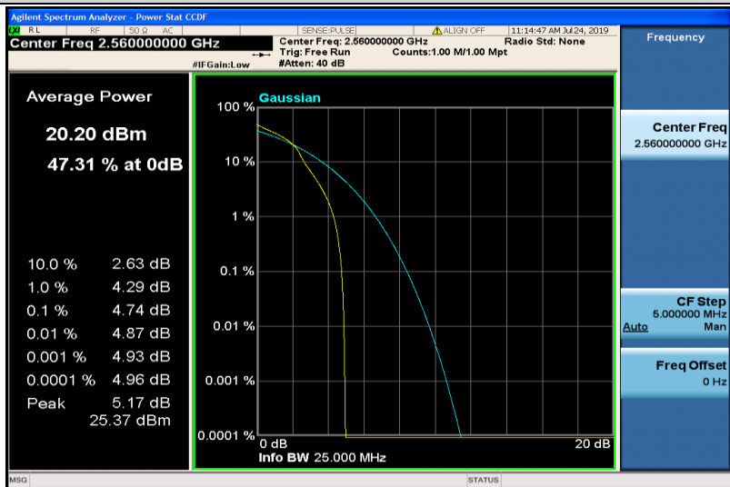
Band7-20MHz-16QAM-21350-1RB#0
