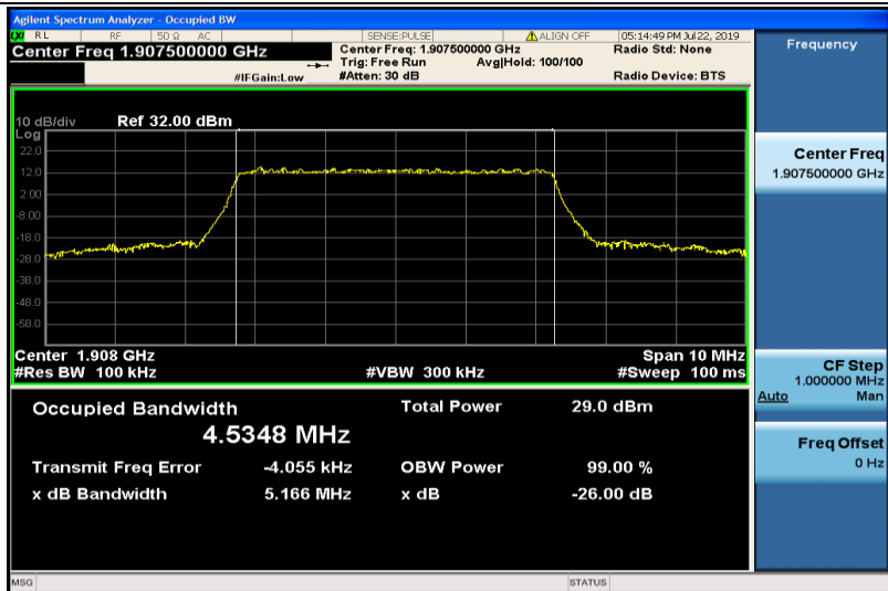
Band2-5MHz-16QAM-19175-25RB#0-4.5348
