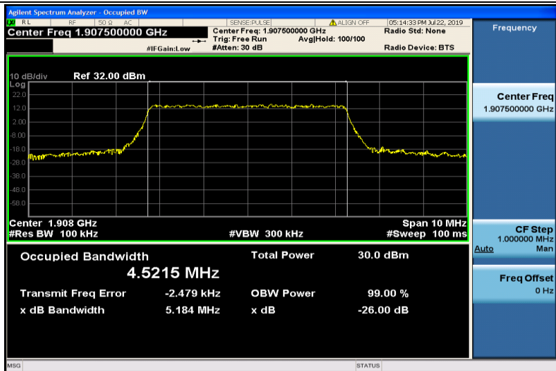
Band2-5MHz-QPSK-19175-25RB#0-4.5215
