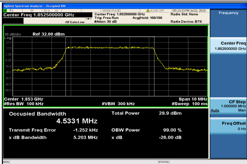
Band2-5MHz-QPSK-18625-25RB#0-4.5331
