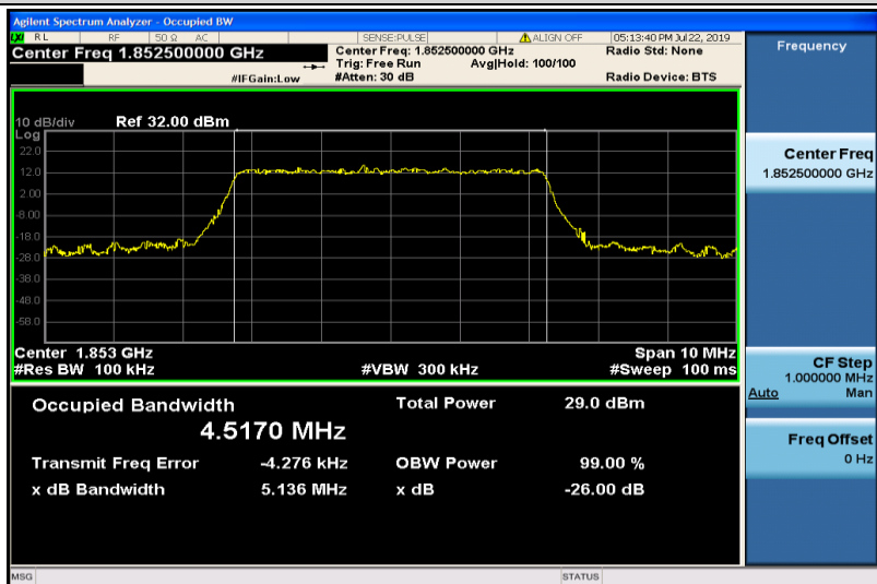
Band2-5MHz-16QAM-18625-25RB#0-4.5170
