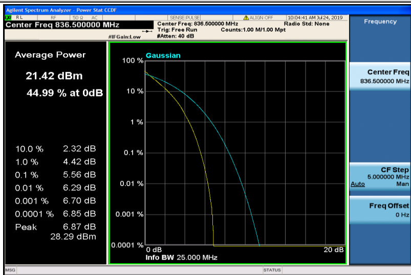
Band5-10MHz-QPSK-20525-50RB#0
