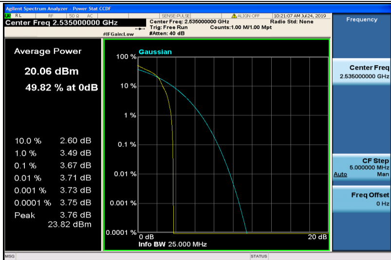
Band7-5MHz-16QAM-21100-1RB#0
