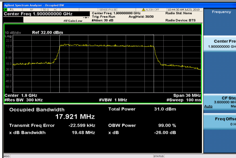
Band2-20MHz-QPSK-19100-100RB#0-17.921
