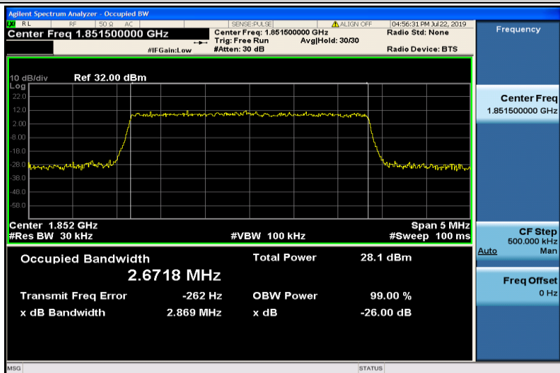
Band2-3MHz-16QAM-18615-15RB#0-2.6718
