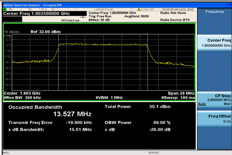
Band2-15MHz-16QAM-19125-75RB#0-13.527
