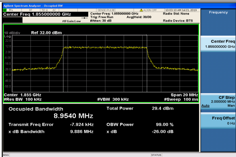
Band2-10MHz-16QAM-18650-50RB#0-8.9540
