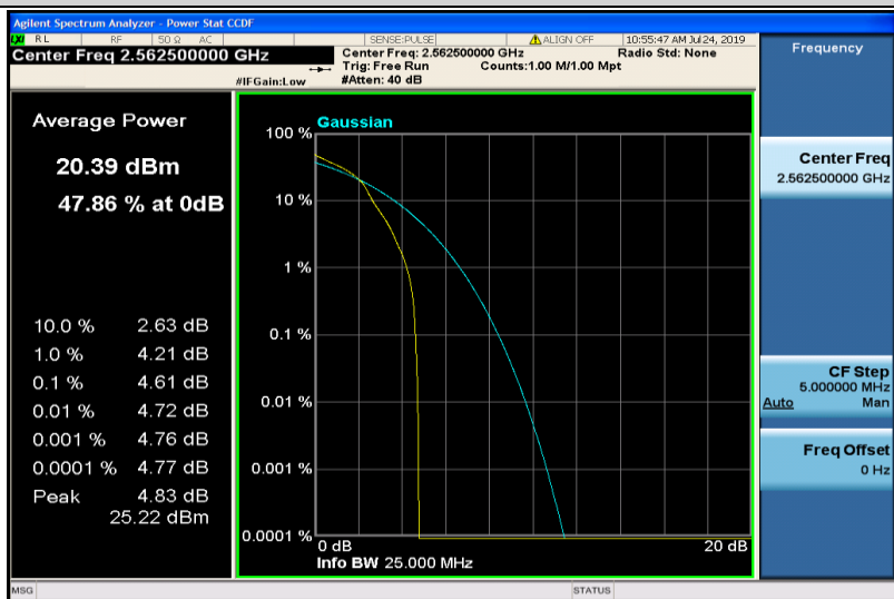
Band7-15MHz-16QAM-21375-1RB#0
