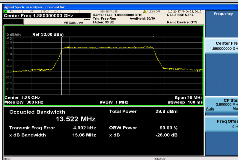
Band2-15MHz-16QAM-18900-75RB#0-13.522
