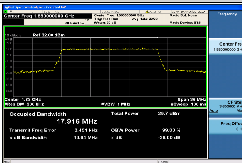
Band2-20MHz-16QAM-18900-100RB#0-17.916
