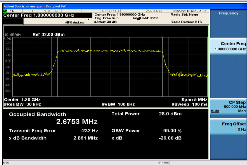
Band2-3MHz-16QAM-18900-15RB#0-2.6753
