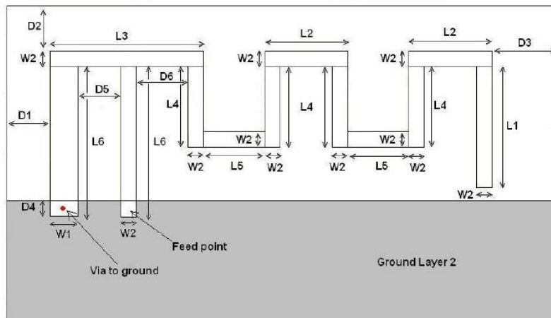
Figure 3: Antenna Dimensions
