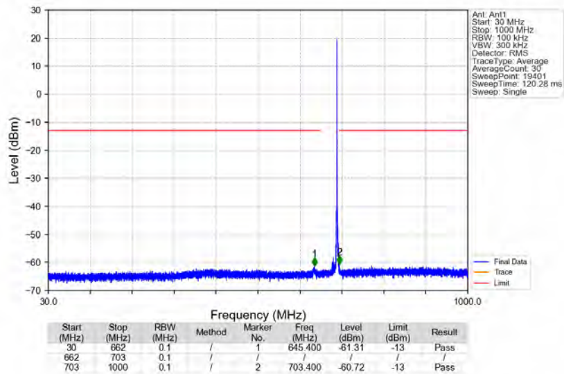
n71_15kHz_SISO_NTNV_10MHz_DFT-s-OFDM PI/2 BPSK_693MHz_Edge_1RB_Right
