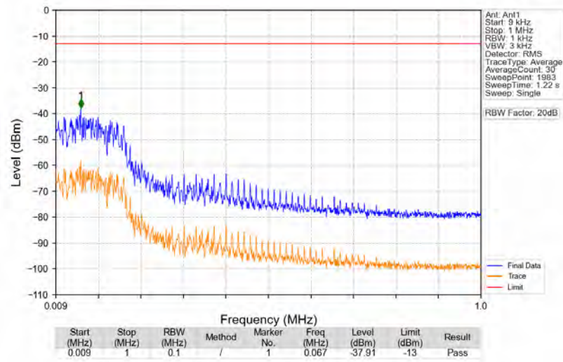
n71_15kHz_SISO_NTNV_10MHz_DFT-s-OFDM_QPSK_680.5MHz_Edge_1RB_Left
