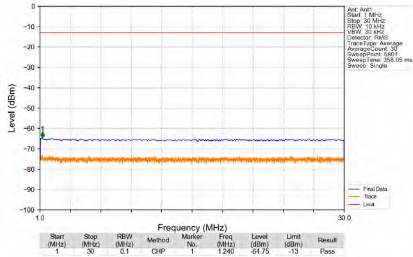
n71_15kHz_SISO_NTNV_10MHz_DFT-s-OFDM PI/2 BPSK_680.5MHz_Edge_1RB_Left
