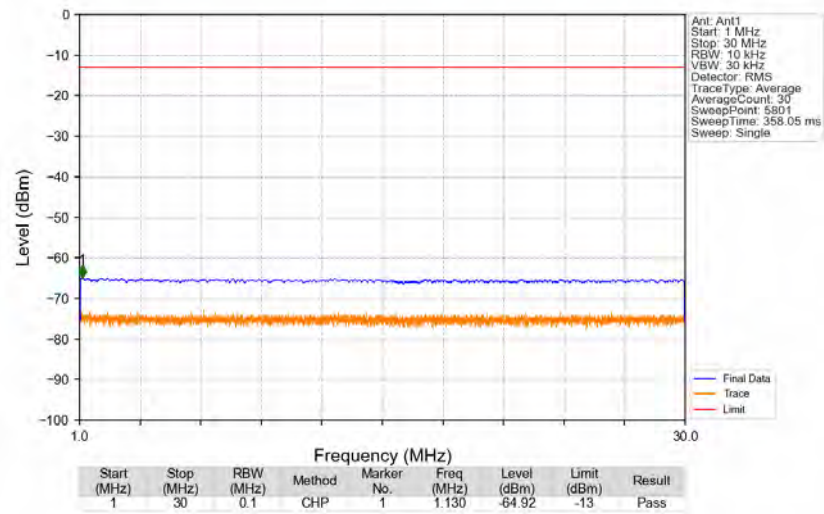
n71_15kHz_SISO_NTNV_10MHz_DFT-s-OFDM PI/2 BPSK_693MHz_Edge_1RB_Right
