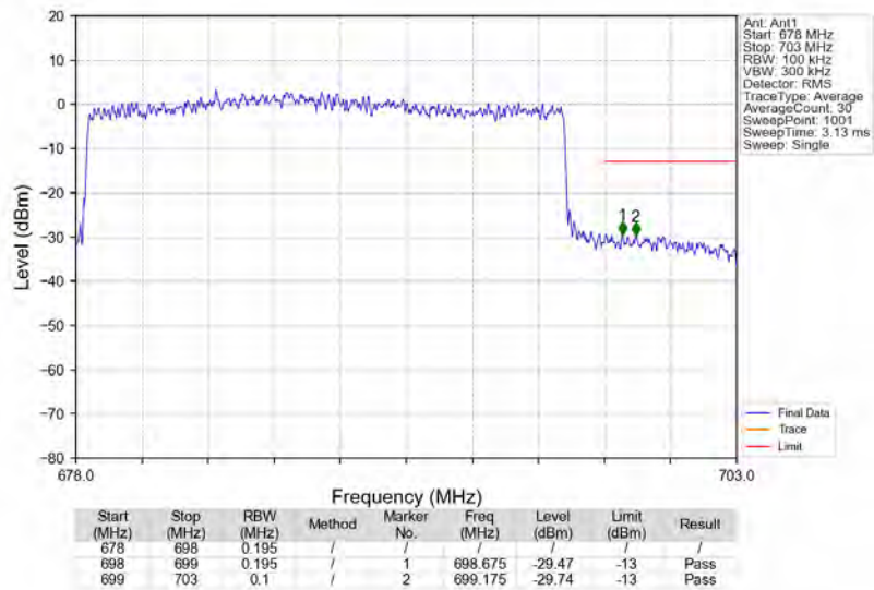
n71_15kHz_SISO_NTNV_20MHz_DFT-s-OFDM_QPSK_688MHz_Outer_Full
