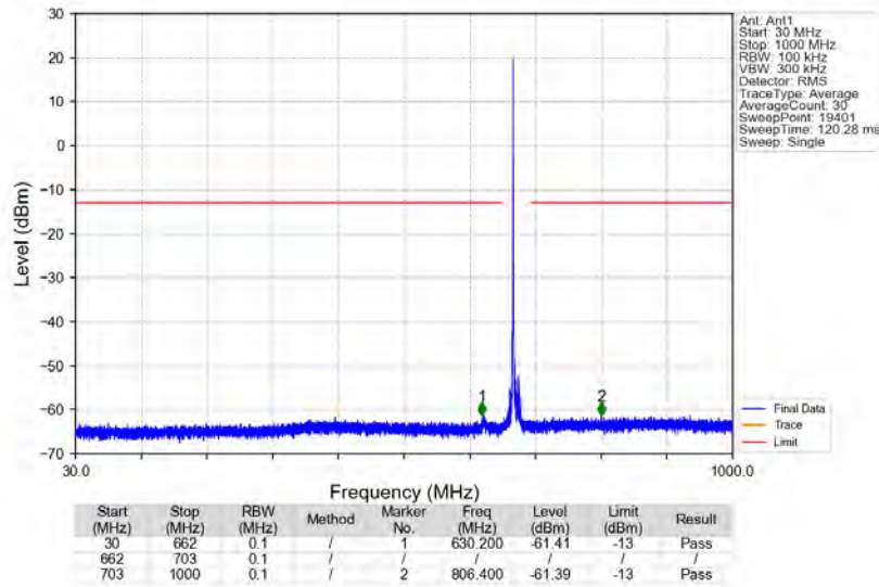
n71_15kHz_SISO_NTNV_10MHz_DFT-s-OFDM_QPSK_680.5MHz_Edge_1RB_Left
