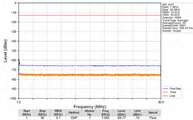
n71_15kHz_SISO_NTNV_15MHz_CP-OFDM_QPSK_680.5MHz_Edge_1RB_Left
