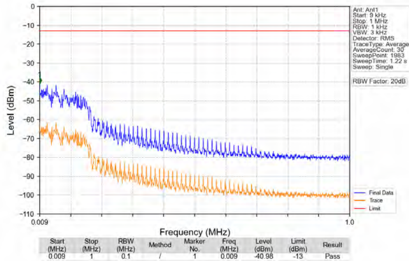
n71_15kHz_SISO_NTNV_10MHz_CP-OFDM_QPSK_668MHz_Edge_1RB_Left
