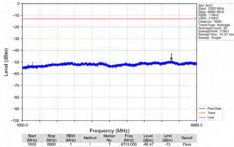
n71_15kHz_SISO_NTNV_10MHz_DFT-s-OFDM_QPSK_680.5MHz_Edge_1RB_Left
