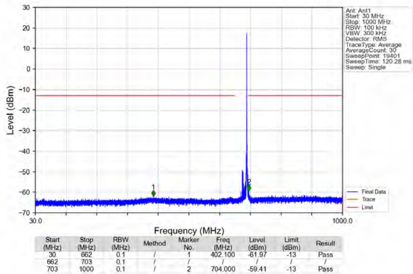
n71_15kHz_SISO_NTNV_15MHz_CP-OFDM_QPSK_690.5MHz_Edge_1RB_Right
