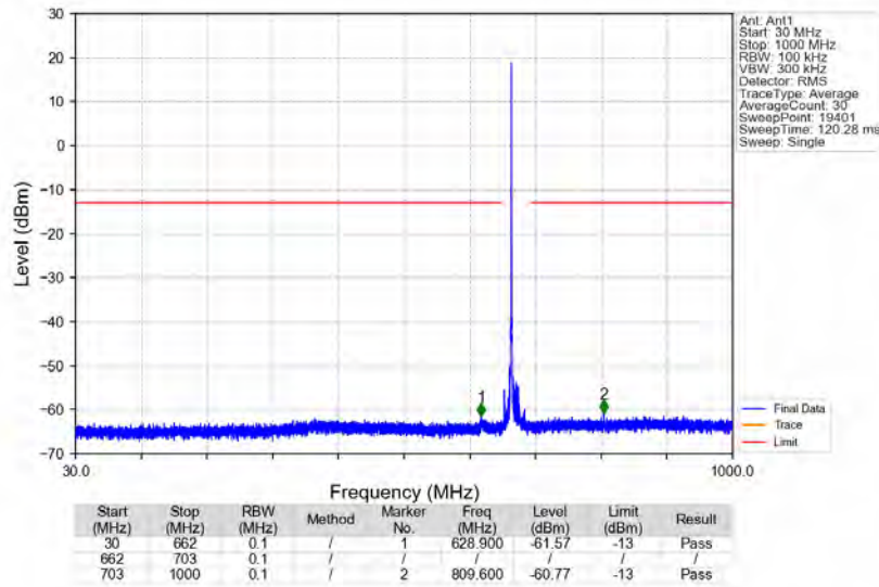
n71_15kHz_SISO_NTNV_15MHz_DFT-s-OFDM_QPSK_680.5MHz_Edge_1RB_Left
