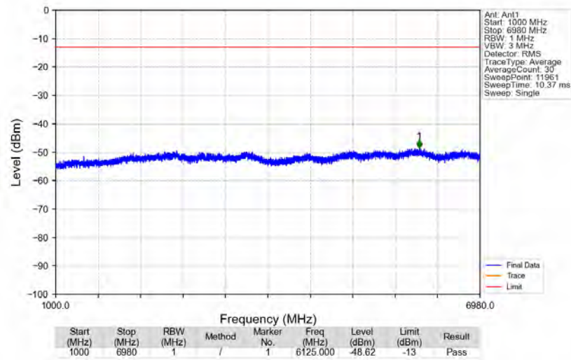
n71_15kHz_SISO_NTNV_10MHz_DFT-s-OFDM_QPSK_693MHz_Edge_1RB_Right
