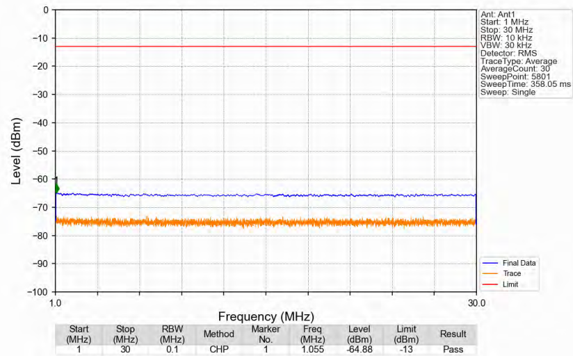
n71_15kHz_SISO_NTNV_10MHz_CP-OFDM_QPSK_668MHz_Edge_1RB_Left
