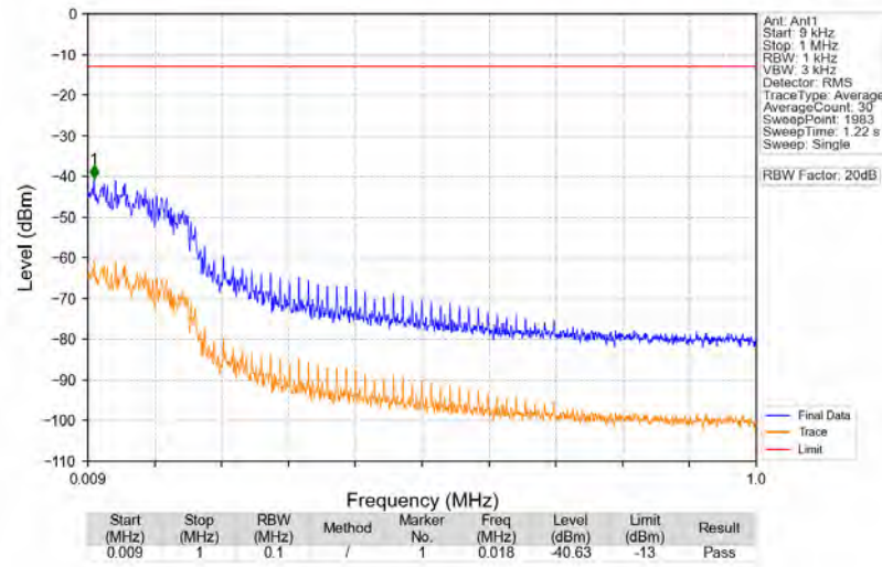
n71_15kHz_SISO_NTNV_10MHz_CP-OFDM QPSK 680.5MHz_Edge_1RB_Left
