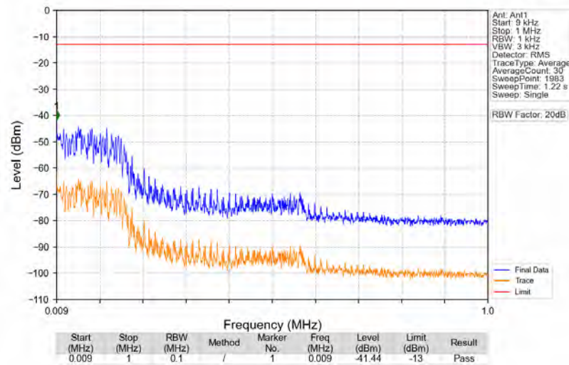
n71_15kHz_SISO_NTNV_15MHz_DFT-s-OFDM_QPSK_670.5MHz_Edge_1RB_Left
