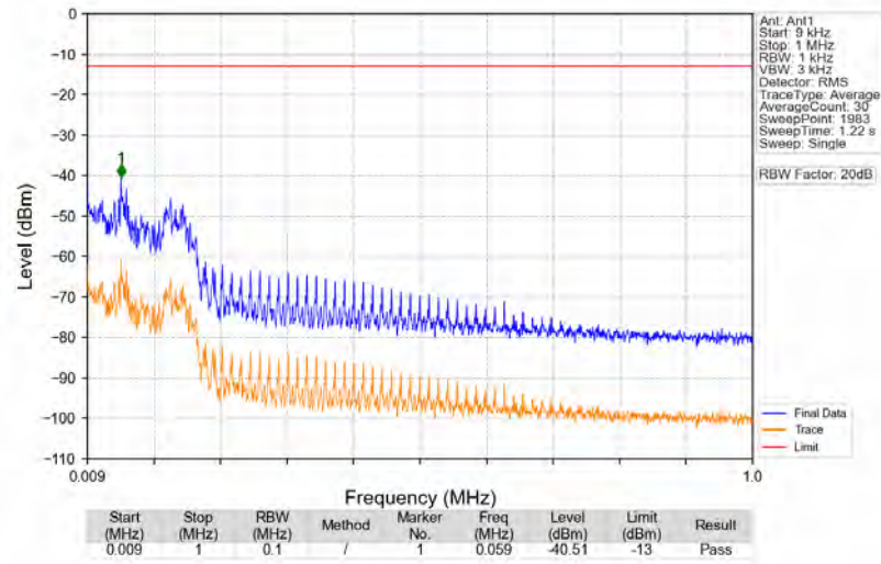
n71_15kHz_SISO_NTNV_20MHz_DFT-s-OFDM PI/2 BPSK_680.5MHz_Edge_1RB_Left
