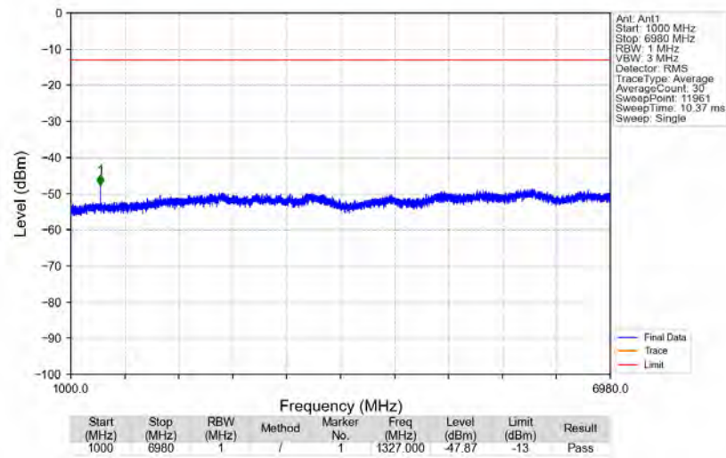
n71_15kHz_SISO_NTNV_15MHz_DFT-s-OFDM_QPSK_670.5MHz_Edge_1RB_Left
