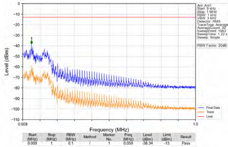
n71_15kHz_SISO_NTNV_15MHz_DFT-s-OFDM_PI/2_BPSK_680.5MHz_Edge_1RB_Left
