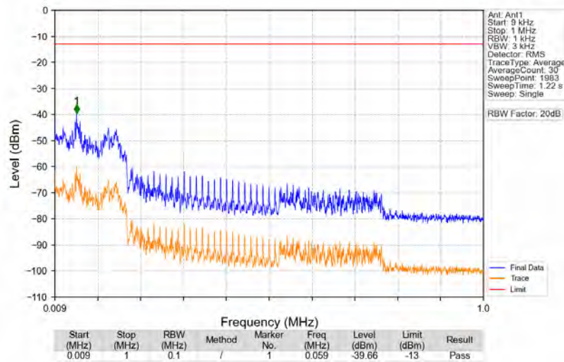
n71_15kHz_SISO_NTNV_10MHz_DFT-s-OFDM PI/2 BPSK_693MHz_Edge_1RB_Right
