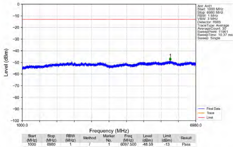
n71_15kHz_SISO_NTNV_20MHz_CP-OFDM_QPSK_680.5MHz_Edge_1RB_Left
