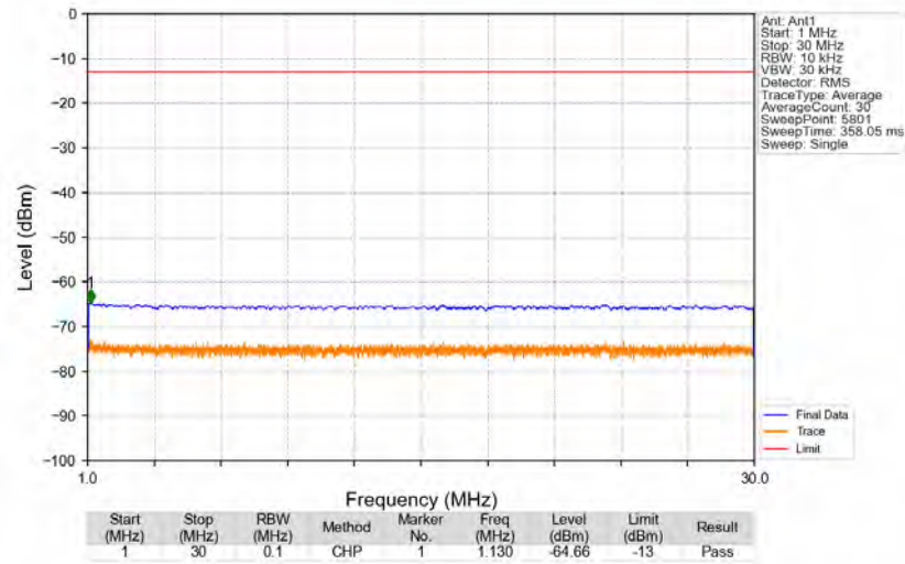
n71_15kHz_SISO_NTNV_10MHz_CP-OFDM QPSK 680.5MHz_Edge_1RB_Left
