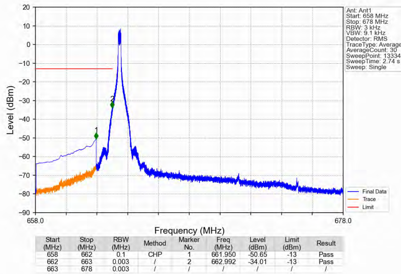
n71_15kHz_SISO_NTNV_15MHz_DFT-s-OFDM_QPSK_670.5MHz_Edge_1RB_Left
