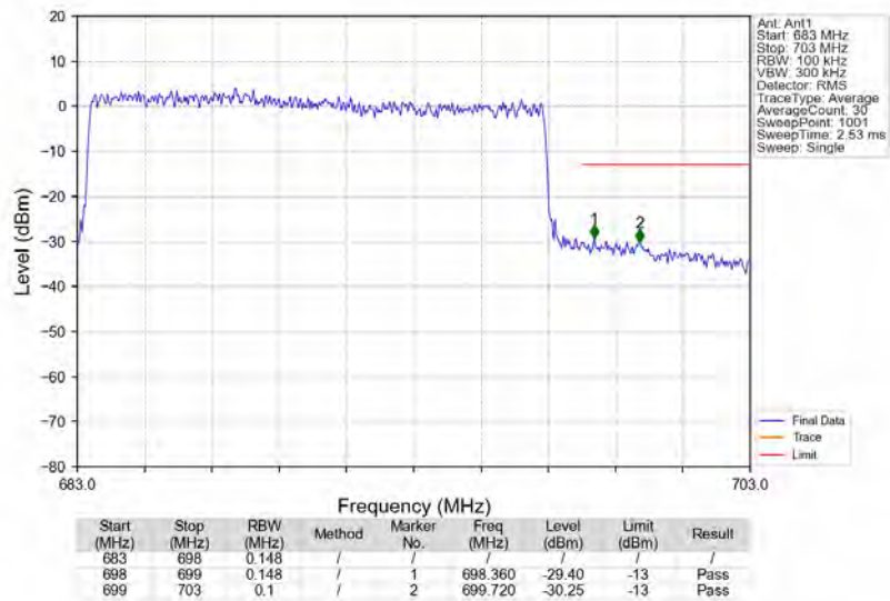
n71_15kHz_SISO_NTNV_15MHz_DFT-s-OFDM_QPSK_690.5MHz_Outer_Full
