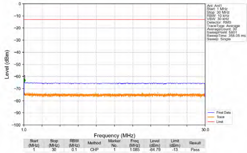
n71_15kHz_SISO_NTNV_20MHz_DFT-s-OFDM PI/2 BPSK_680.5MHz_Edge_1RB_Left
