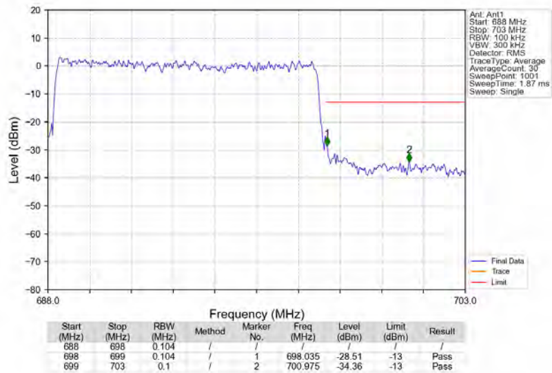
n71_15kHz_SISO_NTNV_10MHz_CP-OFDM_QPSK_693MHz_Outer_Full
