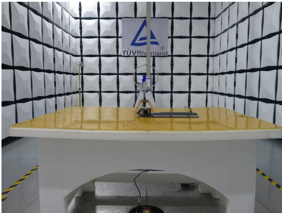
Photograph 2: Set-up photo for Radiated Spurious Emission, Below 30MHz
