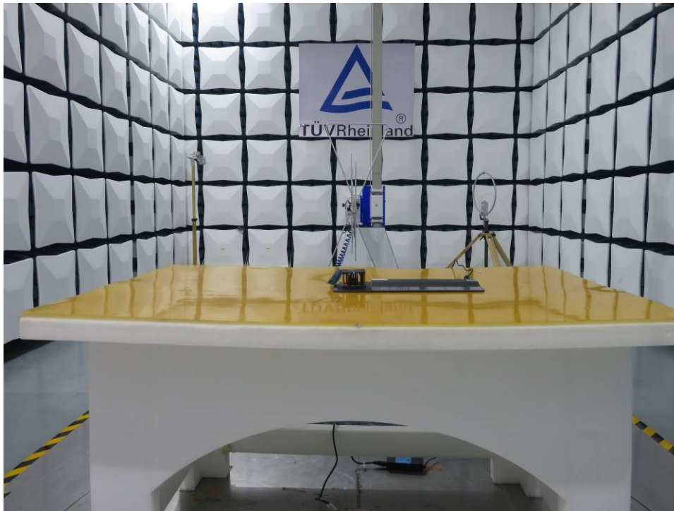
Photograph 3: Set-up photo for Radiated Spurious Emission, 30MHz - 1GHz
