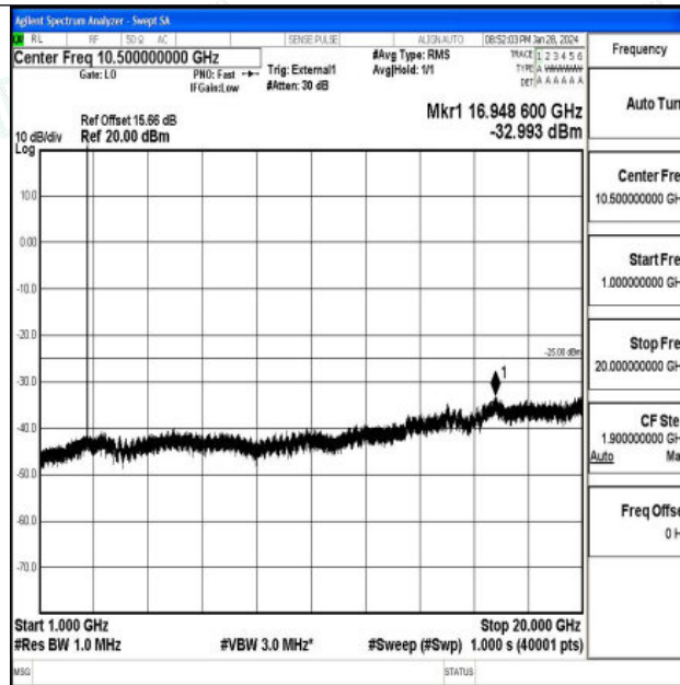
Band41_10MHz_16QAM_41540_1RB#0_1000~20000_1000~20000
