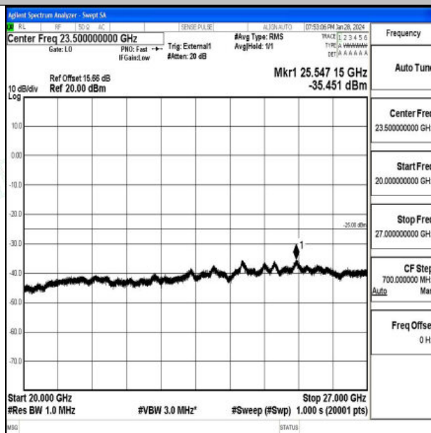
Band41_15MHz_16QAM_40620_1RB#0_20000~27000_20000~27000
