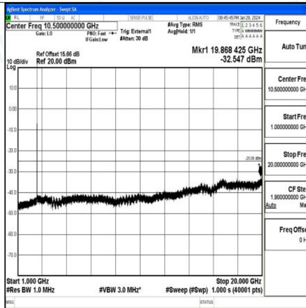
Band41_10MHz_16QAM_39700_1RB#0_1000~20000_1000~20000
