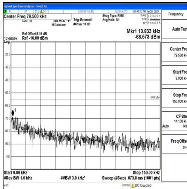
Band41_10MHz_QPSK_41540_1RB#0_0.009~0.15_0.009~0.15
