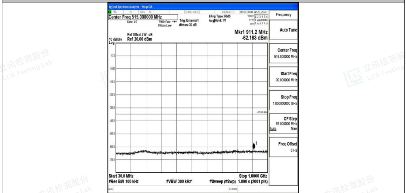
Band41_10MHz_16QAM_41540_1RB#0_30~1000_30~1000
