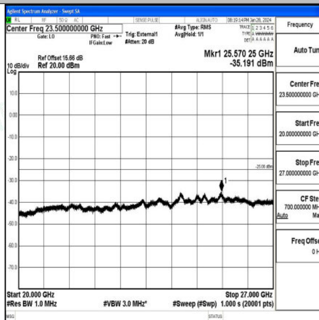
Band41_20MHz_16QAM_41490_1RB#0_20000~27000_20000~27000
