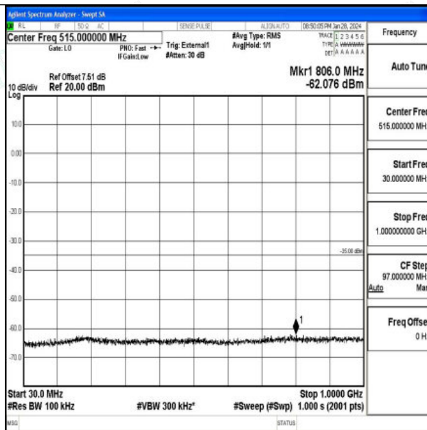
Band41_10MHz_QPSK_41540_1RB#0_30~1000_30~1000
