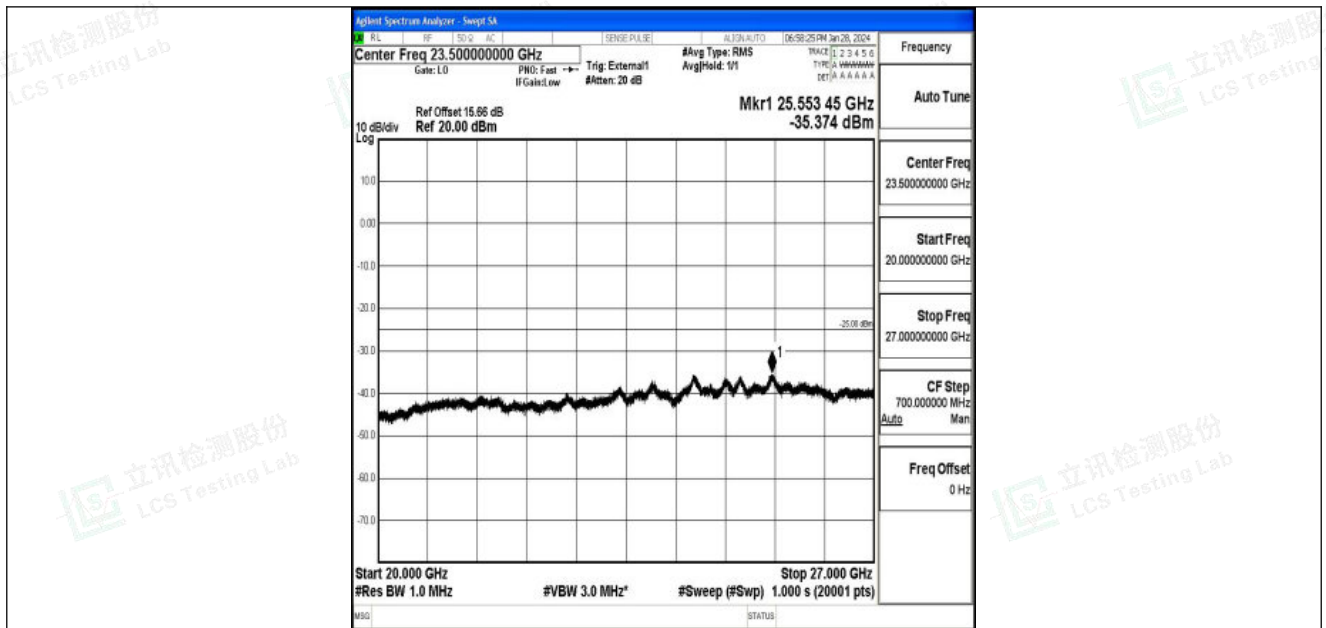
Band41_5MHz_QPSK_41565_1RB#0_20000~27000_20000~27000
