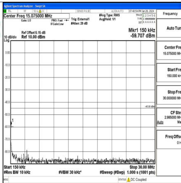
Band41_15MHz_16QAM_39725_1RB#0_0.15~30_0.15~30
