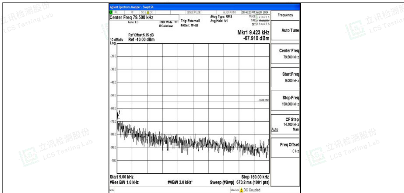
Band41_10MHz_QPSK_40620_1RB#0_0.009~0.15_0.009~0.15
