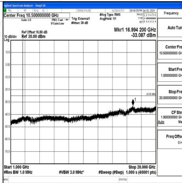
Band41_10MHz_16QAM_40620_1RB#0_1000~20000_1000~20000
