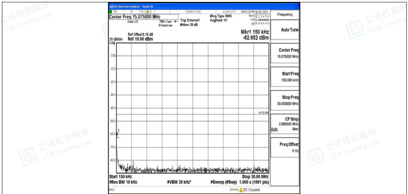
Band41_10MHz_16QAM_41540_1RB#0_0.15~30_0.15~30
