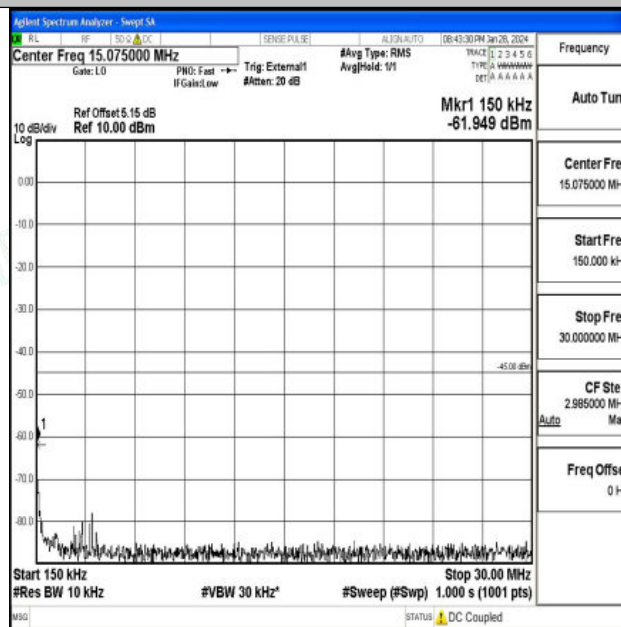
Band41_10MHz_QPSK_39700_1RB#0_0.15~30_0.15~30
