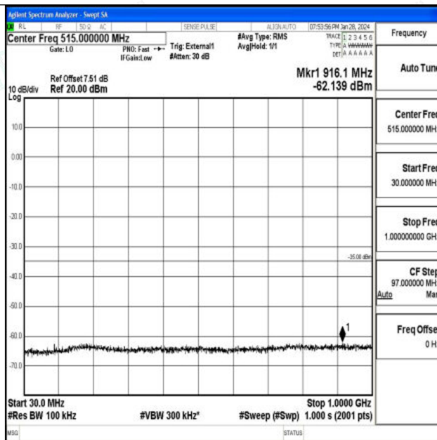
Band41_15MHz_QPSK_41515_1RB#0_30~1000_30~1000
