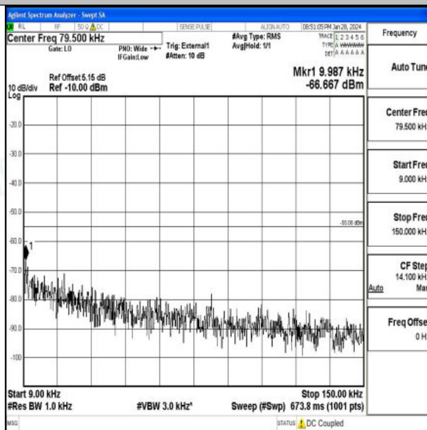
Band41_10MHz_16QAM_41540_1RB#0_0.009~0.15_0.009~0.15
