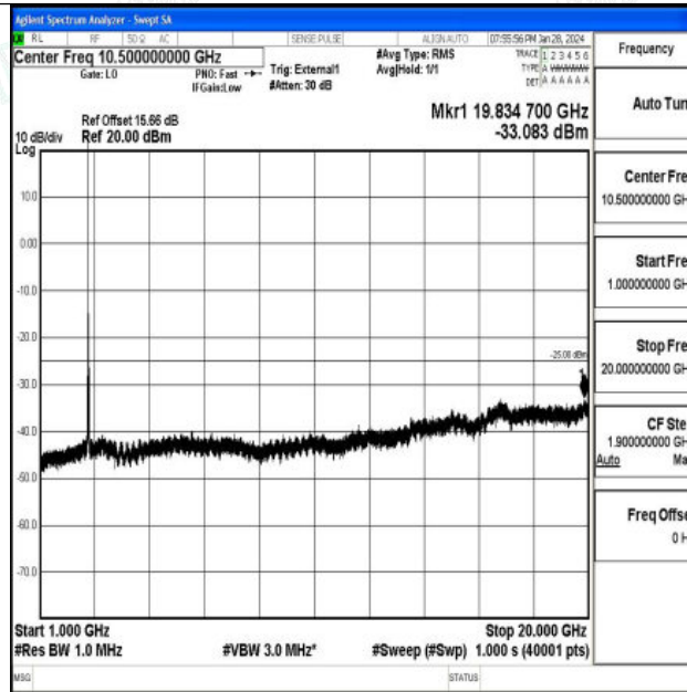
Band41_15MHz_16QAM_41515_1RB#0_1000~20000_1000~20000
