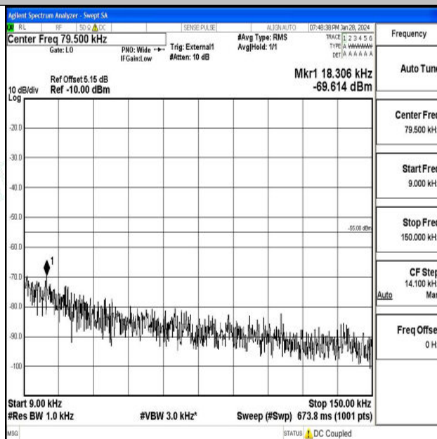
Band41_15MHz_16QAM_39725_1RB#0_0.009~0.15_0.009~0.15
