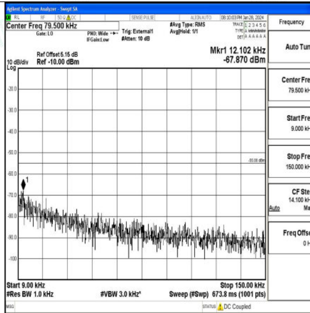
Band41_20MHz_QPSK_39750_1RB#0_0.009~0.15_0.009~0.15
