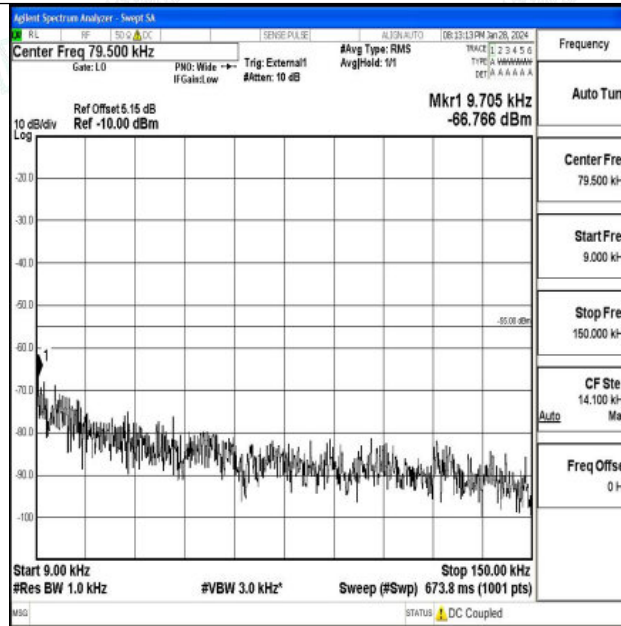
Band41_20MHz_QPSK_40620_1RB#0_0.009~0.15_0.009~0.15
