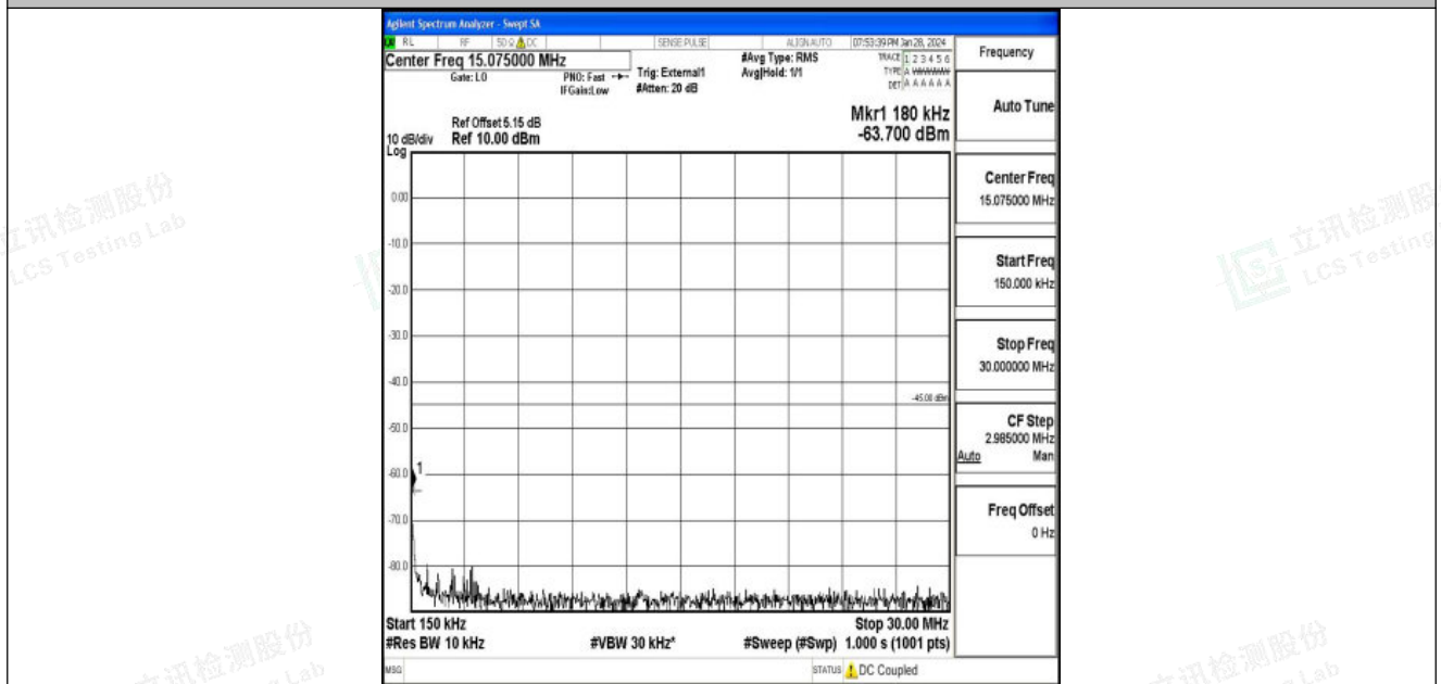
Band41_15MHz_QPSK_41515_1RB#0_0.15~30_0.15~30
