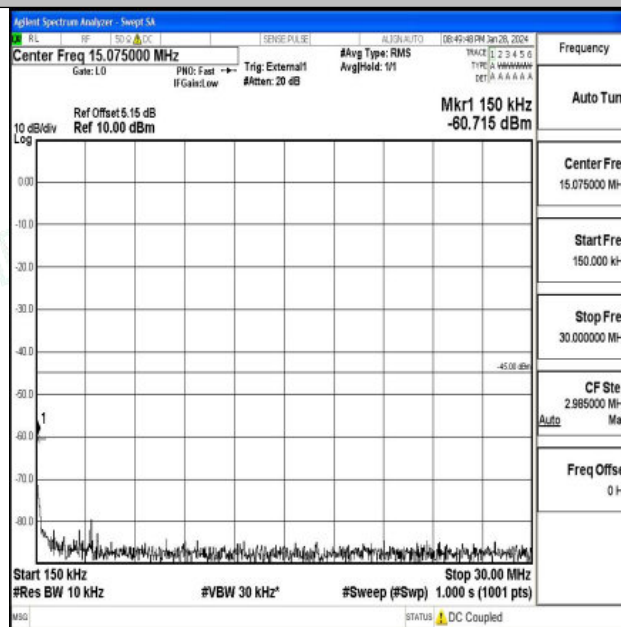
Band41_10MHz_QPSK_41540_1RB#0_0.15~30_0.15~30
