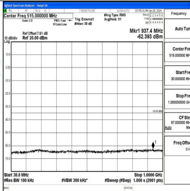
Band41_15MHz_16QAM_41515_1RB#0_30~1000_30~1000
