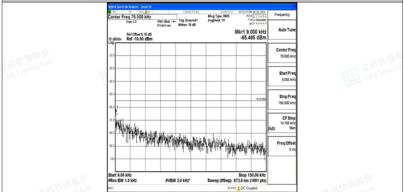
Band41_15MHz_16QAM_40620_1RB#0_0.009~0.15_0.009~0.15
