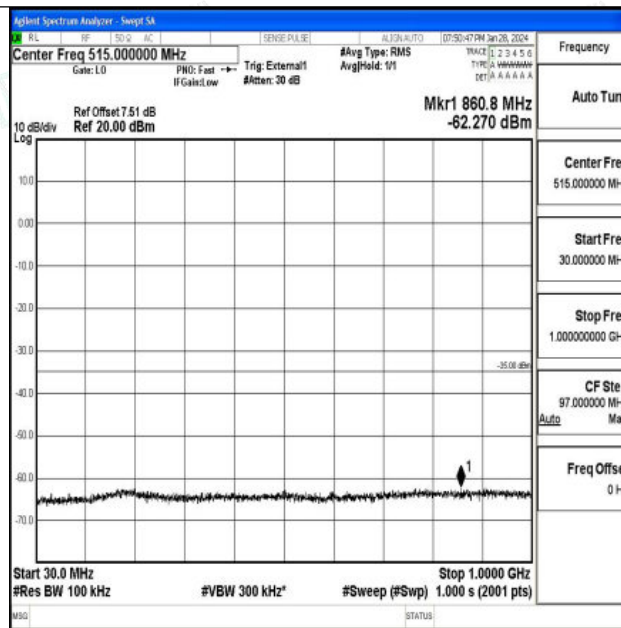
Band41_15MHz_QPSK_40620_1RB#0_30~1000_30~1000
