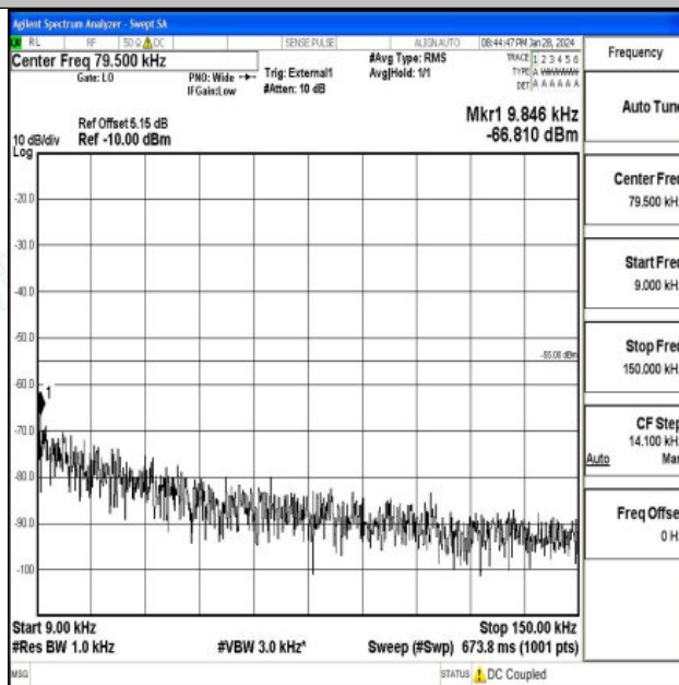
Band41_10MHz_16QAM_39700_1RB#0_0.009~0.15_0.009~0.15
