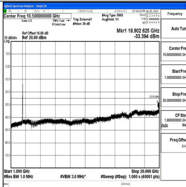
Band41_15MHz_QPSK_39725_1RB#0_1000~20000_1000~20000
