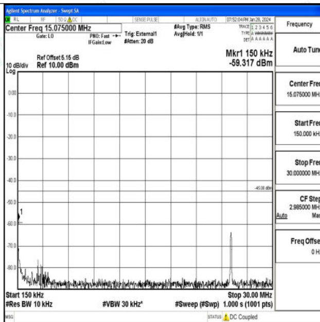
Band41_15MHz_16QAM_40620_1RB#0_0.15~30_0.15~30
