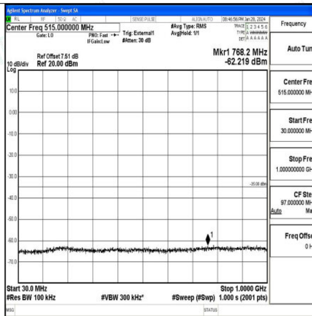
Band41_10MHz_QPSK_40620_1RB#0_30~1000_30~1000
