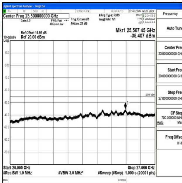
Band41_15MHz_QPSK_39725_1RB#0_20000~27000_20000~27000
