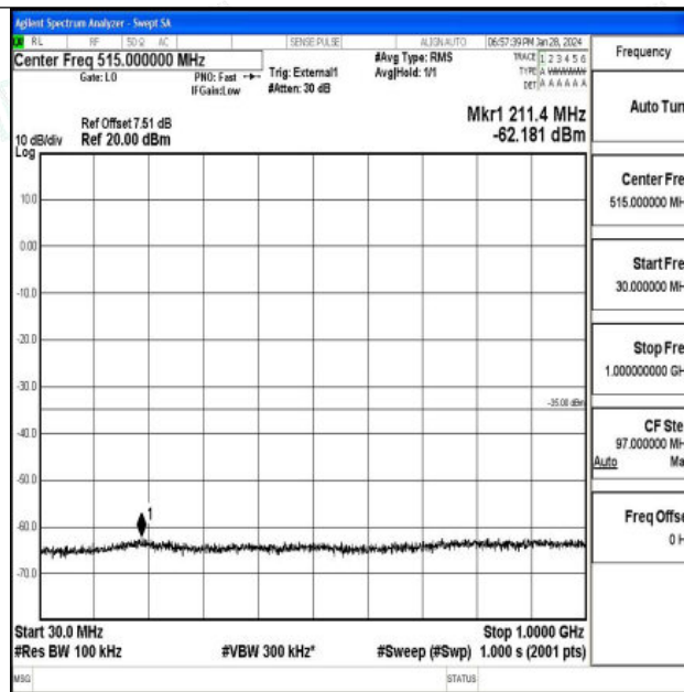
Band41_5MHz_QPSK_41565_1RB#0_30~1000_30~1000
