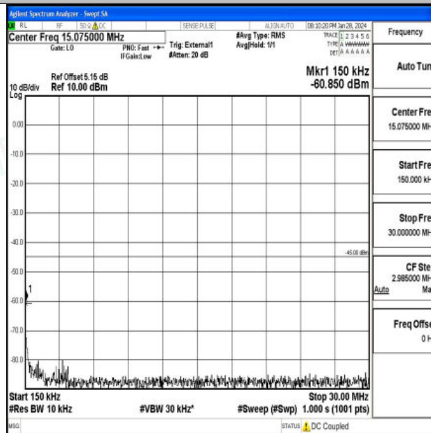
Band41_20MHz_QPSK_39750_1RB#0_0.15~30_0.15~30
