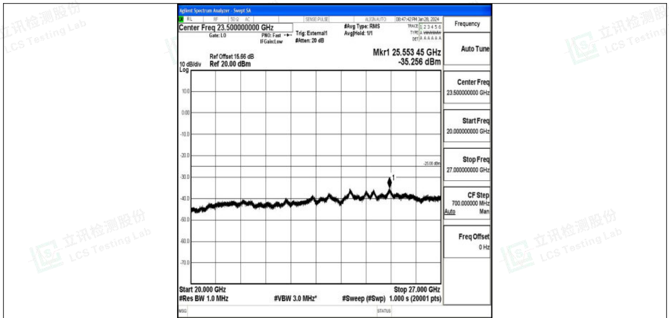
Band41_10MHz_QPSK_40620_1RB#0_20000~27000_20000~27000
