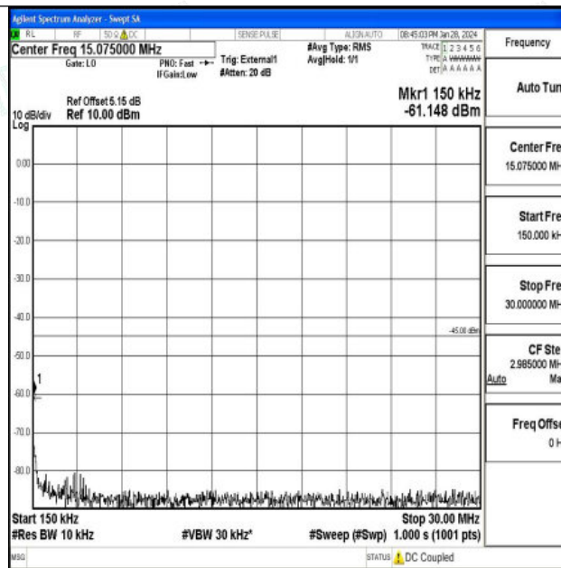
Band41_10MHz_16QAM_39700_1RB#0_0.15~30_0.15~30
