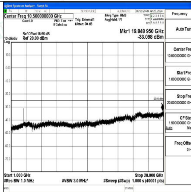
Band41_5MHz_16QAM_40620_1RB#0_1000~20000_1000~20000
