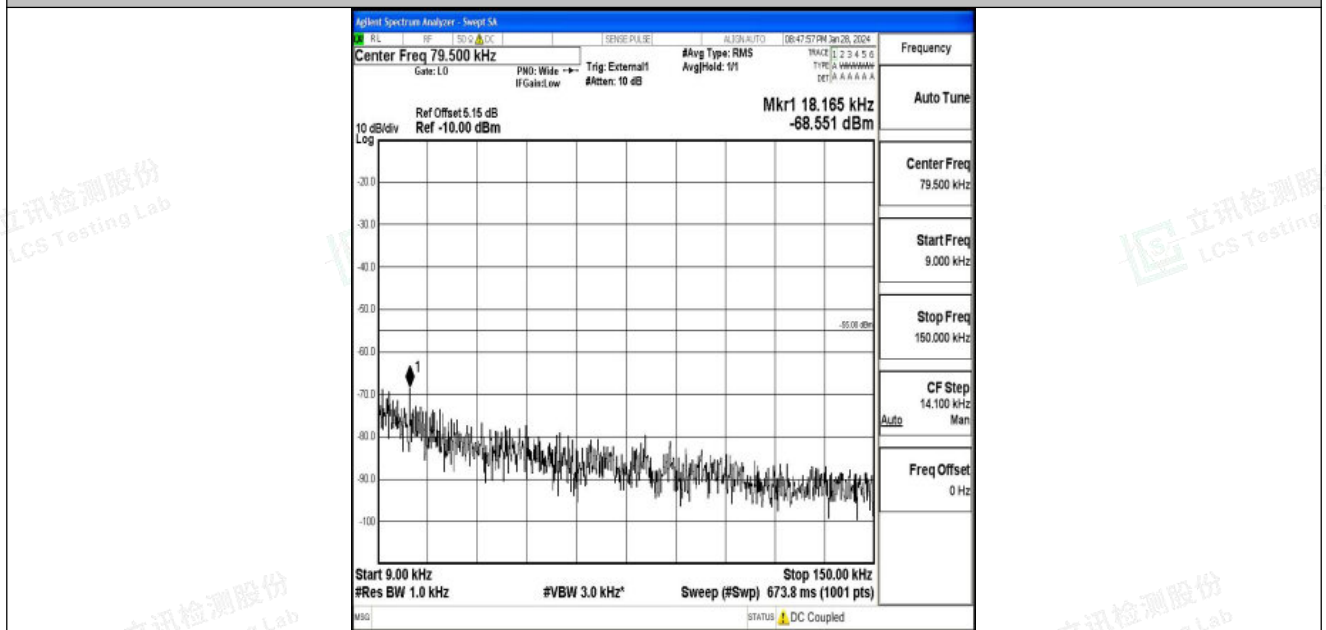
Band41_10MHz_16QAM_40620_1RB#0_0.009~0.15_0.009~0.15
