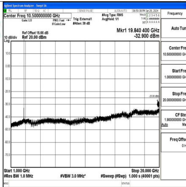
Band41_5MHz_16QAM_41565_1RB#0_1000~20000_1000~20000
