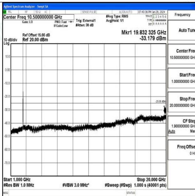
Band41_15MHz_16QAM_39725_1RB#0_1000~20000_1000~20000
