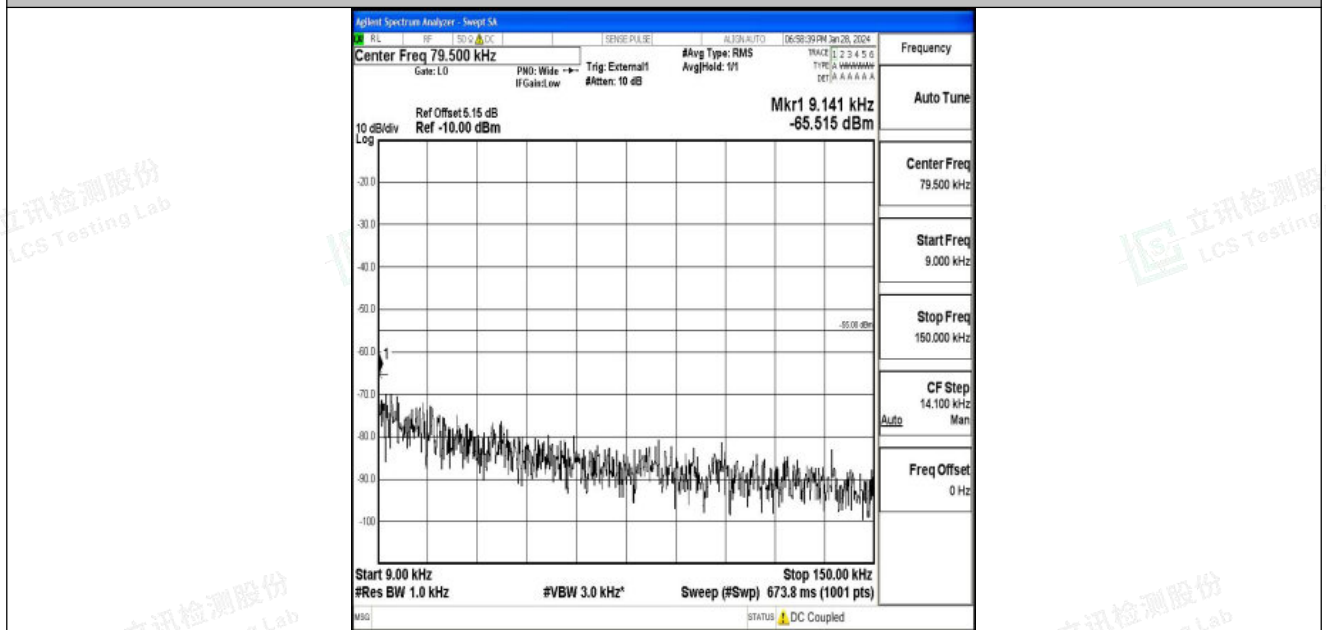
Band41_5MHz_16QAM_41565_1RB#0_0.009~0.15_0.009~0.15
