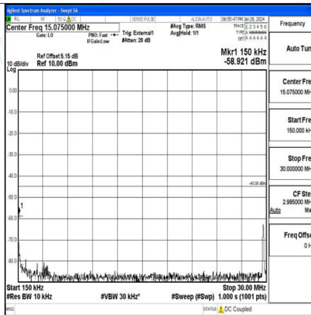
Band41_5MHz_16QAM_40620_1RB#0_0.15~30_0.15~30
