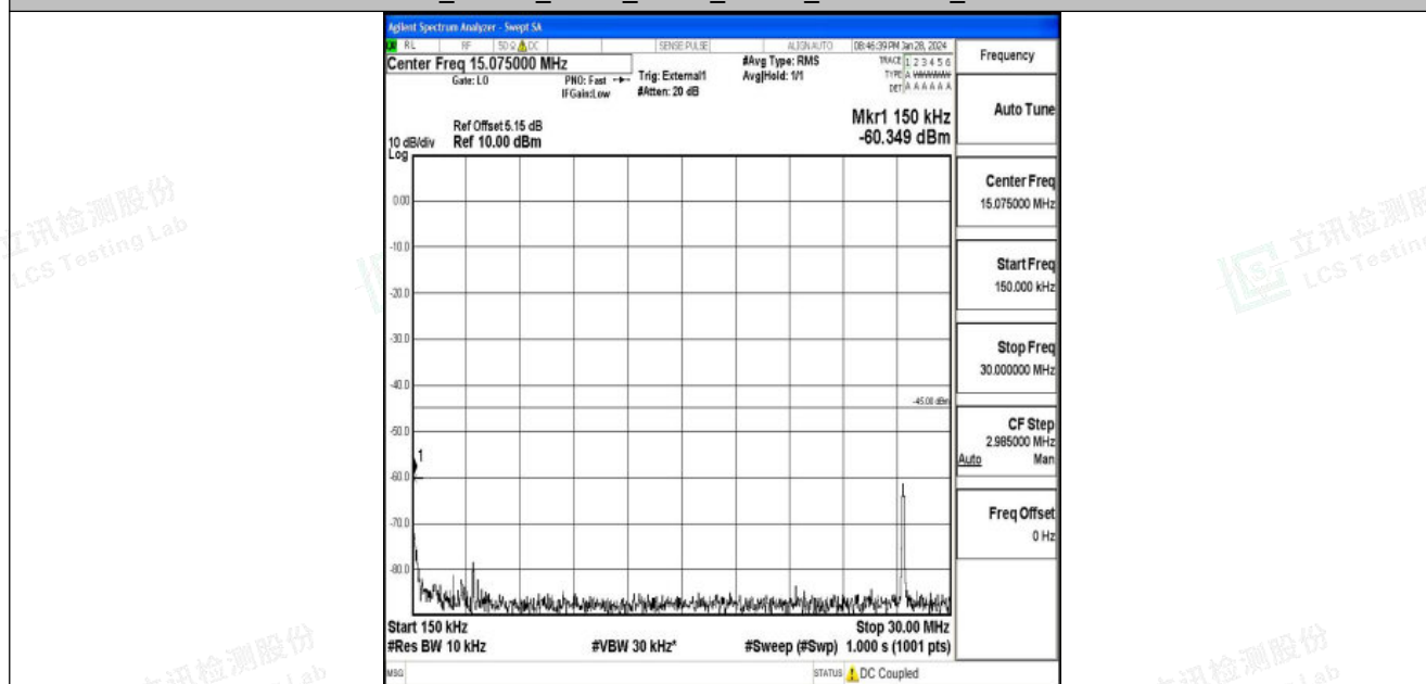
Band41_10MHz_QPSK_40620_1RB#0_0.15~30_0.15~30
