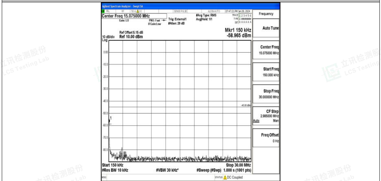
Band41_15MHz_QPSK_39725_1RB#0_0.15~30_0.15~30
