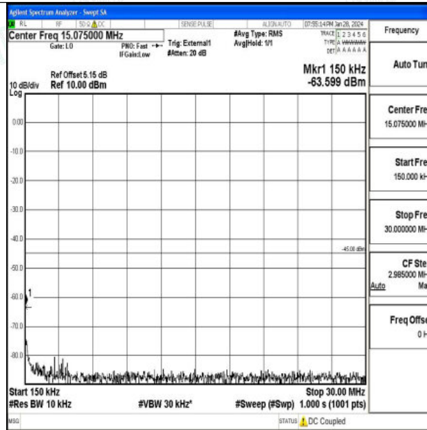
Band41_15MHz_16QAM_41515_1RB#0_0.15~30_0.15~30
