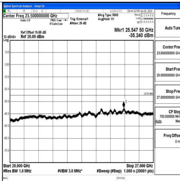
Band41_10MHz_QPSK_39700_1RB#0_20000~27000_20000~27000
