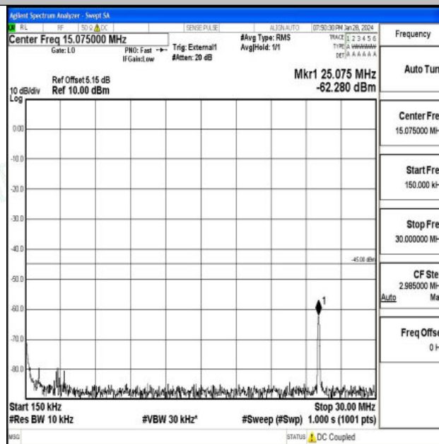
Band41_15MHz_QPSK_40620_1RB#0_0.15~30_0.15~30
