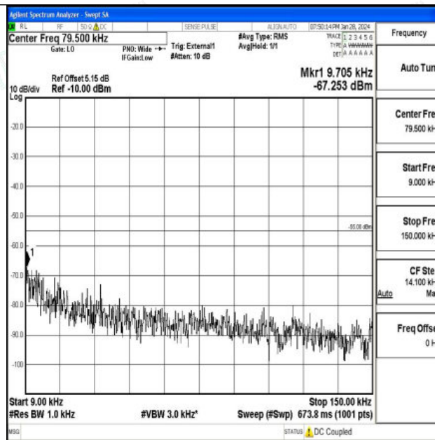
Band41_15MHz_QPSK_40620_1RB#0_0.009~0.15_0.009~0.15
