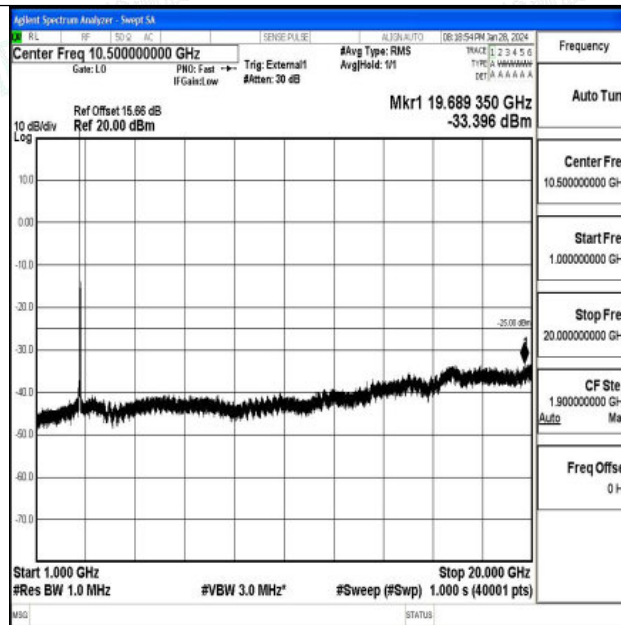
Band41_20MHz_16QAM_41490_1RB#0_1000~20000_1000~20000
