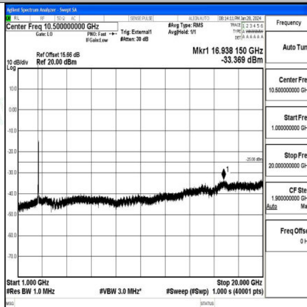
Band41_20MHz_QPSK_40620_1RB#0_1000~20000_1000~20000
