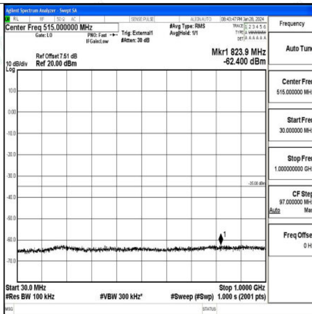
Band41_10MHz_QPSK_39700_1RB#0_30~1000_30~1000
