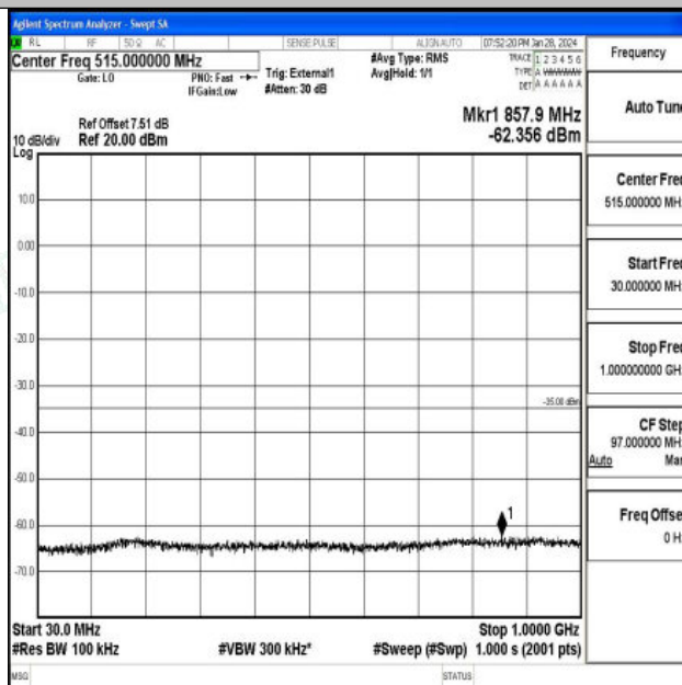
Band41_15MHz_16QAM_40620_1RB#0_30~1000_30~1000
