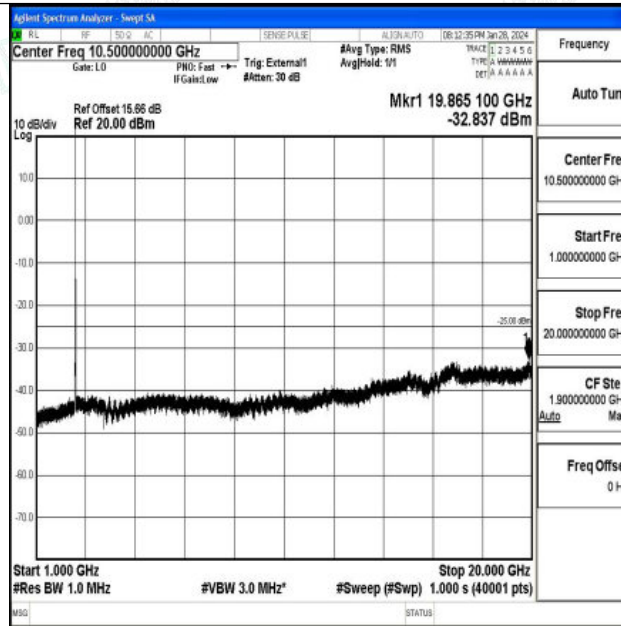
Band41_20MHz_16QAM_39750_1RB#0_1000~20000_1000~20000
