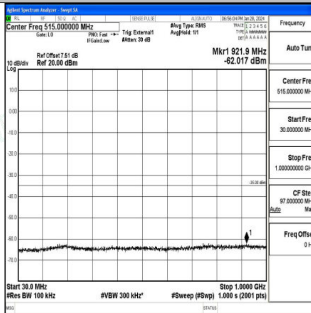
Band41_5MHz_16QAM_40620_1RB#0_30~1000_30~1000
