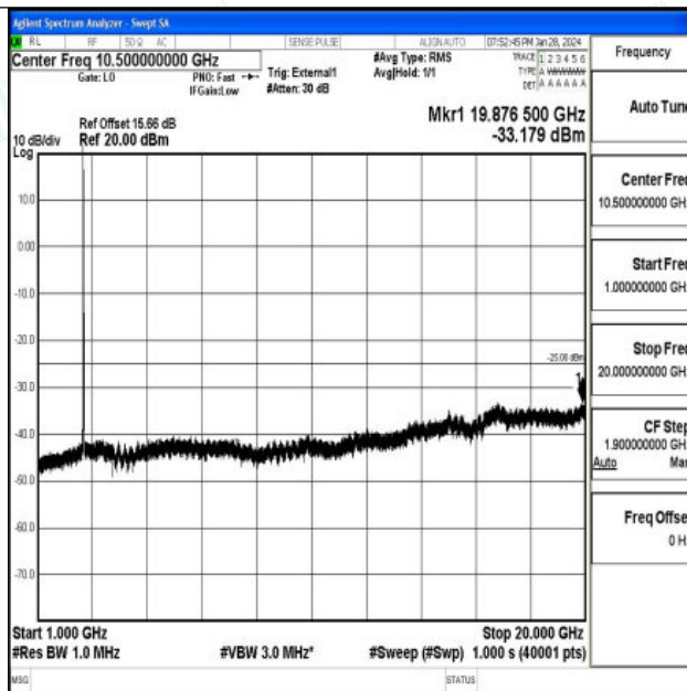
Band41_15MHz_16QAM_40620_1RB#0_1000~20000_1000~20000
