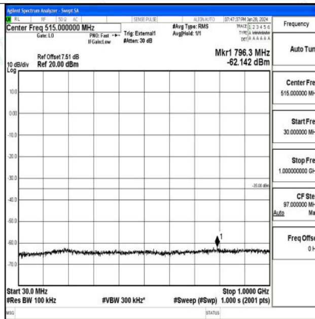
Band41_15MHz_QPSK_39725_1RB#0_30~1000_30~1000
