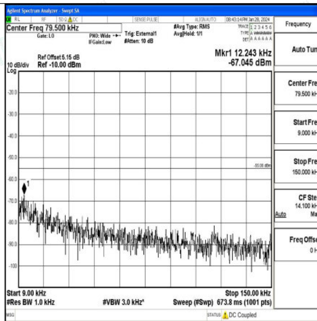
Band41_10MHz_QPSK_39700_1RB#0_0.009~0.15_0.009~0.15
