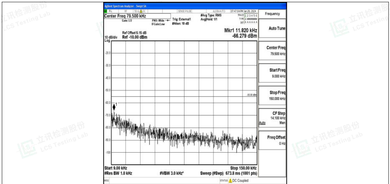
Band41_15MHz_QPSK_39725_1RB#0_0.009~0.15_0.009~0.15
