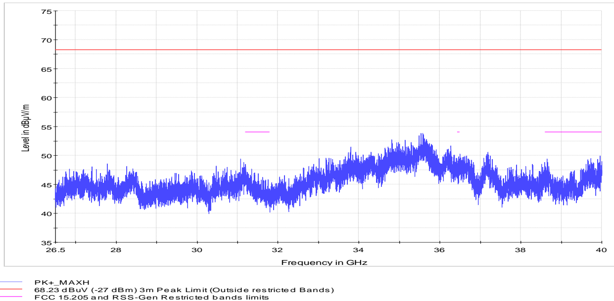
Figure 8.1-14: Radiated – Undesirable (unwanted) emissions 26 to 40 GHz, Channel 140 – 5700 MHz
