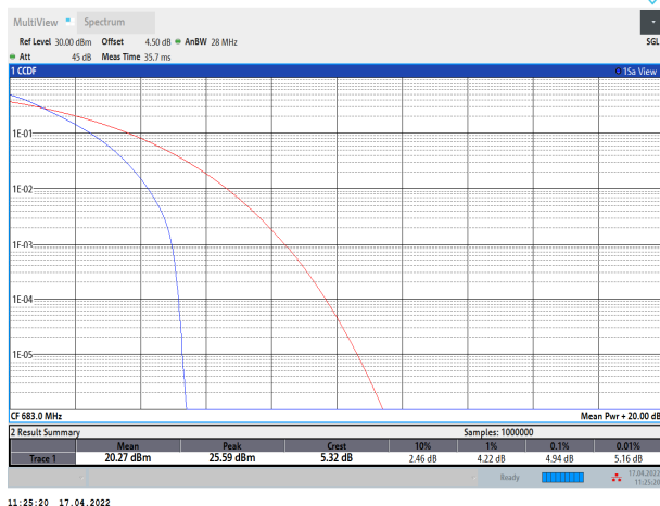
Band71-20MHz-QPSK-133322-100RB#0
