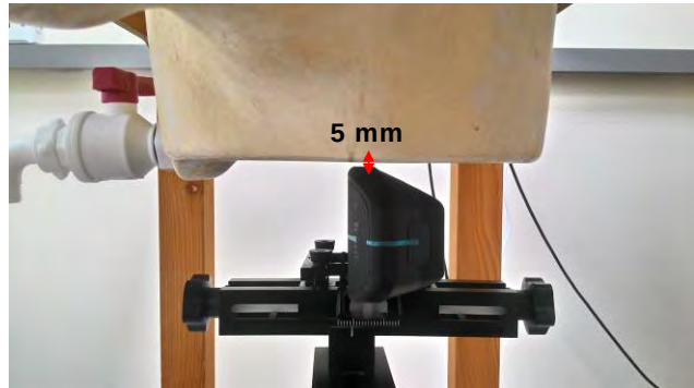
Fig.6 EUT left side to flat phantom
