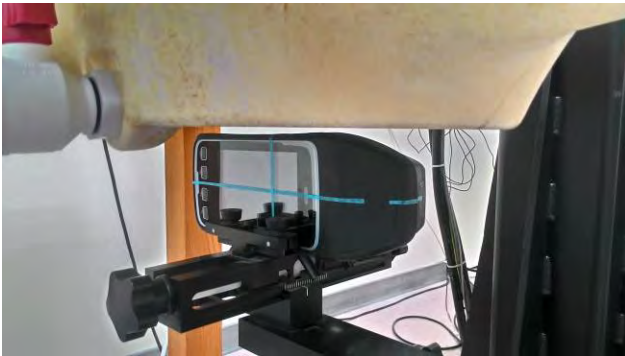
Fig.6 EUT left side to flat phantom
