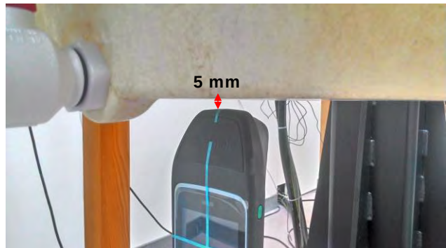
Fig.8 EUT top side to flat phantom
