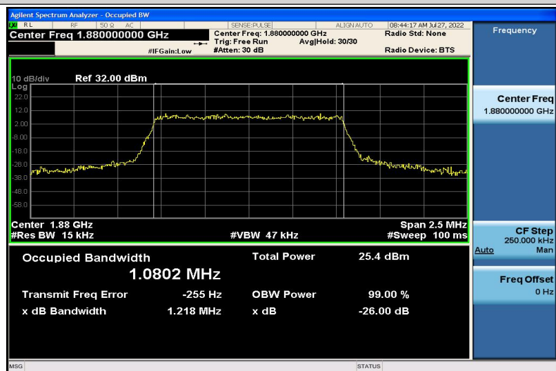
Band2-1.4MHz-16QAM-18900-6RB#0-1.0802
