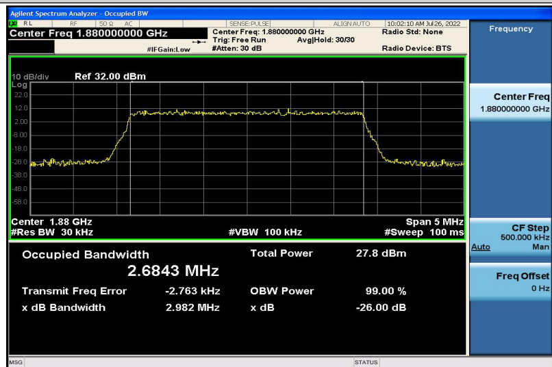
Band2-3MHz-QPSK-18900-15RB#0-2.6843
