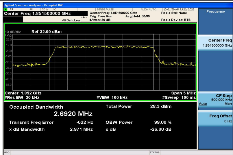
Band2-3MHz-16QAM-18615-15RB#0-2.6920
