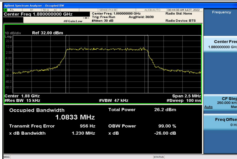
Band2-1.4MHz-QPSK-18900-6RB#0-1.0833
