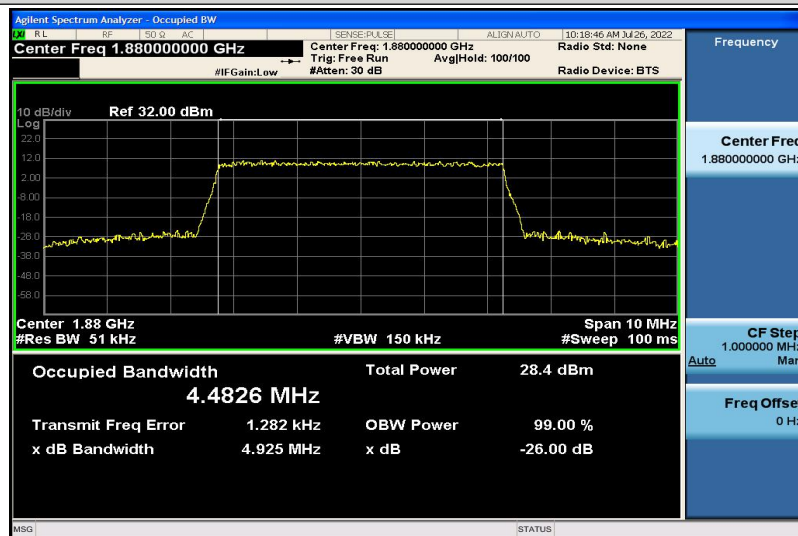
Band2-5MHz-16QAM-18900-25RB#0-4.4826
