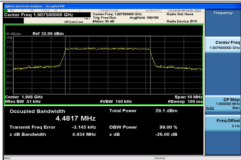
Band2-5MHz-QPSK-19175-25RB#0-4.4817
