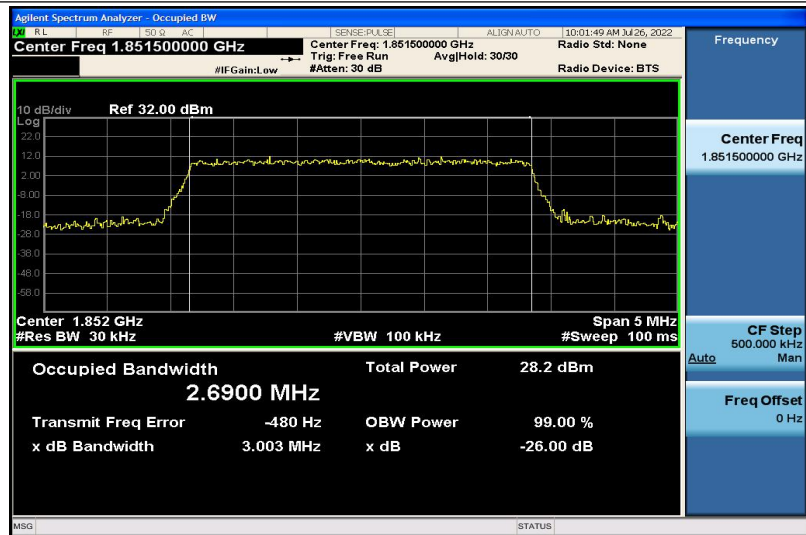
Band2-3MHz-QPSK-18615-15RB#0-2.6900
