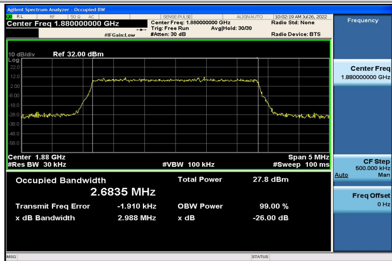
Band2-3MHz-16QAM-18900-15RB#0-2.6835
