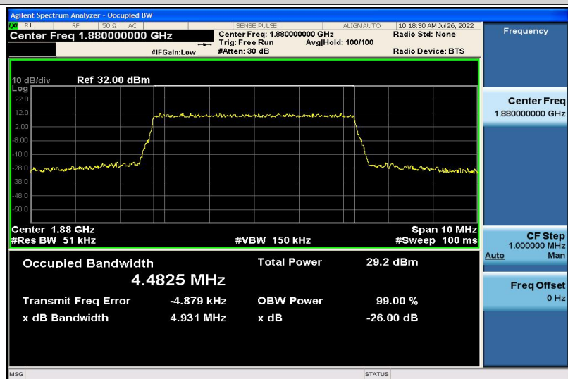
Band2-5MHz-QPSK-18900-25RB#0-4.4825
