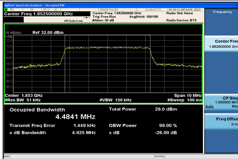
Band2-5MHz-16QAM-18625-25RB#0-4.4841
