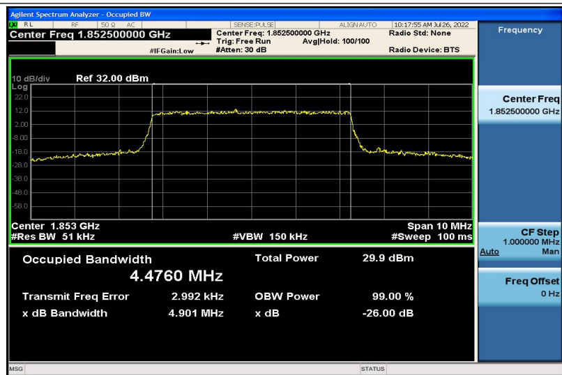
Band2-5MHz-QPSK-18625-25RB#0-4.4760
