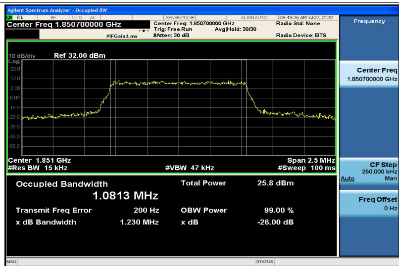
Band2-1.4MHz-16QAM-18607-6RB#0-1.0813
