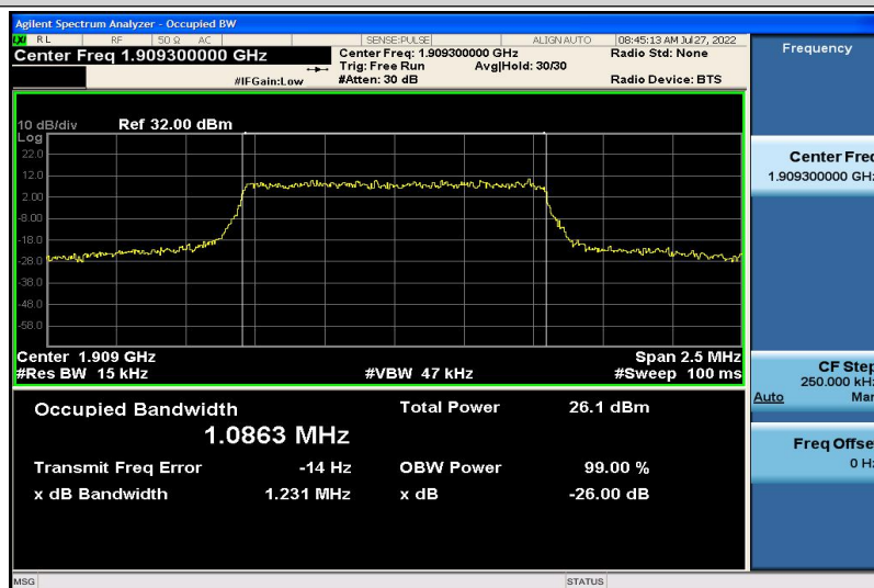
Band2-1.4MHz-QPSK-19193-6RB#0-1.0863
