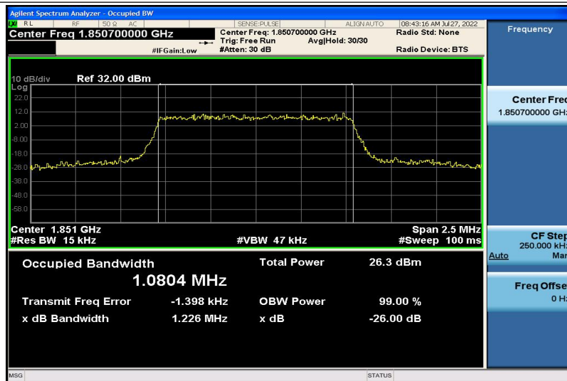
Band2-1.4MHz-QPSK-18607-6RB#0-1.0804
